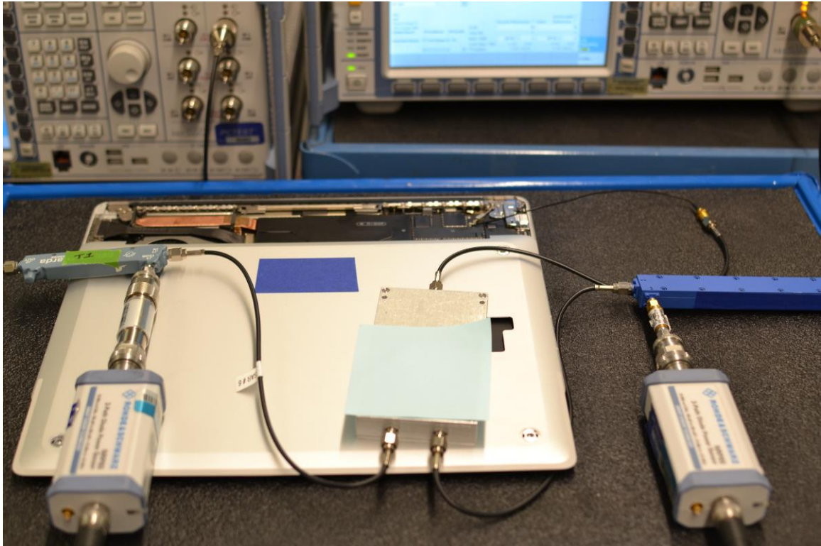
Test Setup Photo 3 – Conducted Test Setup (Figure 5-1b)
