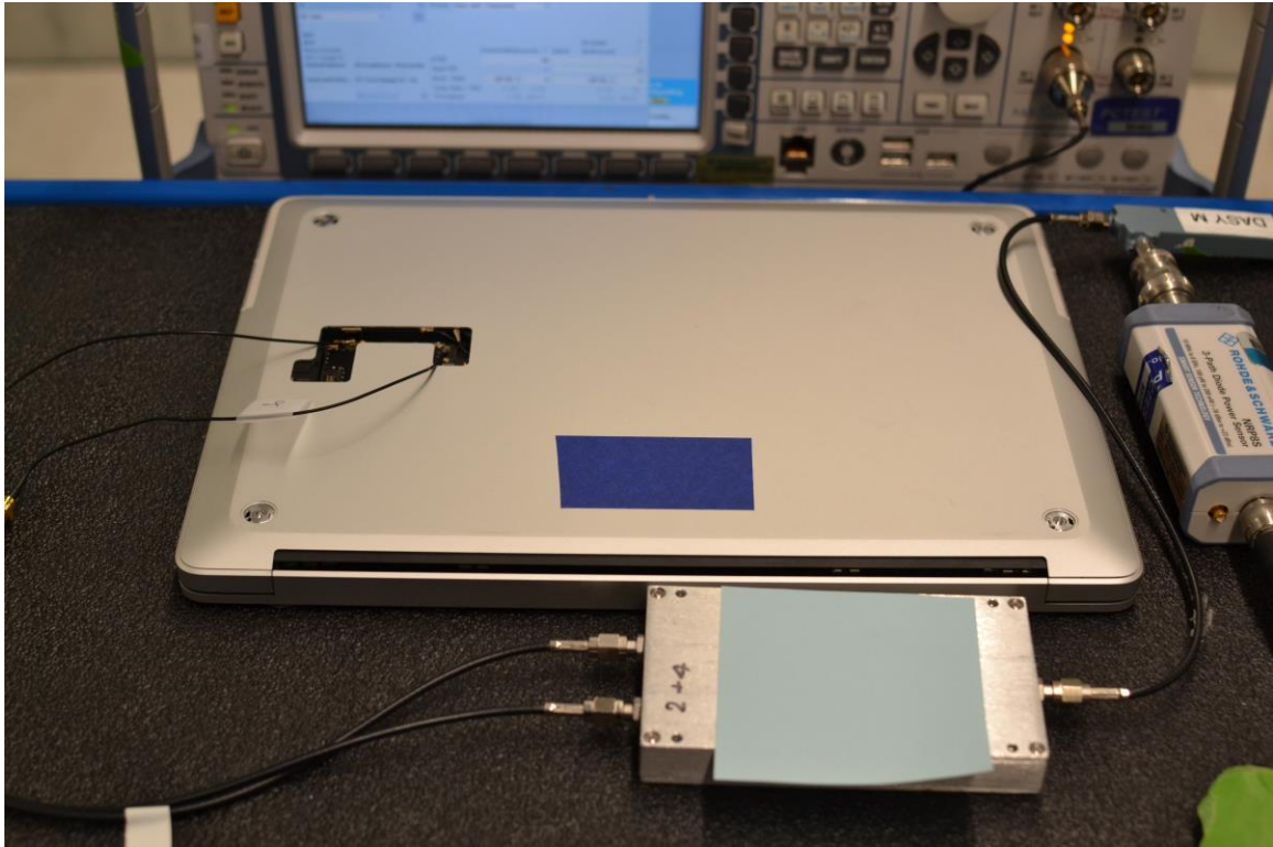
Test Setup Photo 7 – Conducted Test Setup (Figure 6-1b)
