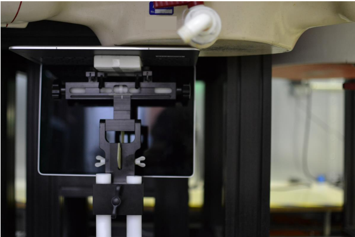
Test Setup Photo 12 – Radiated SAR, Bottom Edge, Antenna 1 at 0mm
