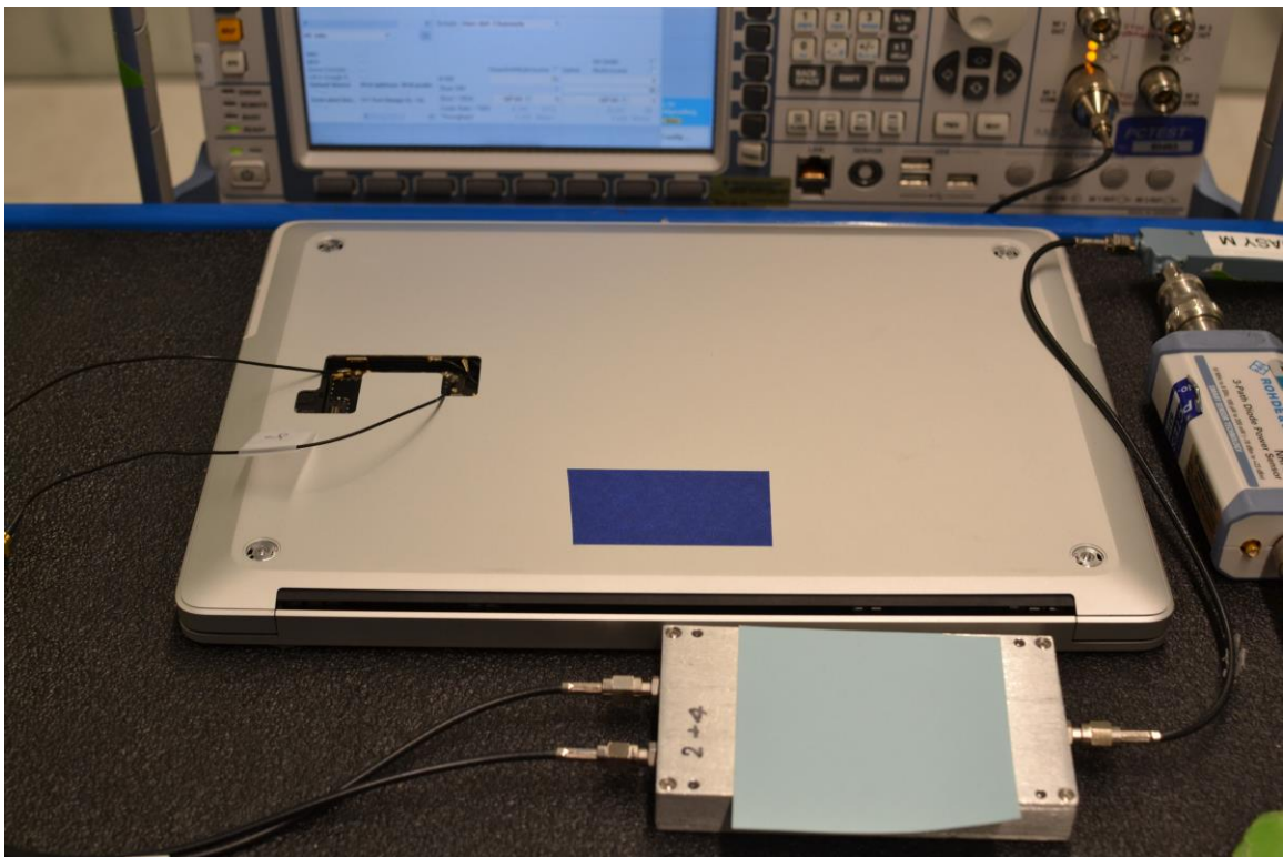
Test Setup Photo 6 – Conducted Test Setup (Figure 6-1b)
