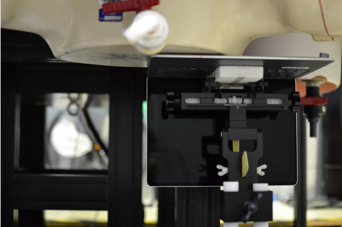
Test Setup Photo 11 – Radiated SAR, Bottom Edge, Antenna 5 and 6 at 0mm
