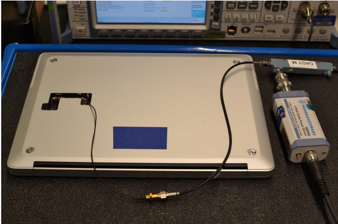
Test Setup Photo 3 – Conducted Test Setup (Figure 6-1a)
