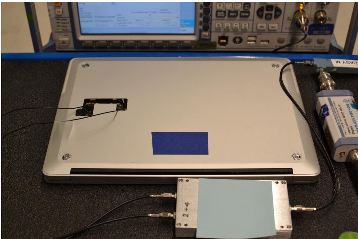
Test Setup Photo 8 – Conducted Test Setup (Figure 6-1b)
