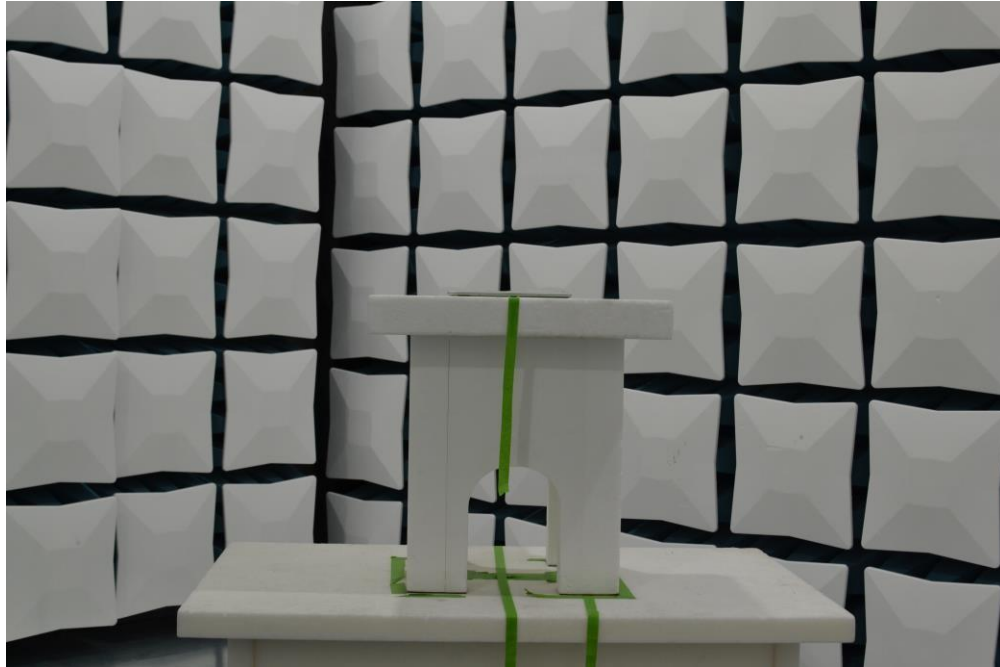
Figure 3. Test Setup – X Position – 1GHz-40GHz – Closed
