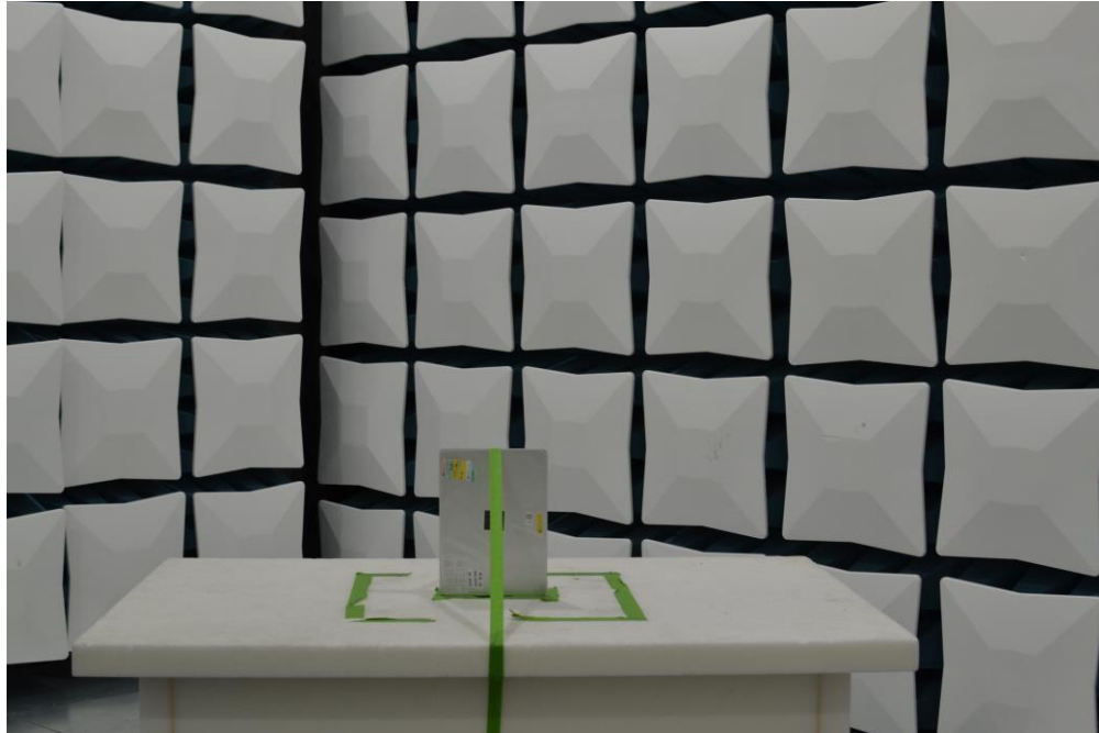
Figure 7. Test Setup – Y Position – 30MHz-1GHz – Closed
