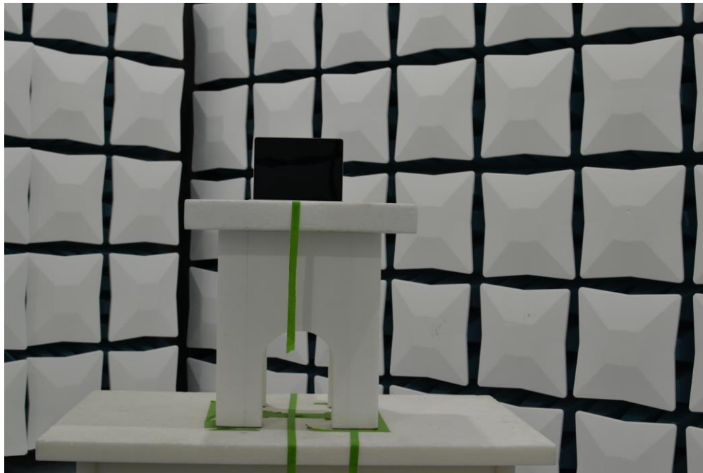
Figure 15. Test Setup – X Position – 1GHz-40GHz – Half Open
