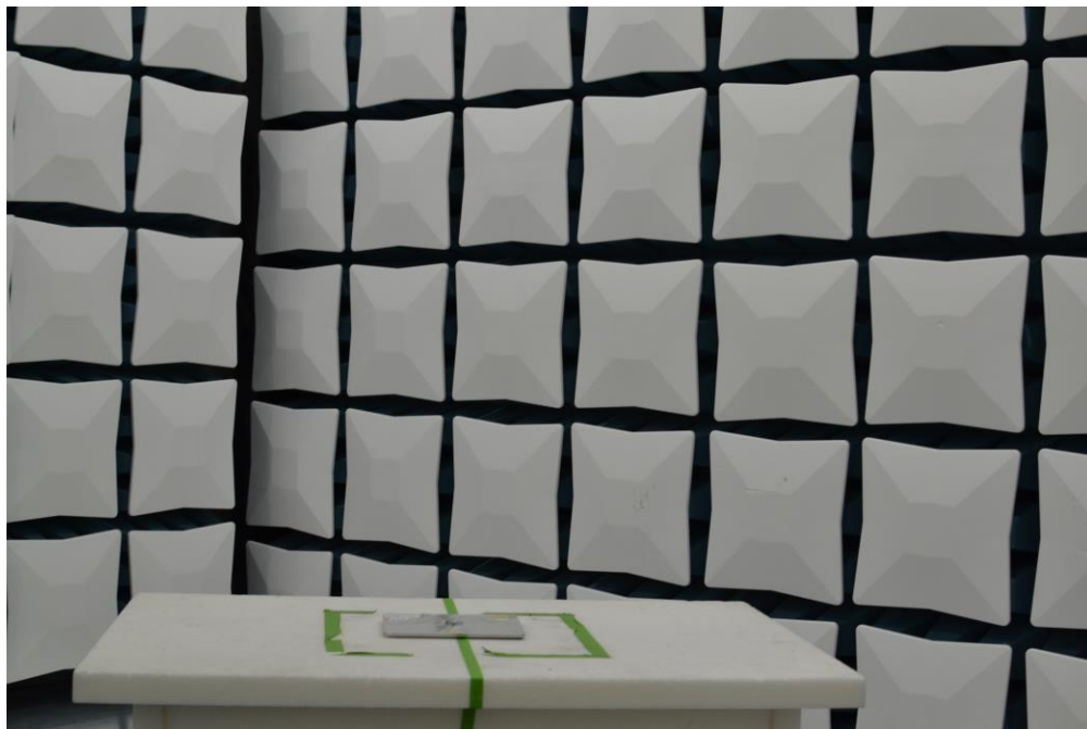
Figure 6. Test Setup – X Position – 30MHz-1GHz – Closed
