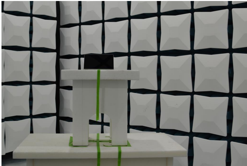
Figure 9. Test Setup – X Position – 1GHz-40GHz – Open
