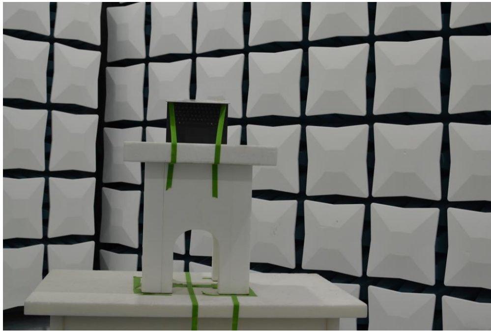
Figure 17. Test Setup – Z Position – 1GHz-40GHz – Half Open
