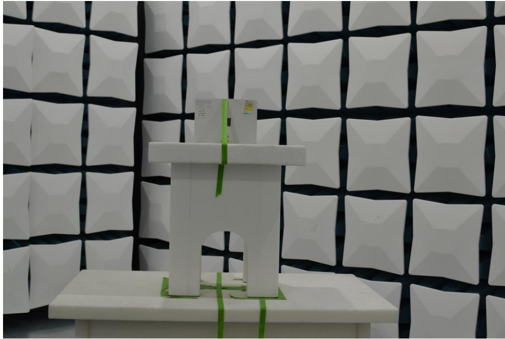
Figure 5. Test Setup – Z Position – 1GHz-40GHz – Closed
