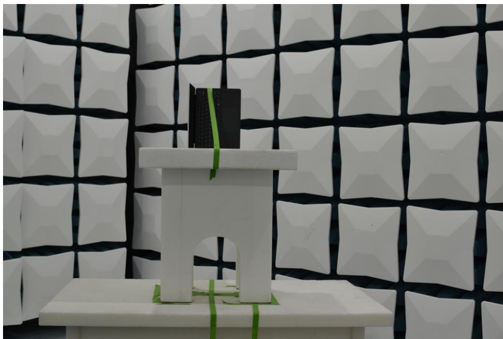
Figure 16. Test Setup – Y Position – 1GHz-40GHz – Half Open
