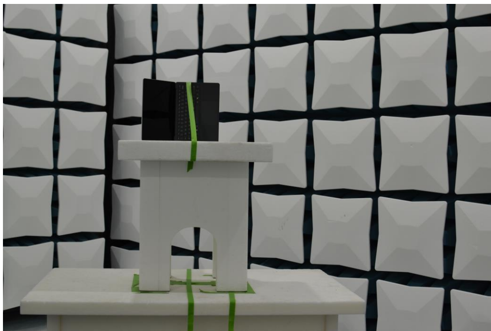
Figure 10. Test Setup – Y Position – 1GHz-40GHz – Open
