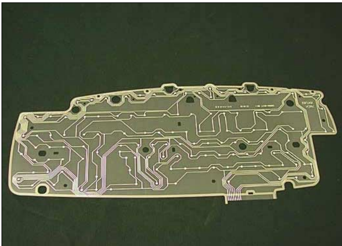
Keyboard - Top Membrane Bottom Side
