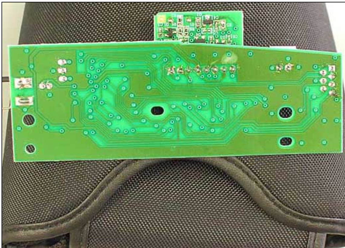
Keyboard - Main and RF Bottom Side
