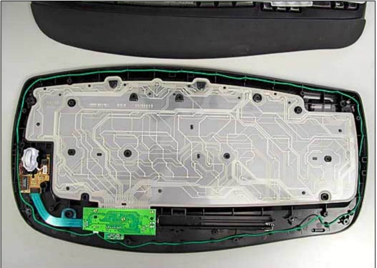
Keyboard – Top Cover Off 2
