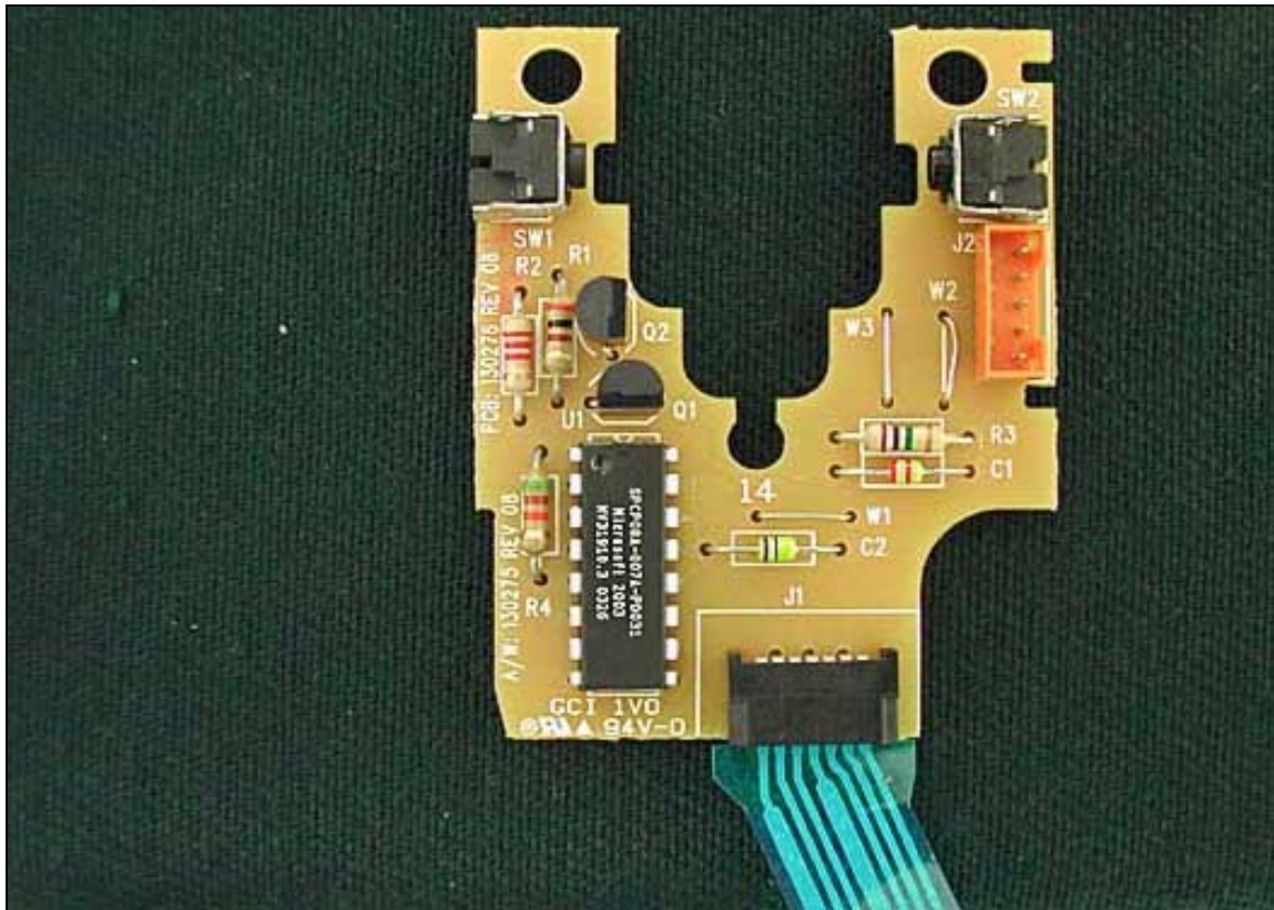
Keyboard - Scroll Wheel PCB Top Side
