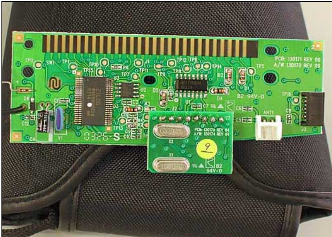
Keyboard - Main And RF Top Side
