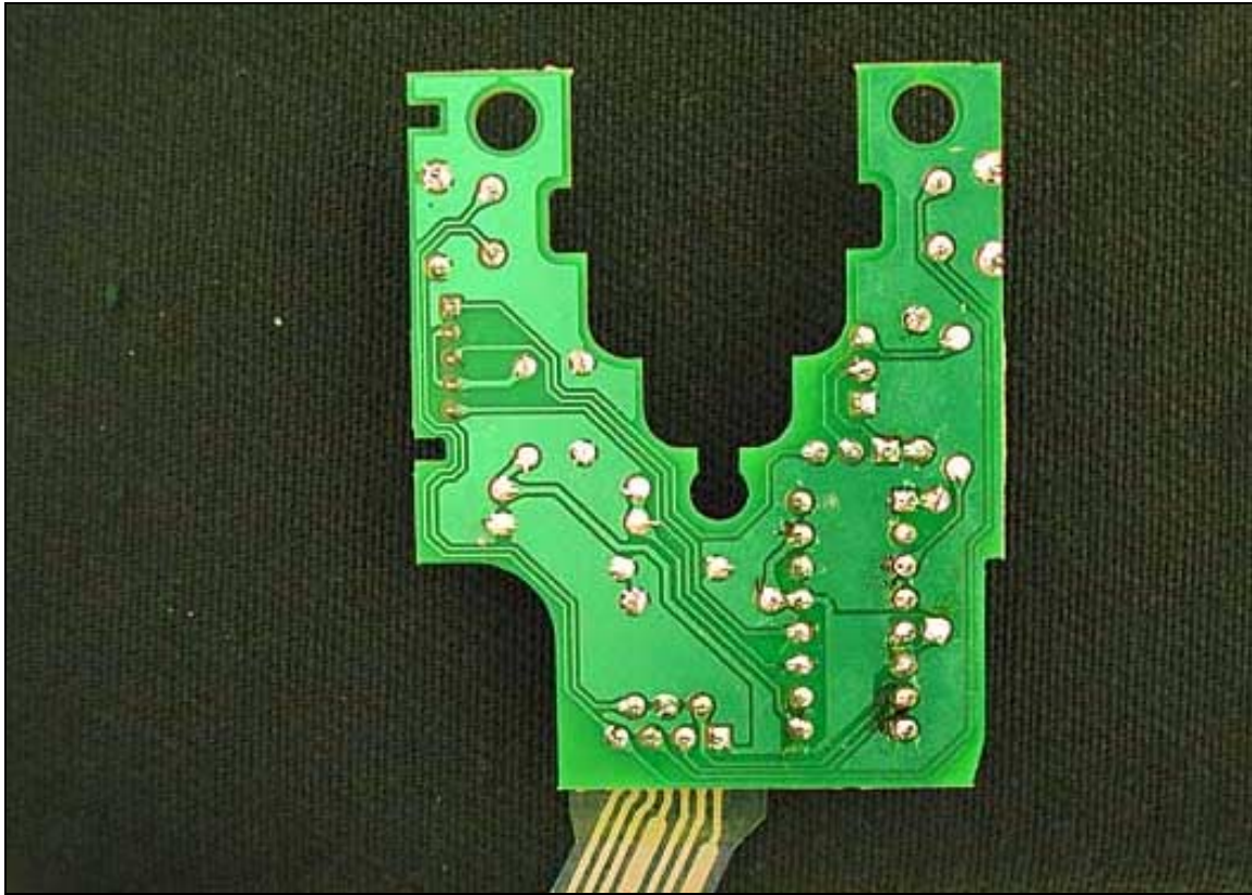
Keyboard - Scroll Wheel PCB Bottom Side
