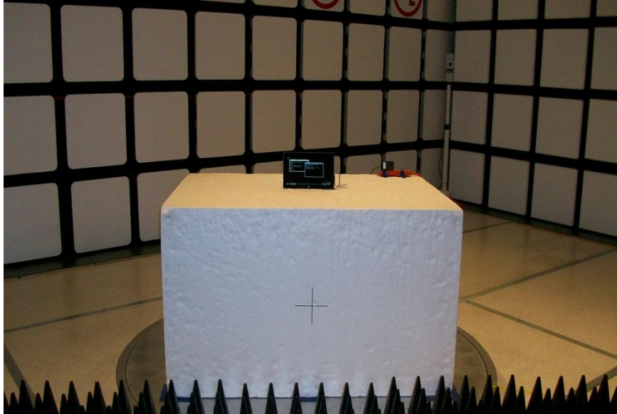
RADIATED FRONT PHOTO (ABOVE 1 GHz)
