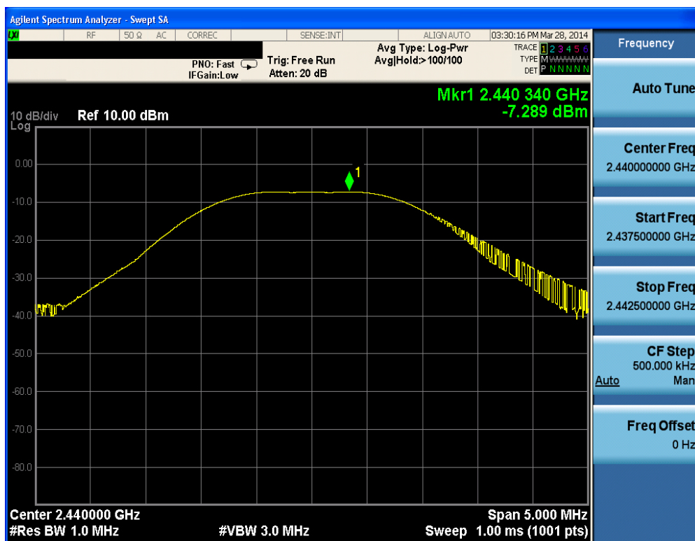
Plot 9-7. Peak Power (Ch. 19)
