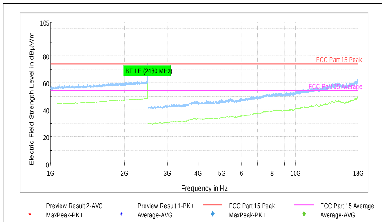
Plot 9-22. Radiated Spurious Emissions (Ch. 39) (1-18GHz)
