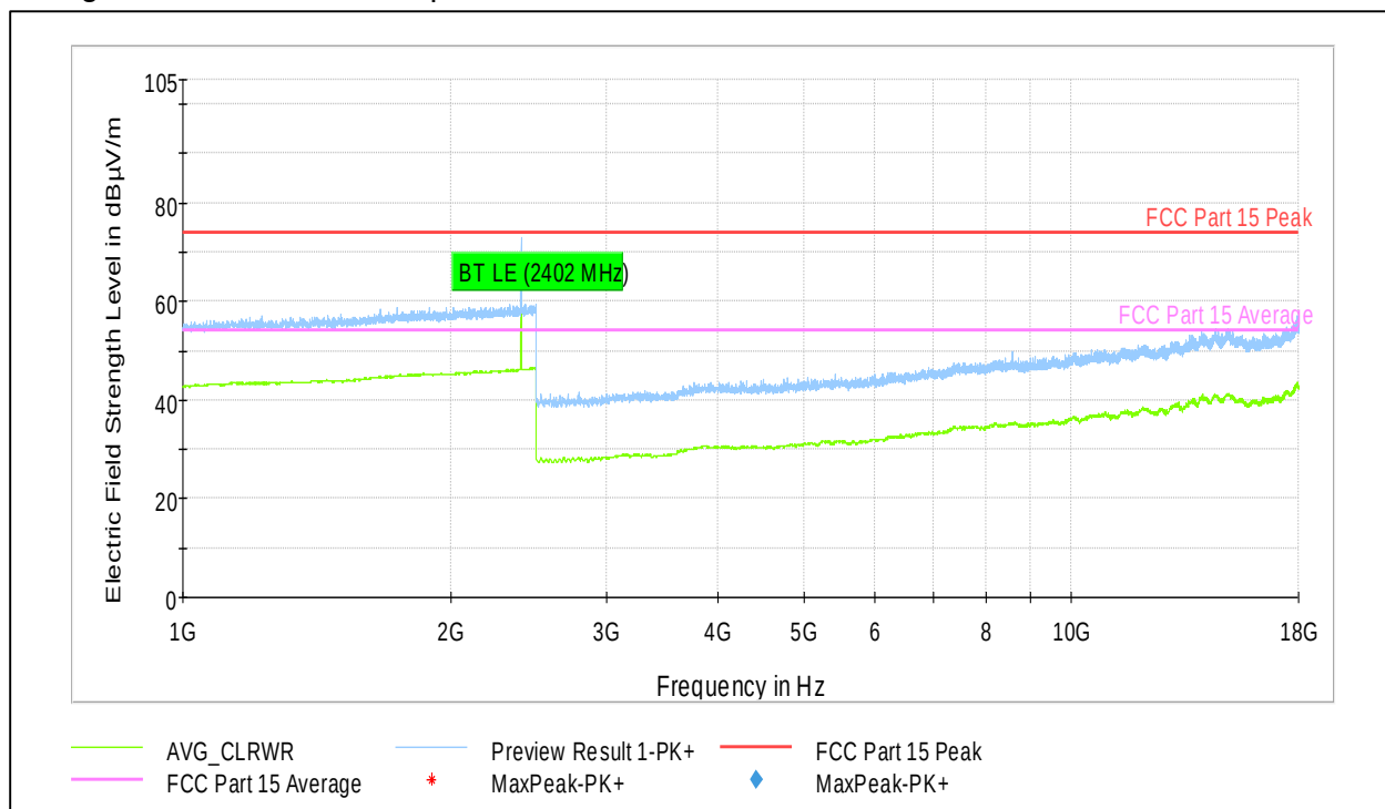
Plot 9-20. Radiated Spurious Emissions (Ch. 0) (1-18GHz)
