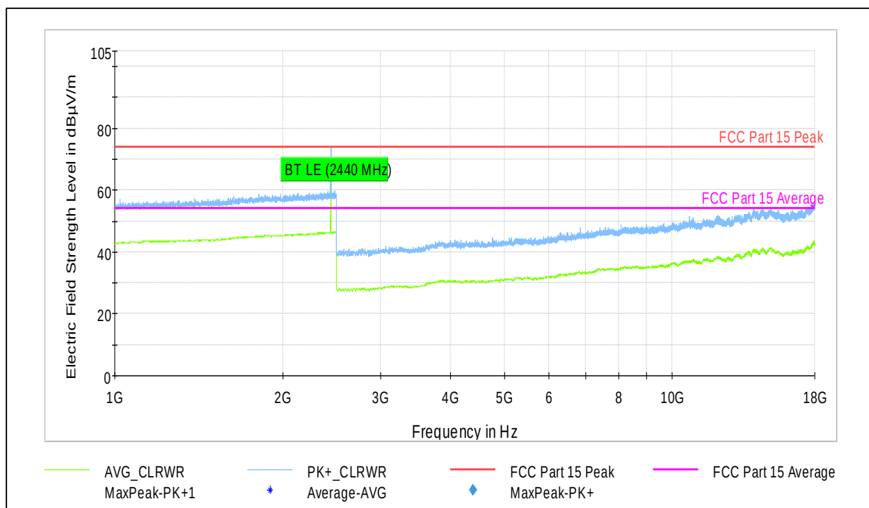
Plot 9-21. Radiated Spurious Emissions (Ch. 19) (1-18GHz)
