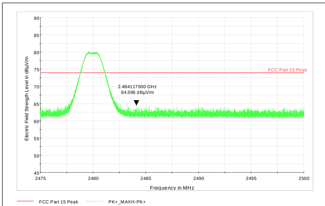
Plot 9-26. Radiated Restricted Band Edge (Ch. 39) Peak
