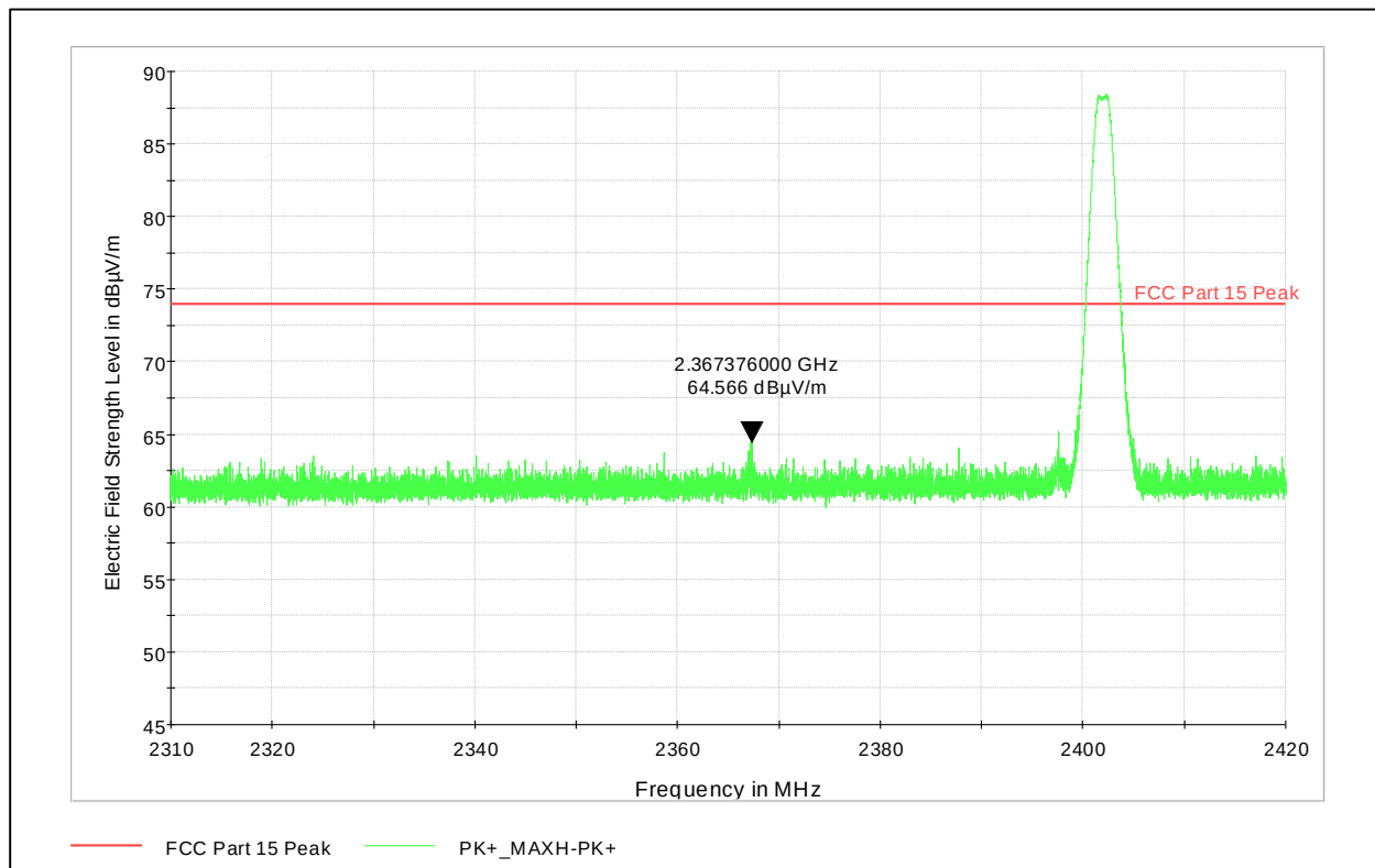
Plot 9-24. Radiated Restricted Band Edge (Ch. 0) Peak
