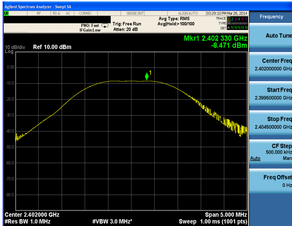
Plot 9-4. Average Power (Ch. 0)
