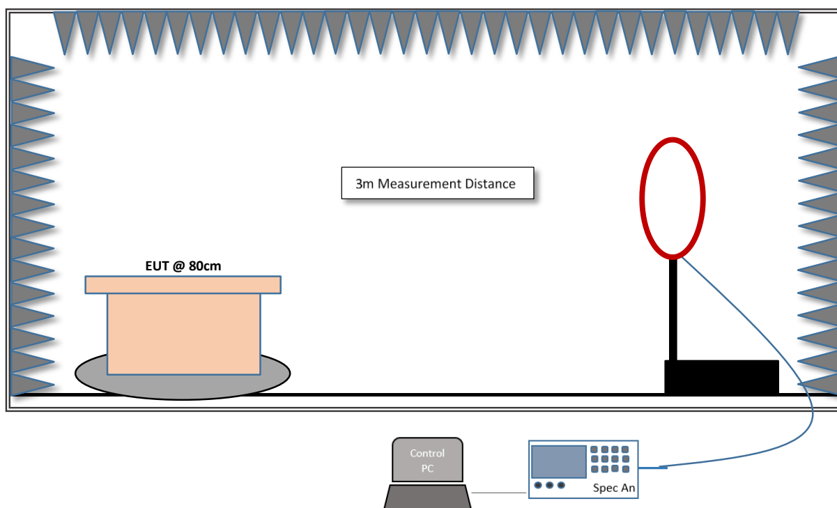
Fig.2. Test Setup for Radiated measurements <30 MHz
