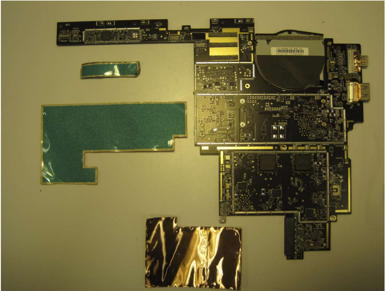
Motherboard Top Side. Shield cans removed.
