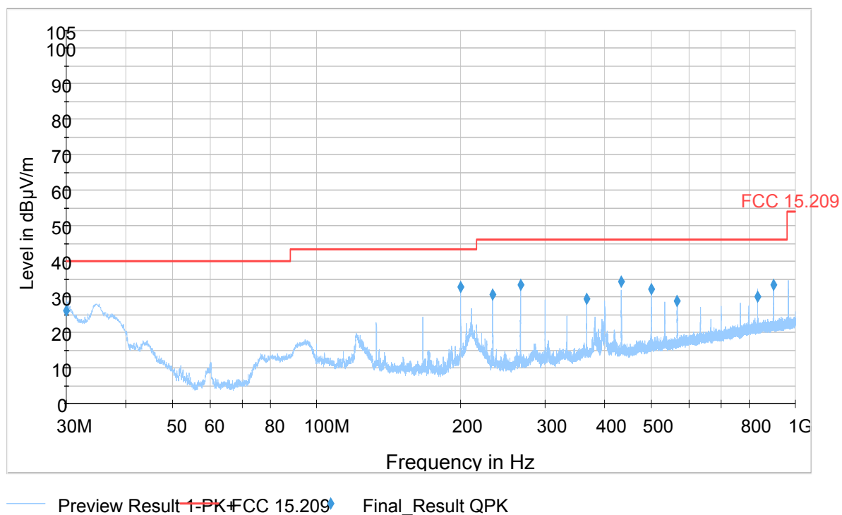
Figure 9-9 Radiated Spurious Emissions (2440 MHz) (30MHz - 1GHz)
