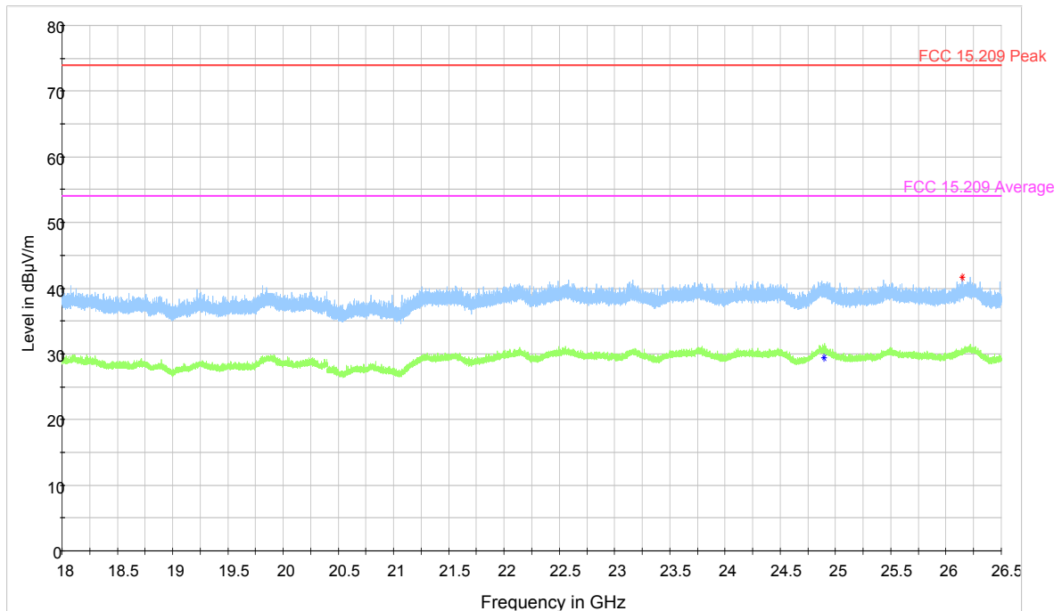
Plot 9-25. Radiated Spurious Emissions (Ch. 0) (18 – 26.5 GHz)
