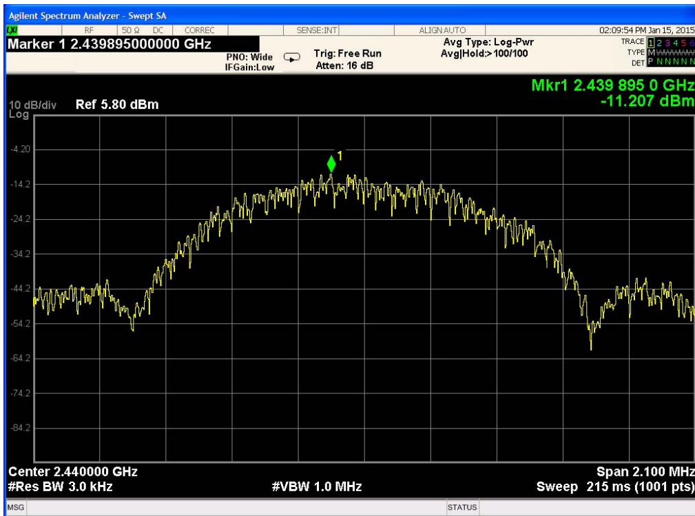
Plot 9-11. Power Spectral Density (Ch. 19)
