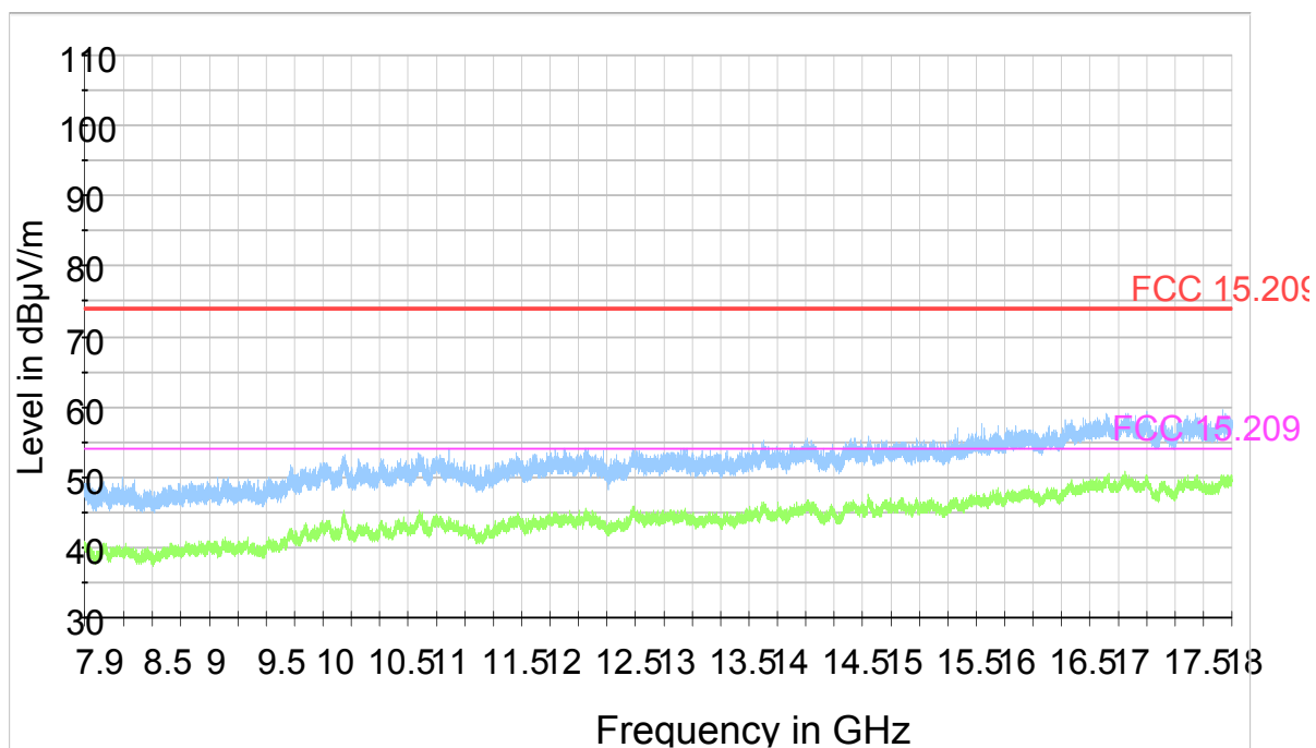
Plot 9-24. Radiated Spurious Emissions (Ch. 39) (7.9-18 GHz)
