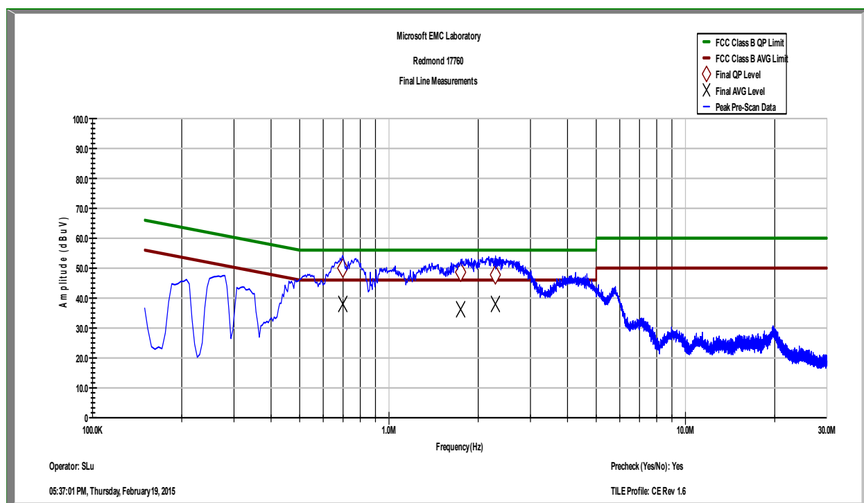
Plot 9-32. AC Line Conducted Emissions- Line (150 kHz- 30 MHz)
