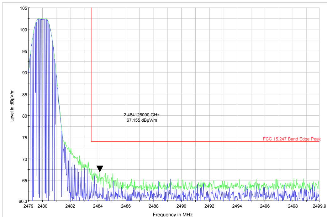
Plot 9-30. Radiated Restricted Band Edge (Ch. 39) Peak
