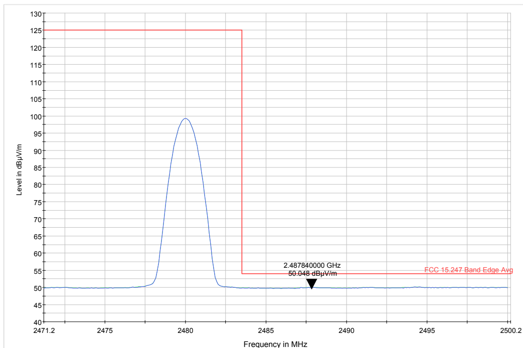
Plot 9-31. Radiated Restricted Band Edge (Ch. 39) Average
