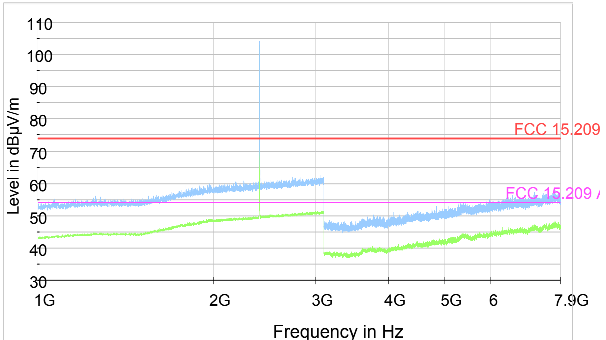
Plot 9-19. Radiated Spurious Emissions (Ch. 0) (1-7.9GHz)
