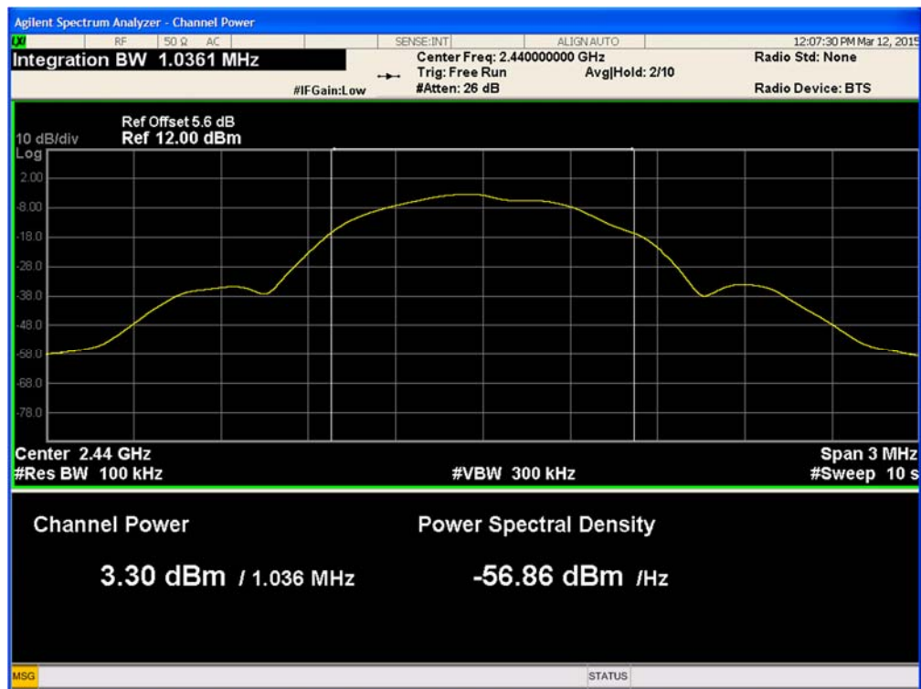
Plot 9-6. Average Power (Ch. 19)
