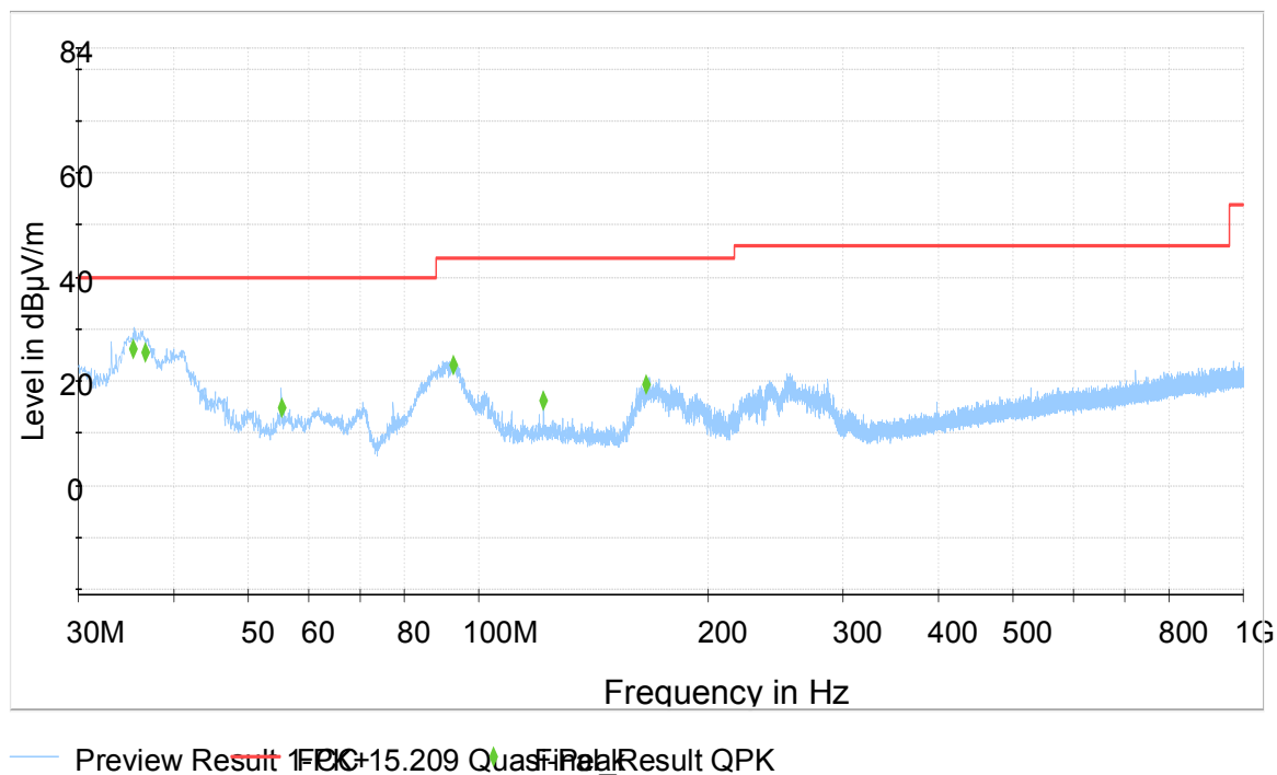
Plot 9-18. Radiated Spurious Emissions (Ch. 39) (30MHz - 1GHz)
