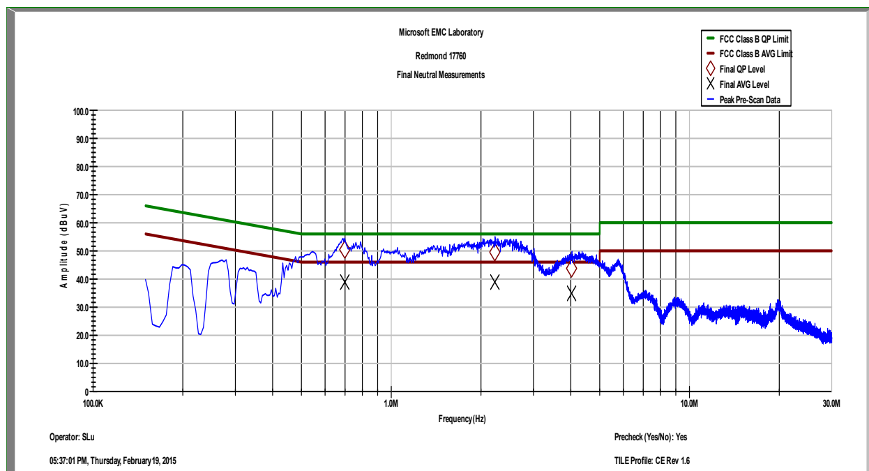
Plot 9-33. AC Line Conducted Emissions- Neutral (150 kHz- 30 MHz)
