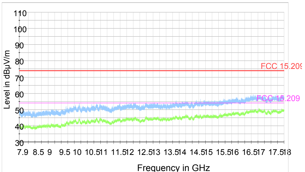
Plot 9-22. Radiated Spurious Emissions (Ch. 0) (7.9-18 GHz)
