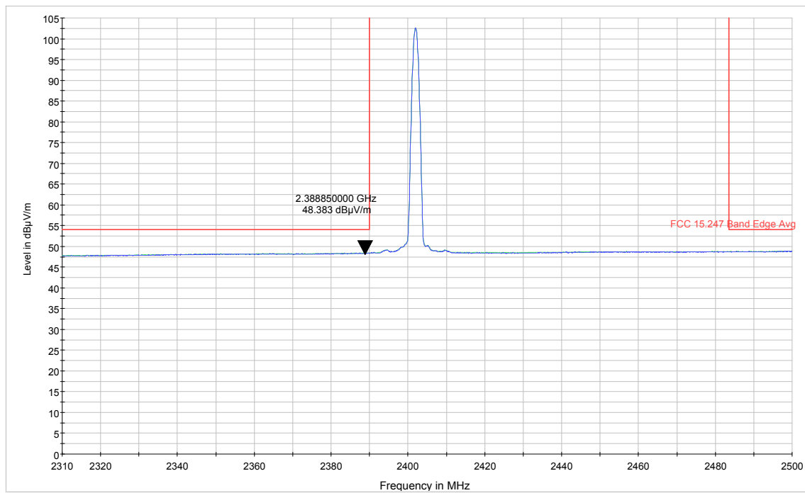
Plot 9-29. Radiated Restricted Band Edge (Ch. 0) Average
