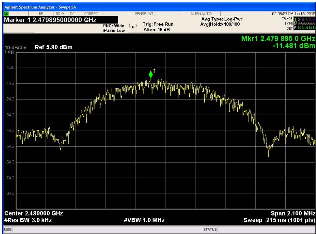
Plot 9-12. Power Spectral Density (Ch. 39)
