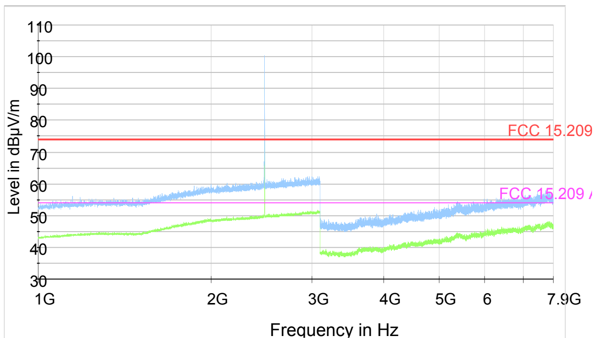
Plot 9-21. Radiated Spurious Emissions (Ch. 39) (1-7.9GHz)
