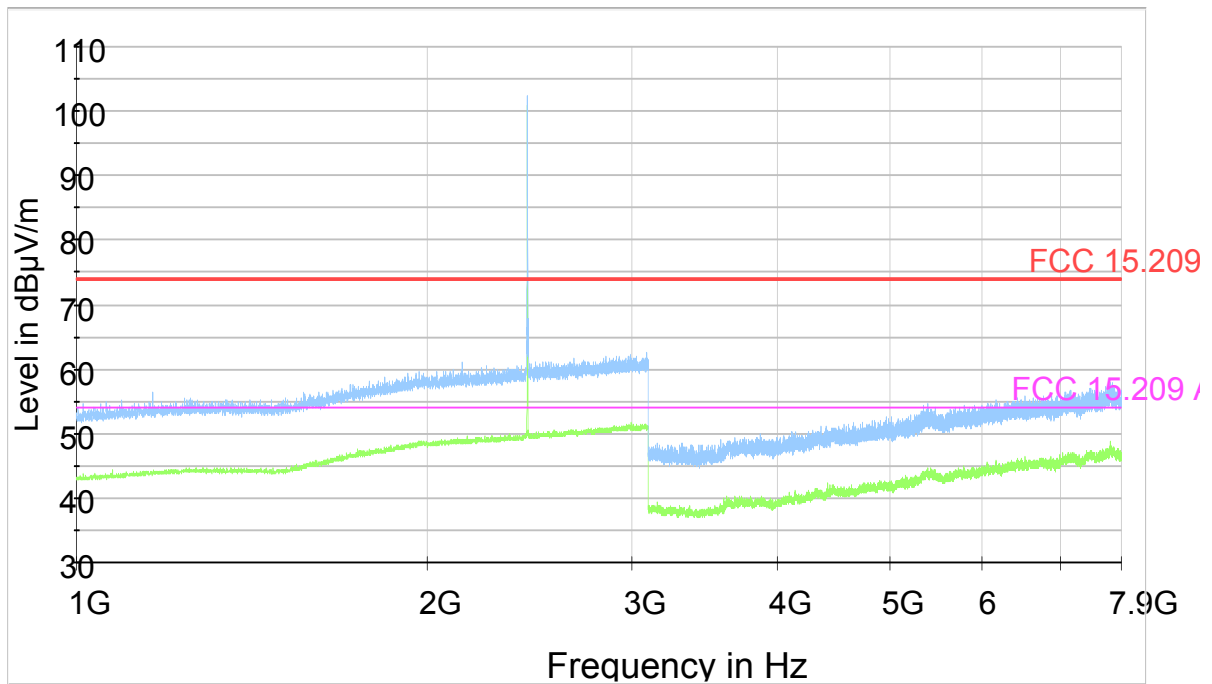
Plot 9-20. Radiated Spurious Emissions (Ch. 19) (1-7.9GHz)
