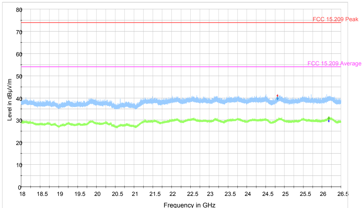
Plot 9-26. Radiated Spurious Emissions (Ch. 19) (18 – 26.5 GHz)
