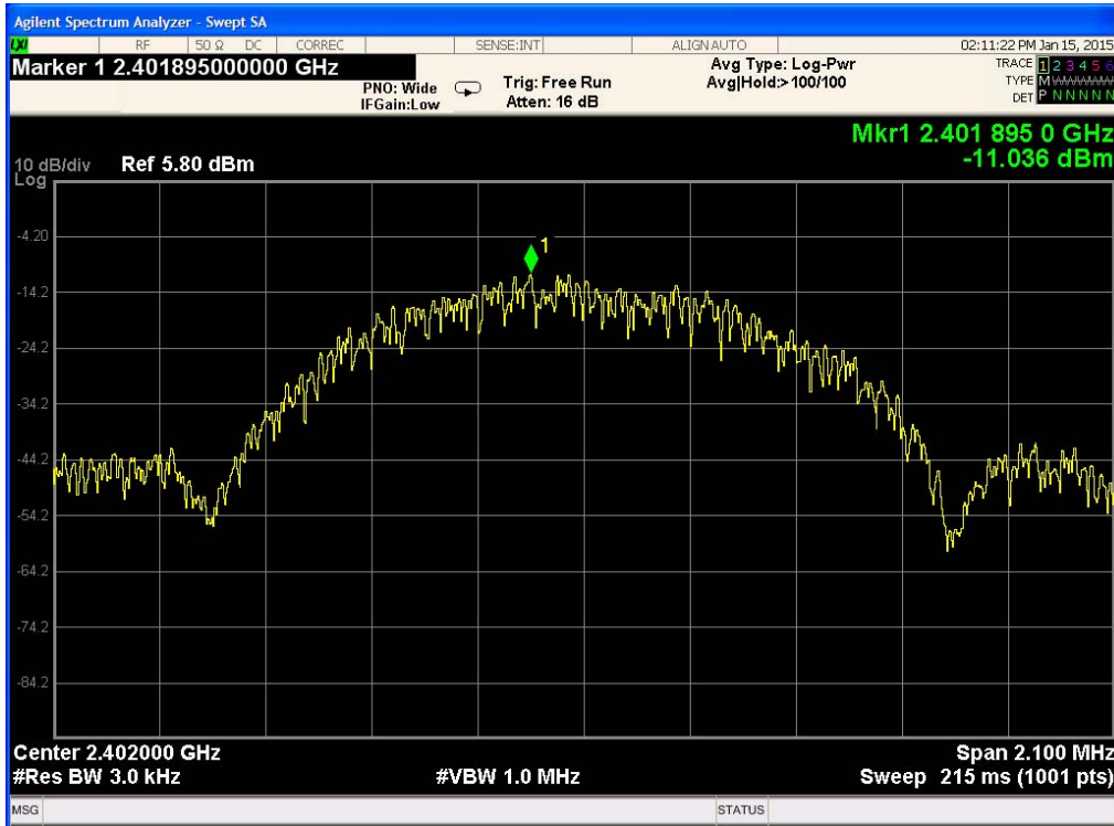
Plot 9-10. Power Spectral Density (Ch. 0)
