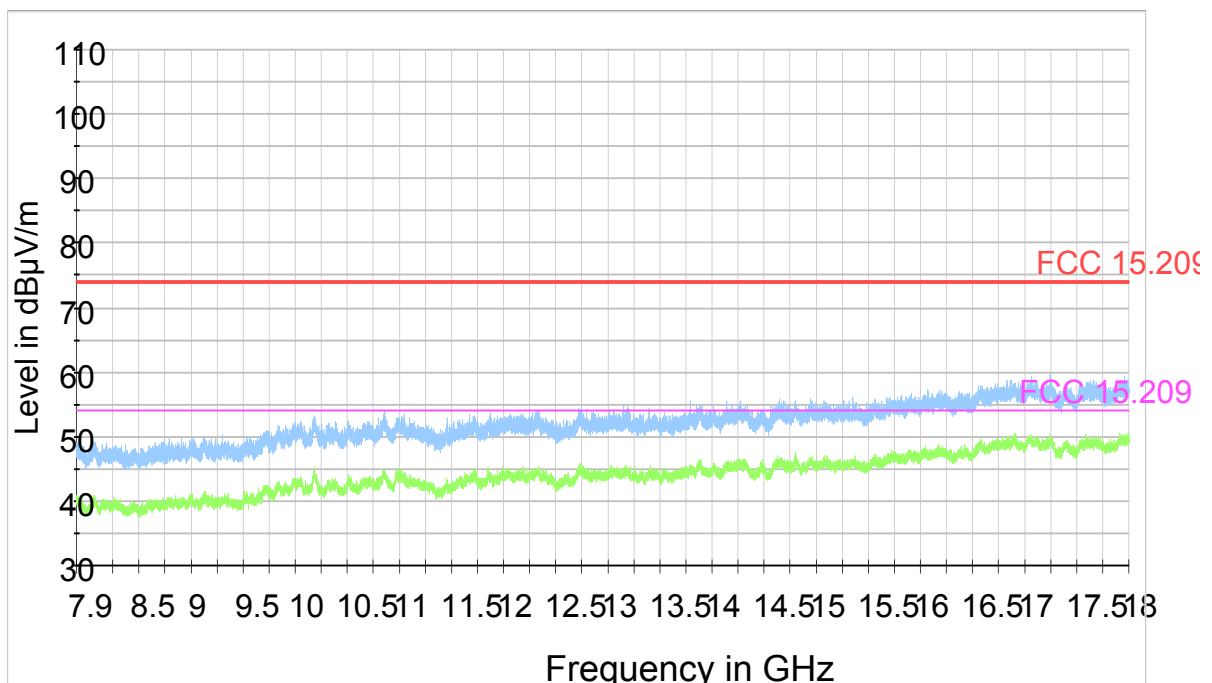
Plot 9-23. Radiated Spurious Emissions (Ch. 19) (7.9-18 GHz)
