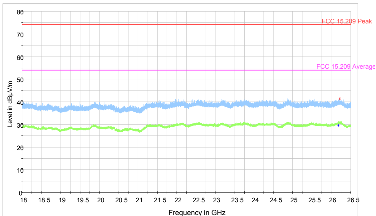
Plot 9-27. Radiated Spurious Emissions (Ch. 39) (18 – 26.5 GHz)
