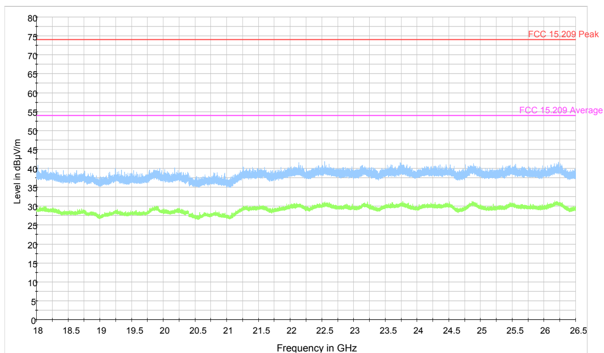
Plot 9-14. Radiated Spurious Emissions (Ch. 78) (18 - 26GHz)
