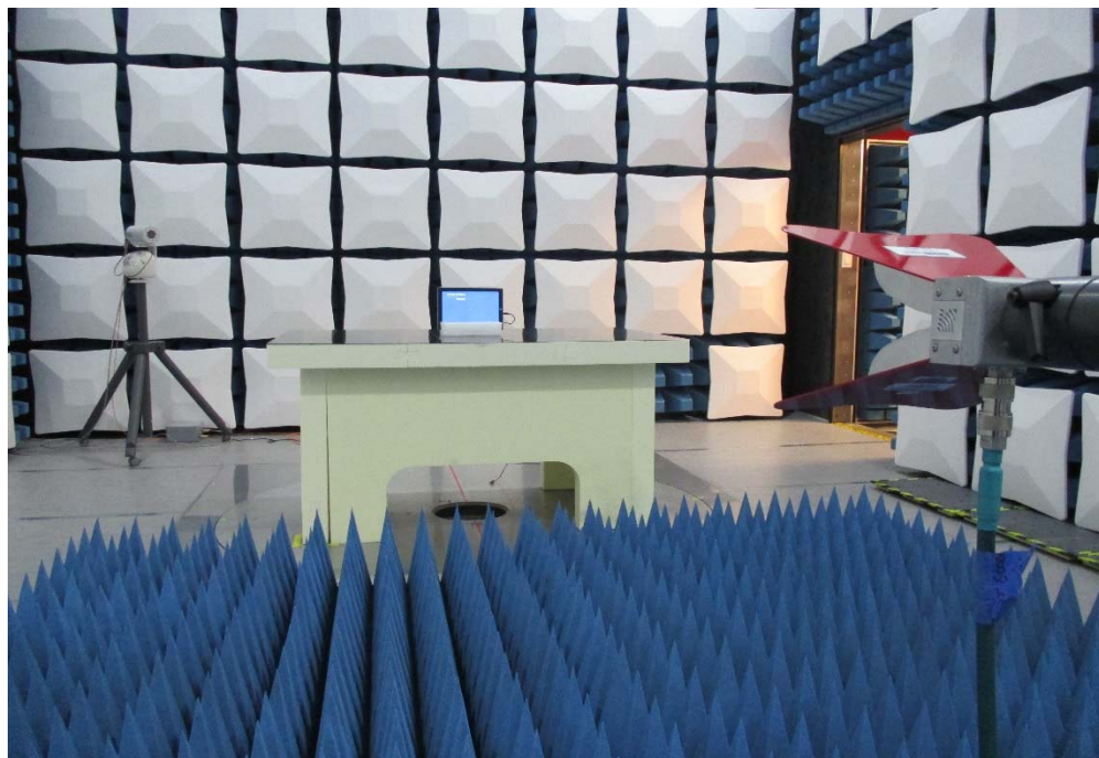
Fig.5 Radiated Spurious Emissions Test Setup (1-18 GHz)
