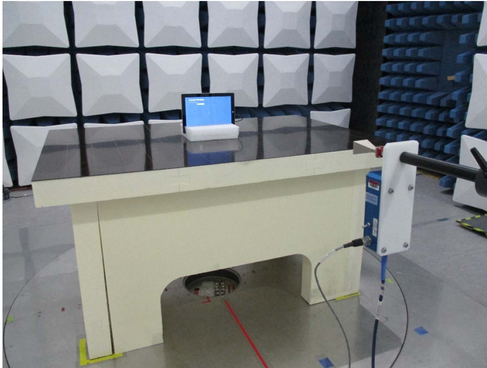
Fig.6 Radiated Spurious Emissions (1-26.5GHz)
