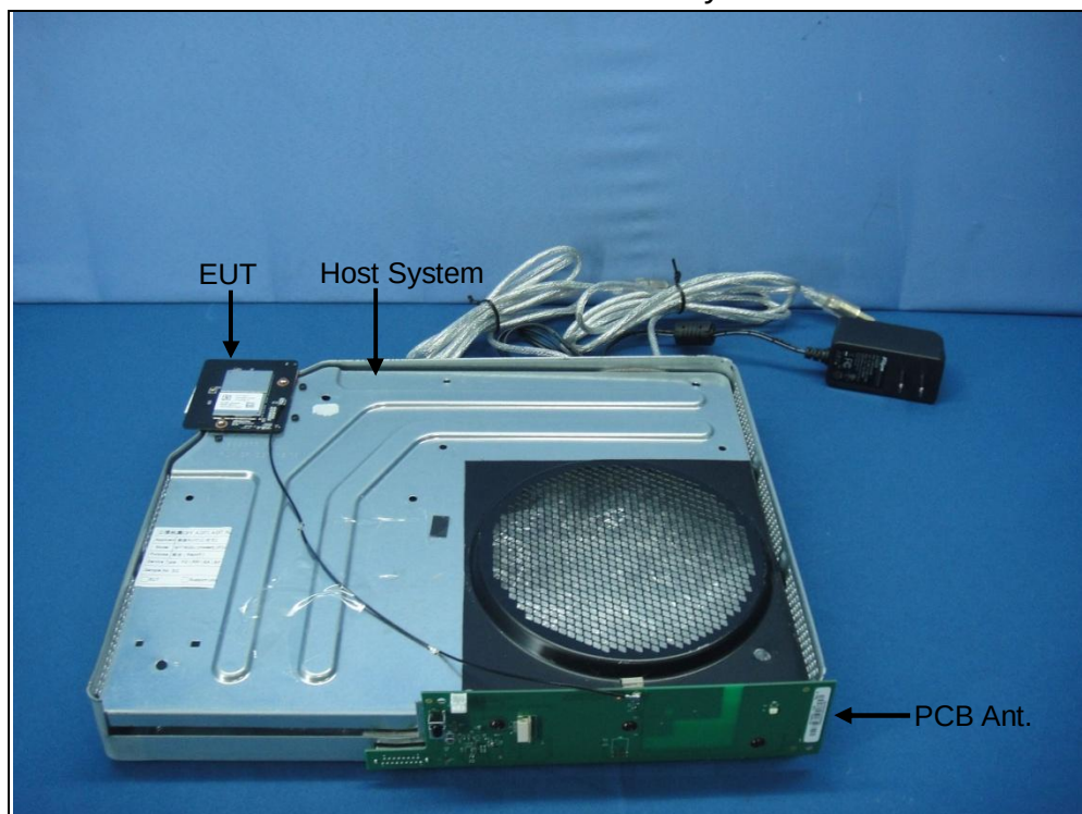
EUT + PCB Ant. + Host System
