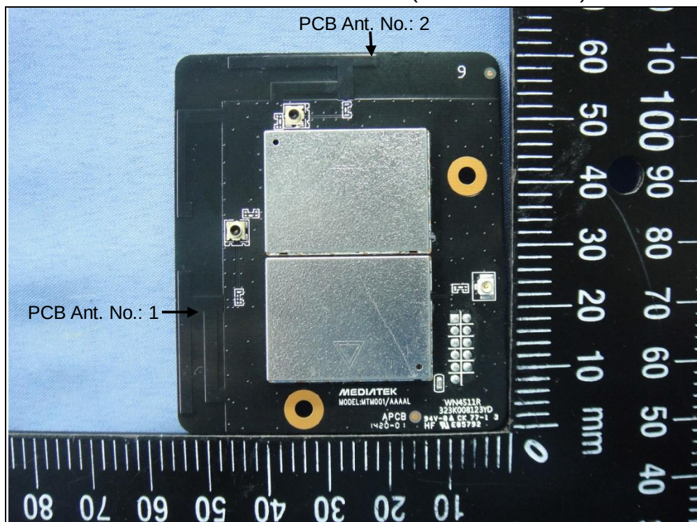
Network Radio Ant. No.: 1~2 (Brand: Microsoft)
