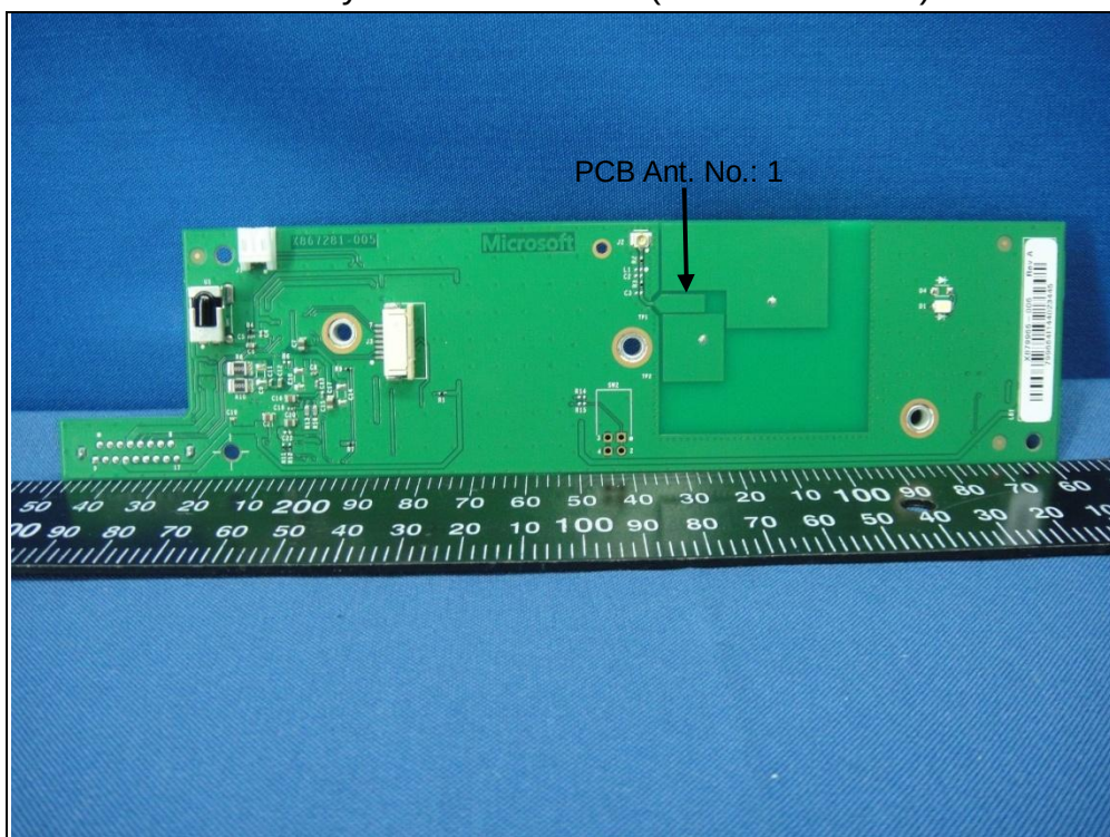
Accessory Radio Ant. No.: 1 (Brand: Microsoft)
