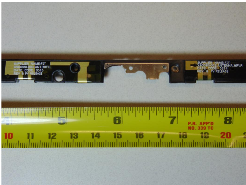
Figure 12 Wifi Antennas (Main and Aux)
