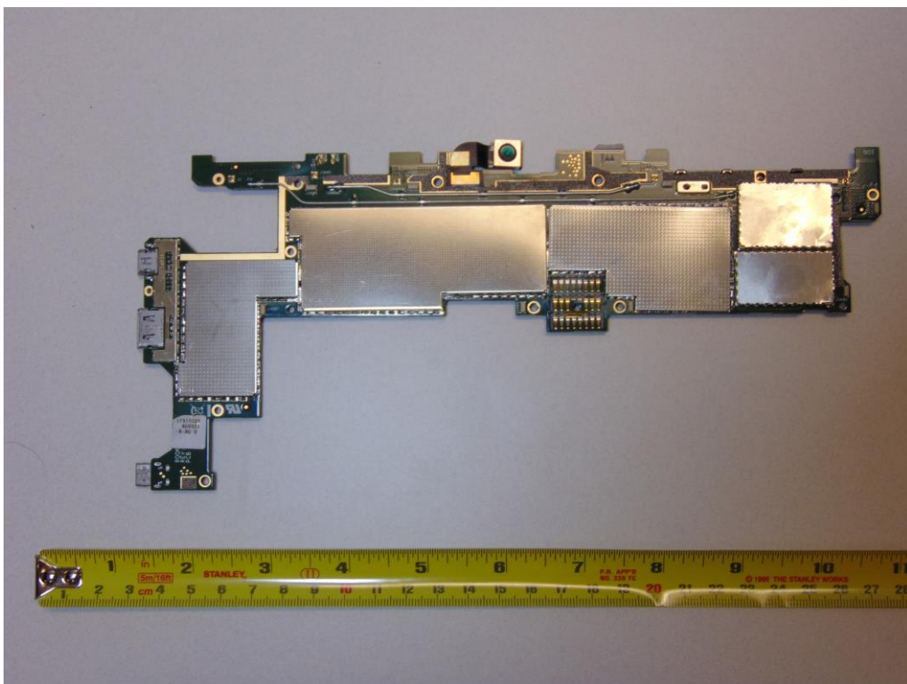
Figure 6 Motherboard (back)
