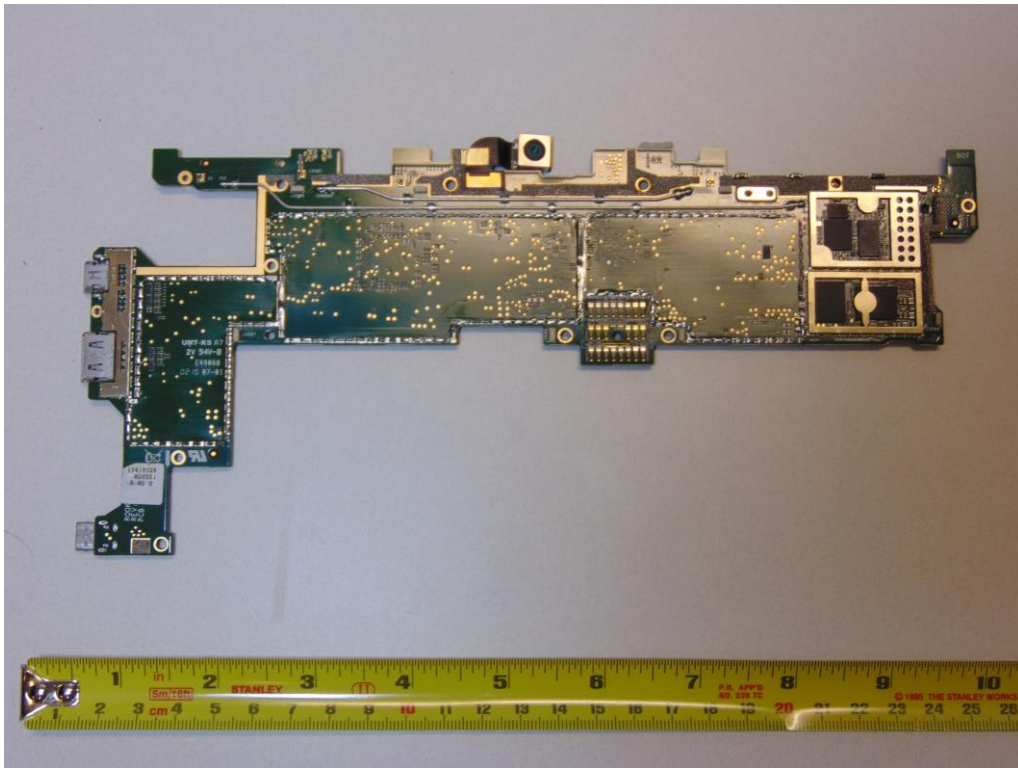
Figure 7 Motherboard (back) with shield cans removed
