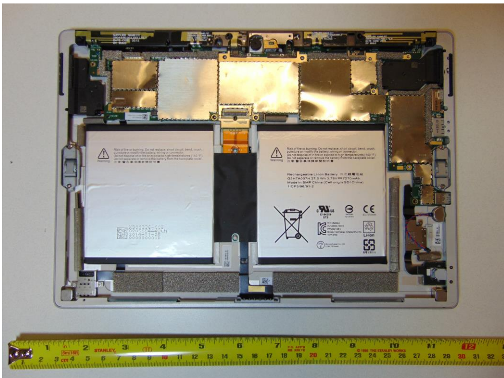
Figure 2 Antenna/Motherboard/Battery
