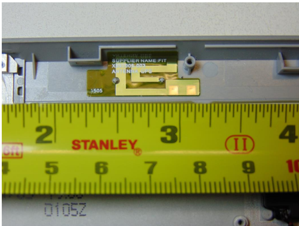
Figure 13 GPS (Receive) Antenna
