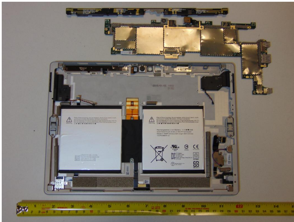
Figure 3 Antenna, motherboard, battery removed
