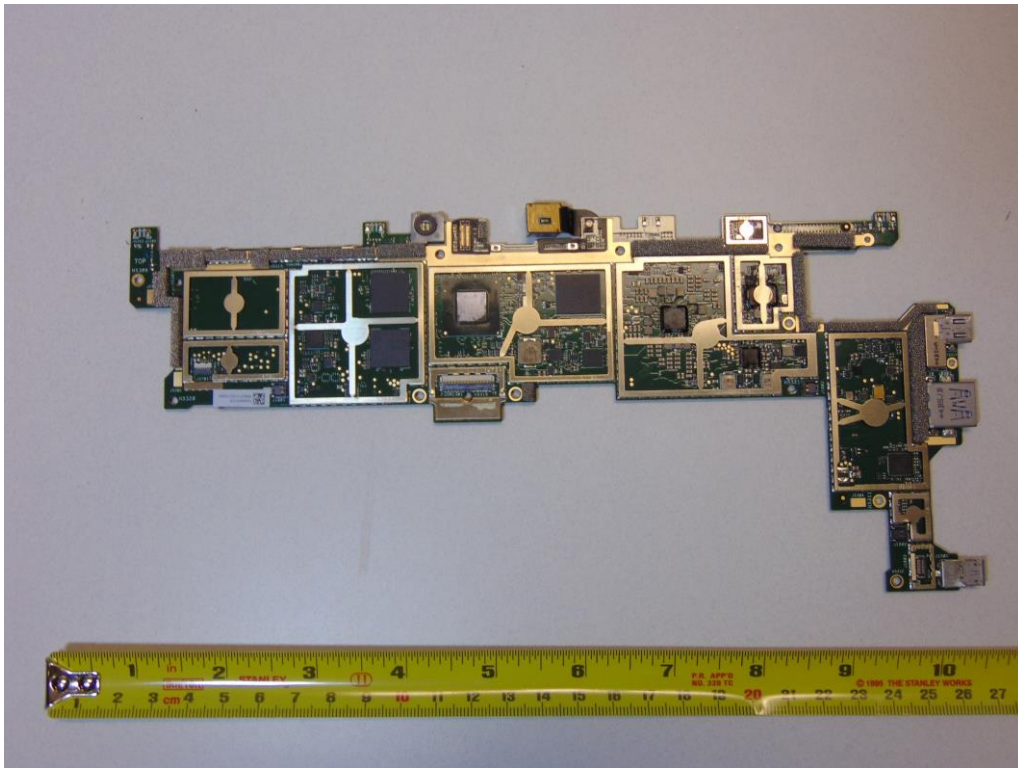
Figure 5 Motherboard (front) with shield cans removed
