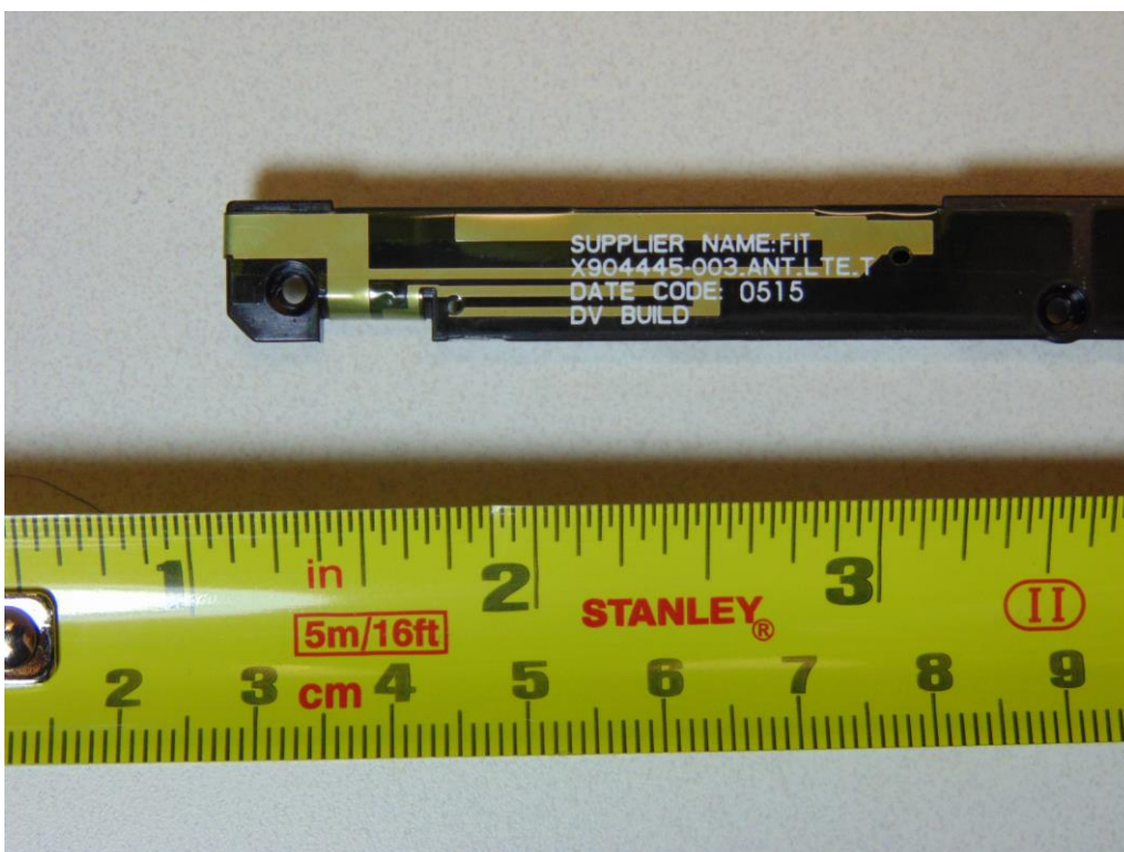
Figure 10 Cellular (Main) Antenna
