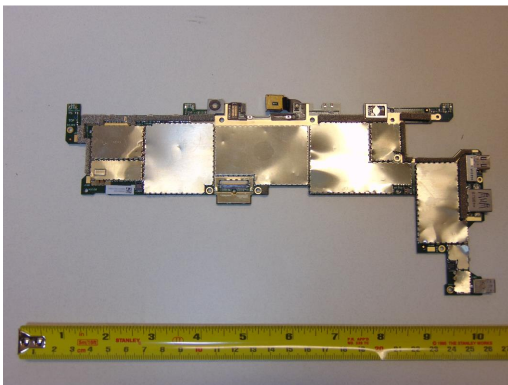
Figure 4 Motherboard (front)
