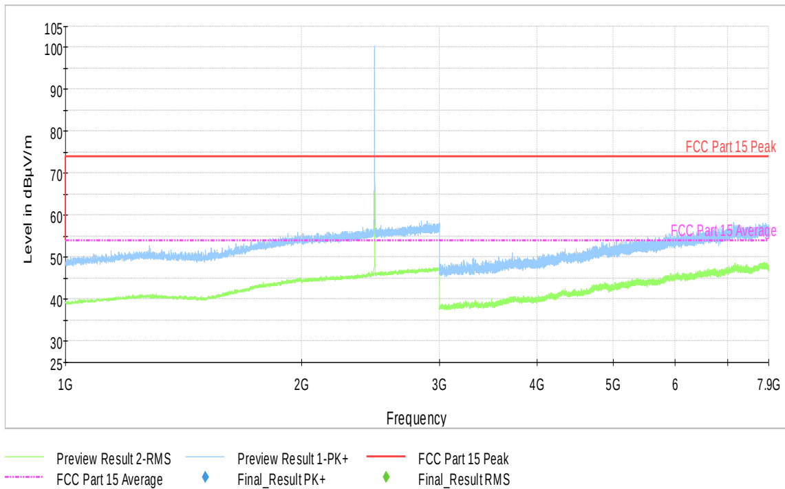
Plot 9-21. Radiated Spurious Emissions (Ch. 39) (1-7.9GHz)
