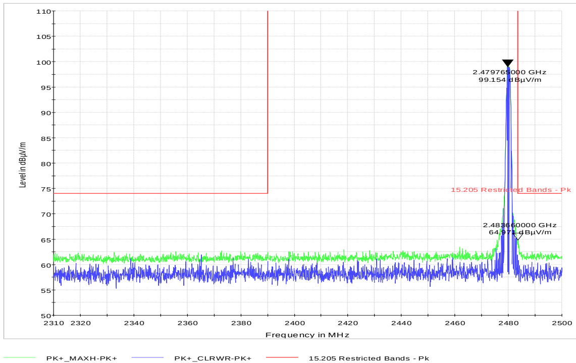
Plot 9-30. Radiated Restricted Band Edge (Ch. 39) Peak
