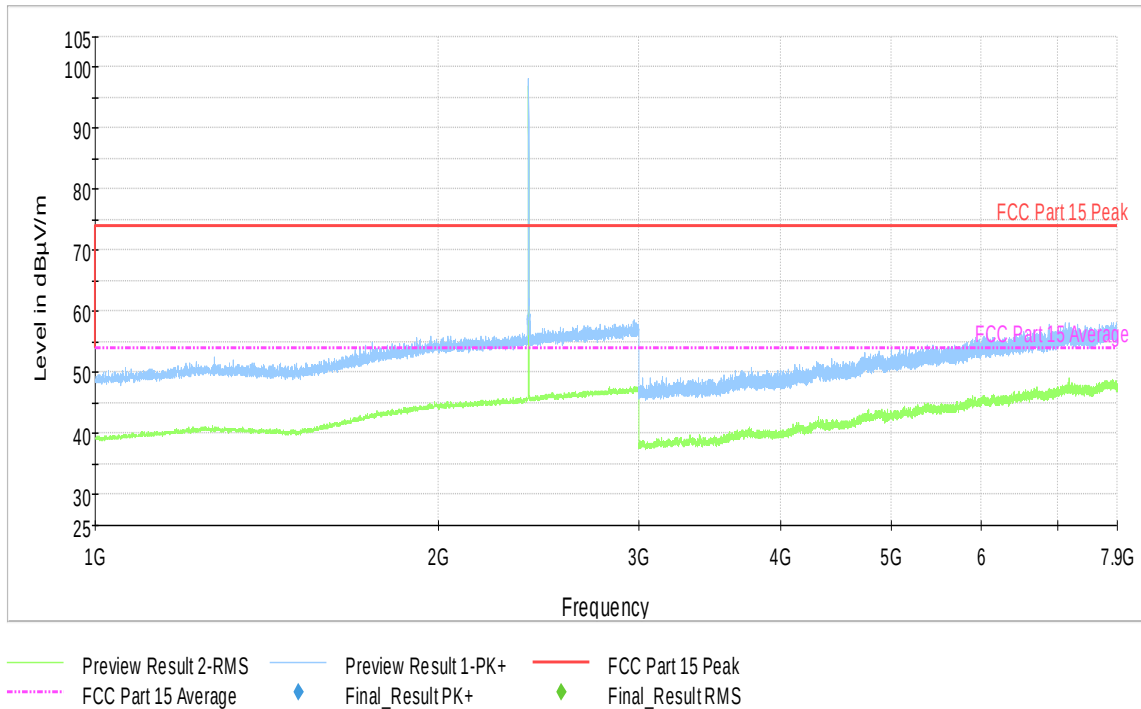
Plot 9-19. Radiated Spurious Emissions (Ch. 0) (1-7.9GHz)
