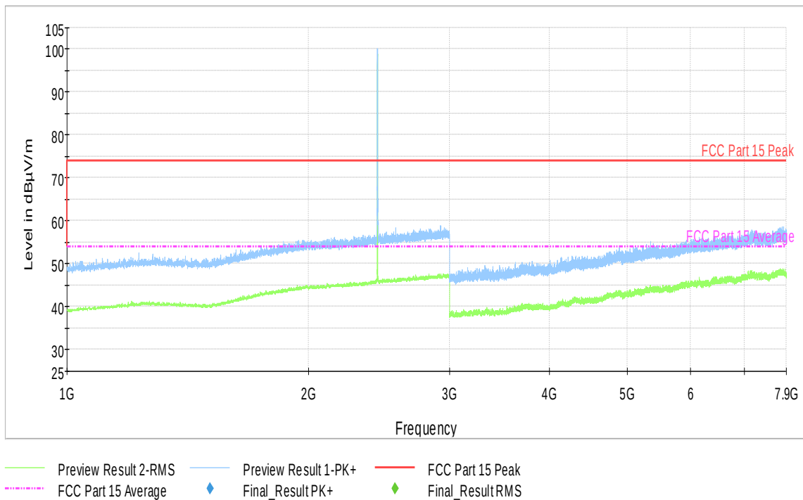
Plot 9-20. Radiated Spurious Emissions (Ch. 19) (1-7.9GHz)
