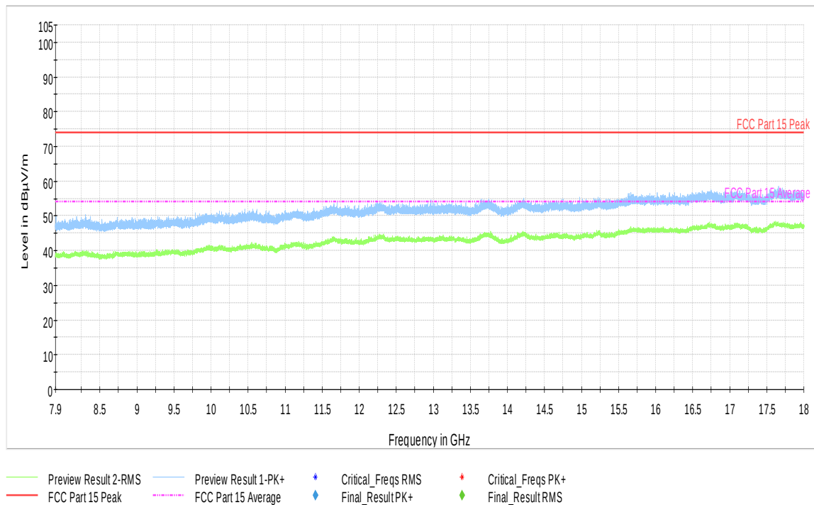
Plot 9-24. Radiated Spurious Emissions (Ch. 39) (7.9-18 GHz)
