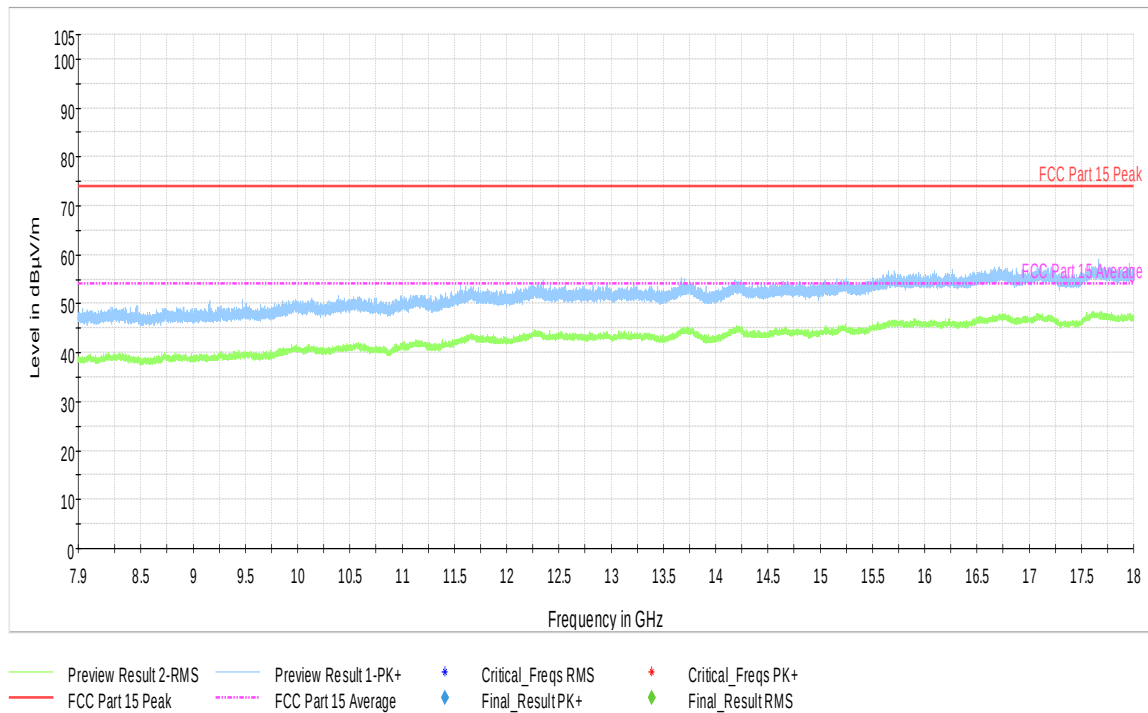
Plot 9-23. Radiated Spurious Emissions (Ch. 19) (7.9-18 GHz)
