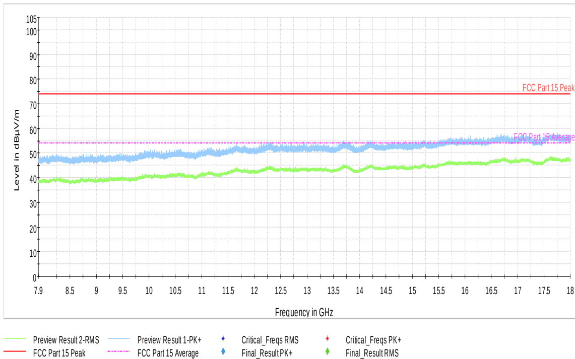
Plot 9-22. Radiated Spurious Emissions (Ch. 0) (7.9-18 GHz)
