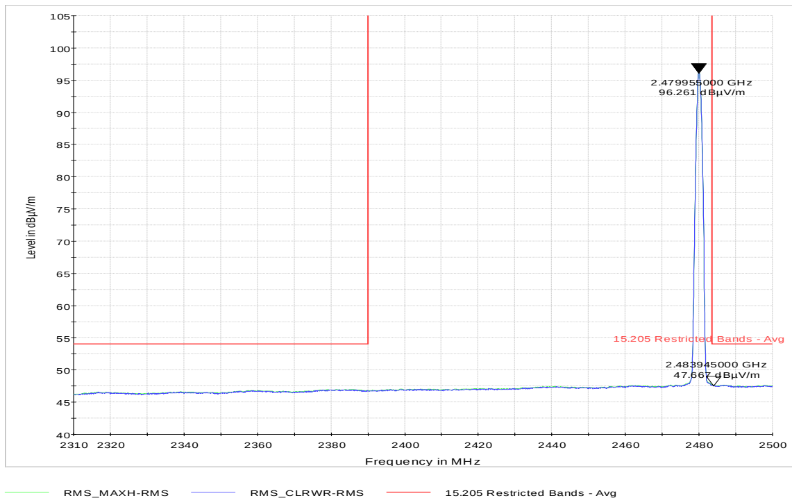
Plot 9-31. Radiated Restricted Band Edge (Ch. 39) Average
