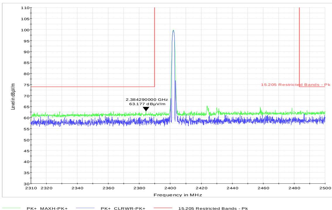
Plot 9 57. Restricted Band Edge 3-DH5 Mode- Ch. 0 (2310-2390MHz) – Peak
