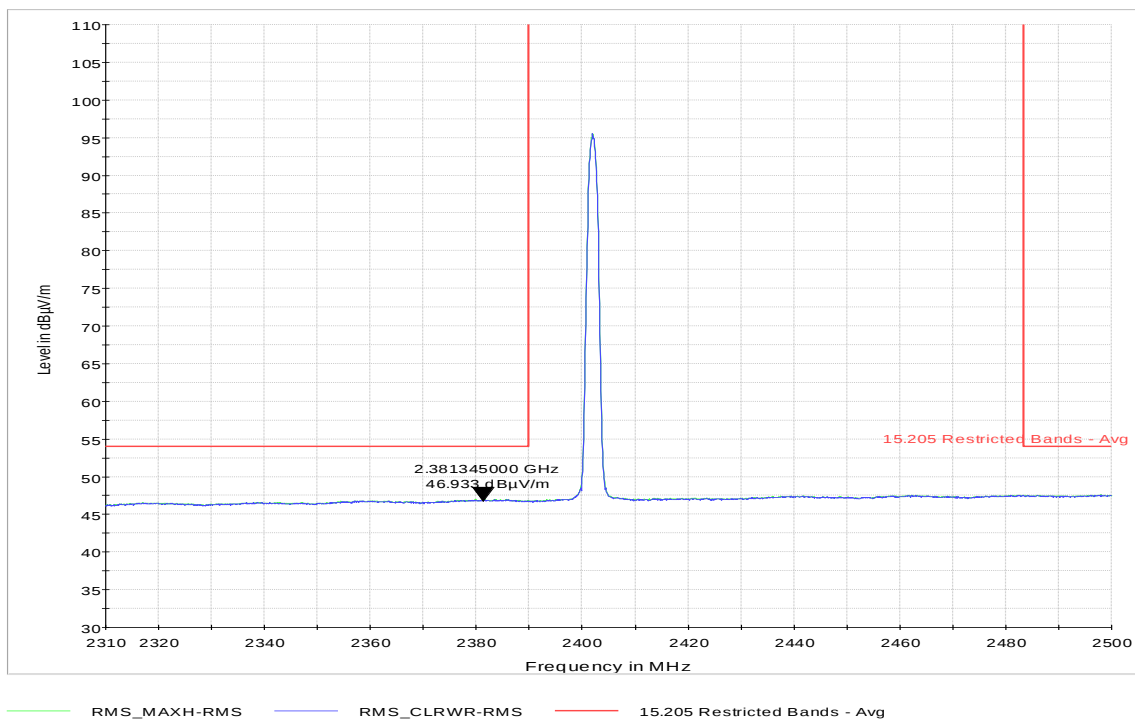
Plot 9-58. Restricted Band Edge 3-DH5 Mode- Ch. 0 (2310-2390MHz) - Average
