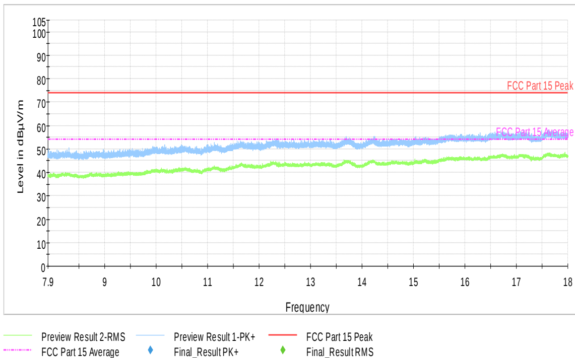
Plot 9-43. Radiated Spurious Emissions (Ch. 39) (7.9 – 18GHz)
