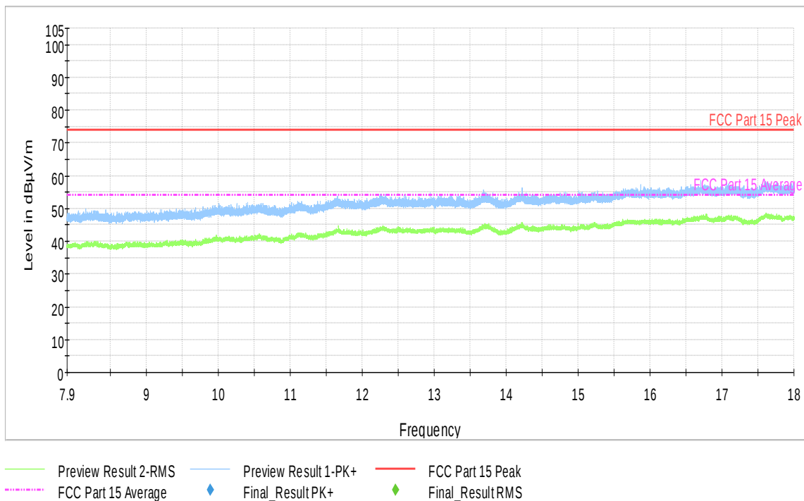
Plot 9-45. Radiated Spurious Emissions (Ch. 78) (7.9 – 18GHz)
