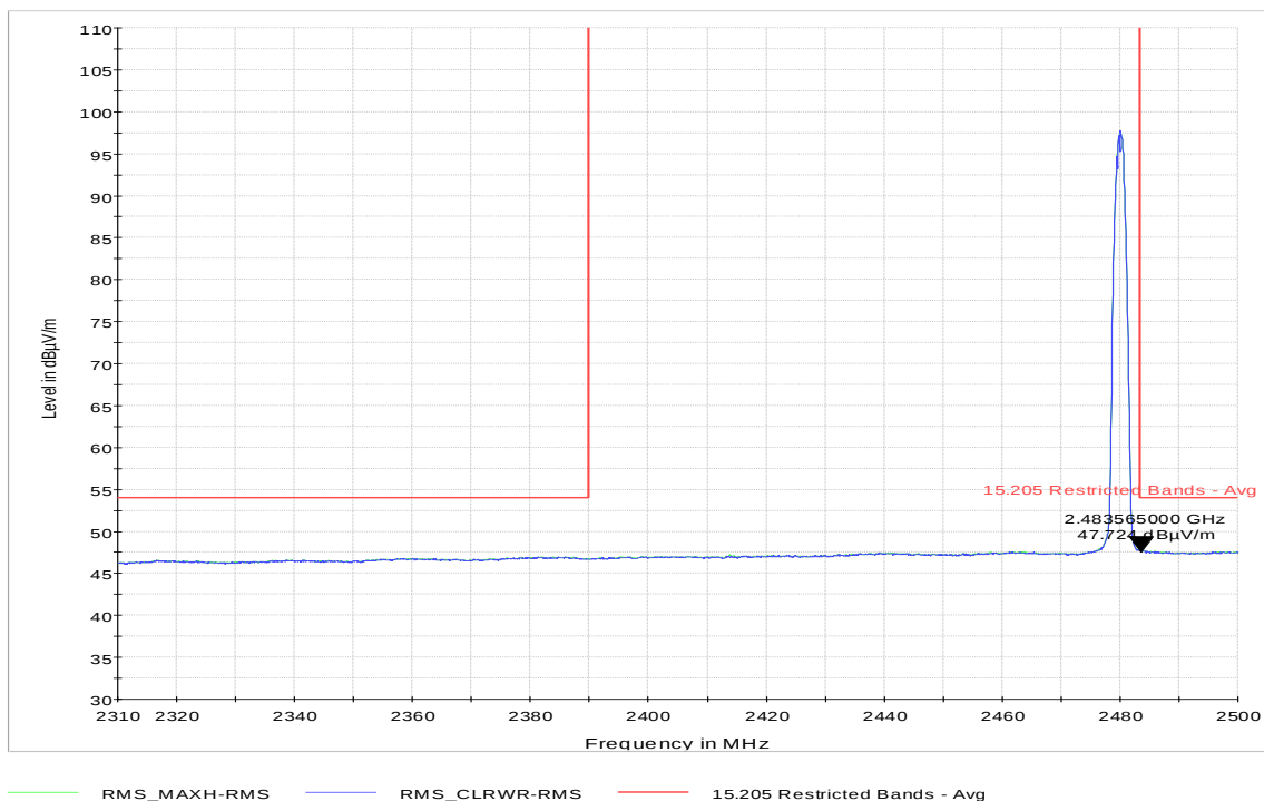
Plot 9-56. Restricted Band Edge 2-DH5 Mode- Ch. 78 (2483.5-2500MHz) – Average
