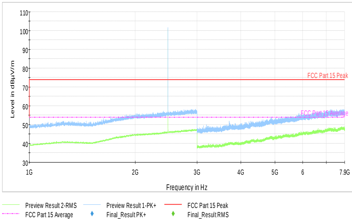
Plot 9-44. Radiated Spurious Emissions (Ch. 78) (1 – 7.9GHz)
