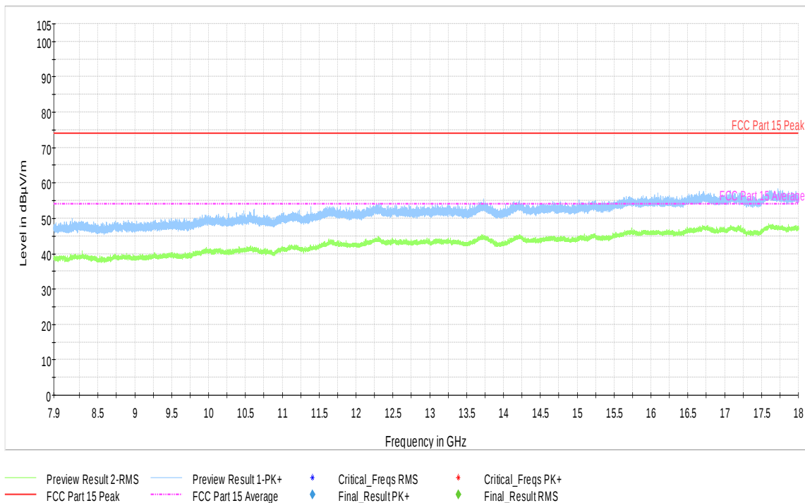
Plot 9-41. Radiated Spurious Emissions (Ch. 0) (7.9 – 18GHz)
