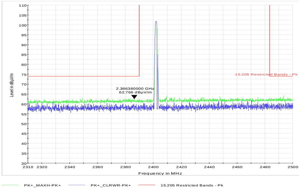
Plot 9 49. Restricted Band Edge 1-DH5 Mode- Ch. 0 (2310-2390MHz) – Peak
