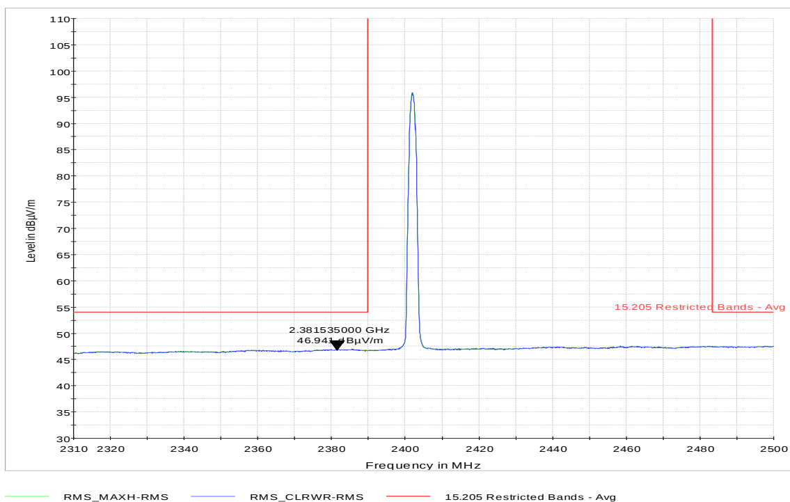
Plot 9-54. Restricted Band Edge 2-DH5 Mode- Ch. 0 (2310-2390MHz) - Average
