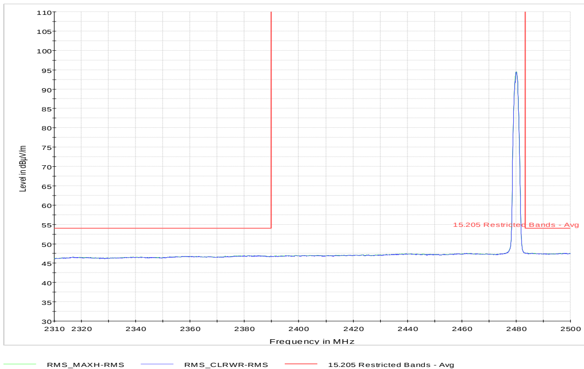
Plot 9-60. Restricted Band Edge 3-DH5 Mode- Ch. 78 (2483.5-2500MHz) - Average
