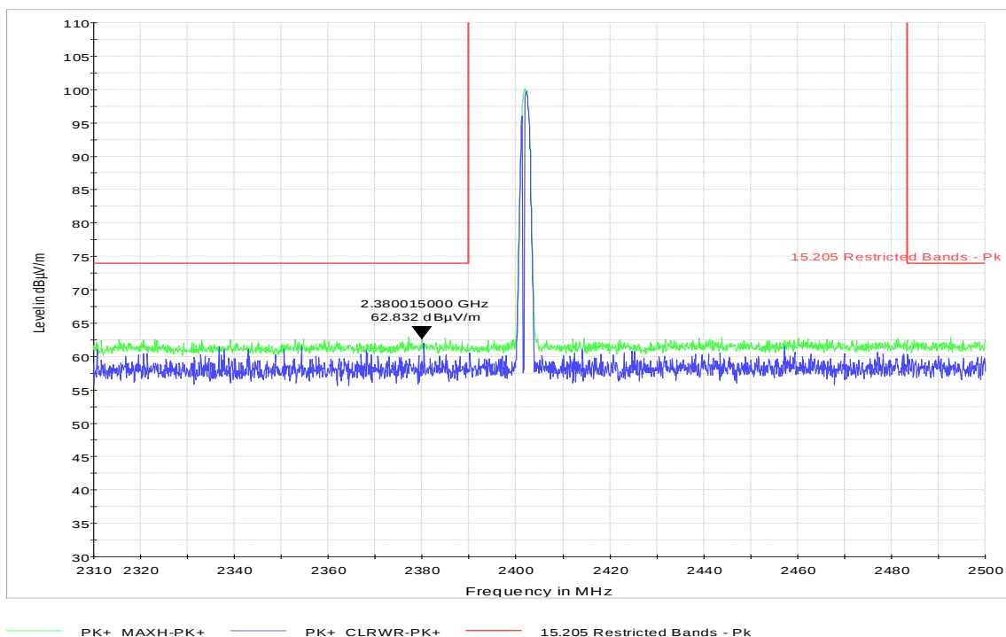
Plot 9 53. Restricted Band Edge 2-DH5 Mode- Ch. 0 (2310-2390MHz) – Peak
