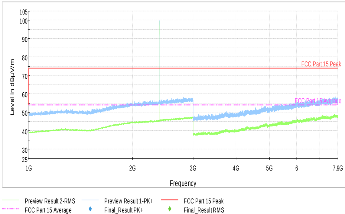
Plot 9-40. Radiated Spurious Emissions (Ch. 0) (1-7.9GHz)
