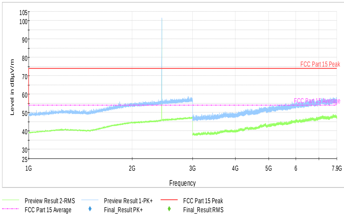
Plot 9-42. Radiated Spurious Emissions (Ch. 39) (1 – 7.9GHz)
