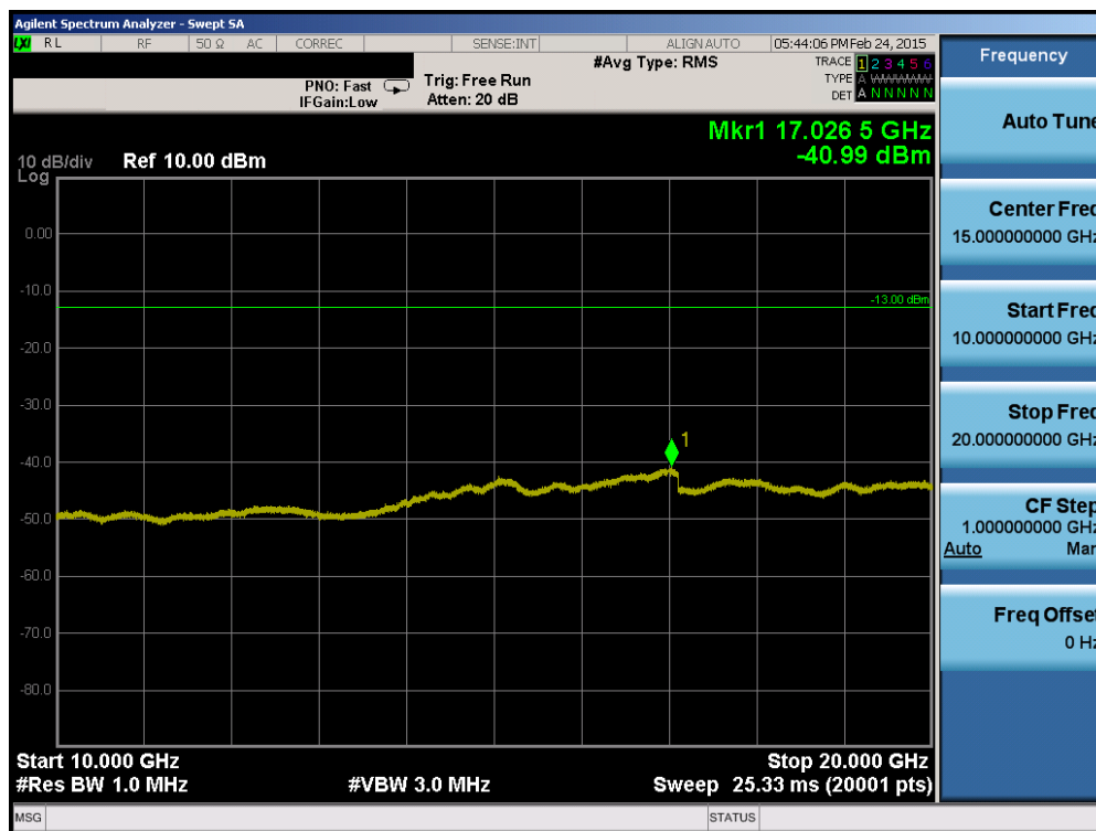
Plot 6-17. Conducted Spurious Plot (PCS WCDMA Mode – Ch. 9400)
