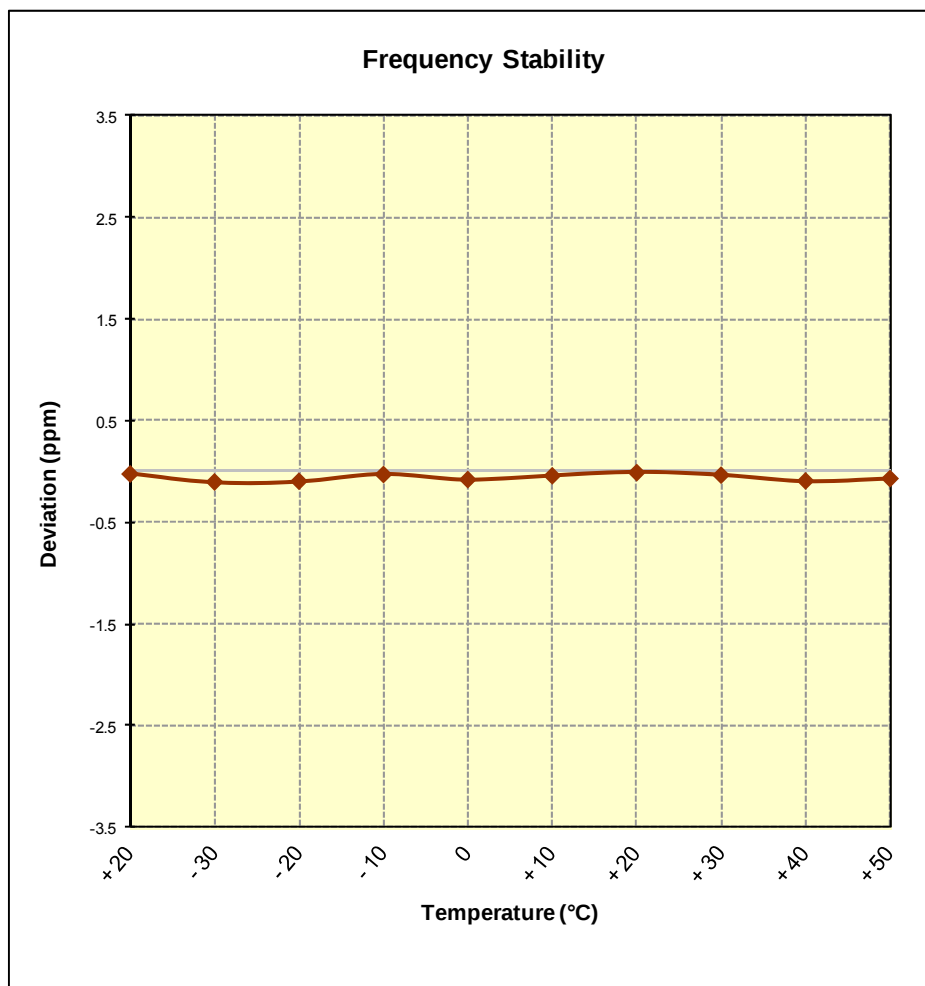
Figure 6-8. Frequency Stability Graph (PCS WCDMA Mode – Ch. 9400)
