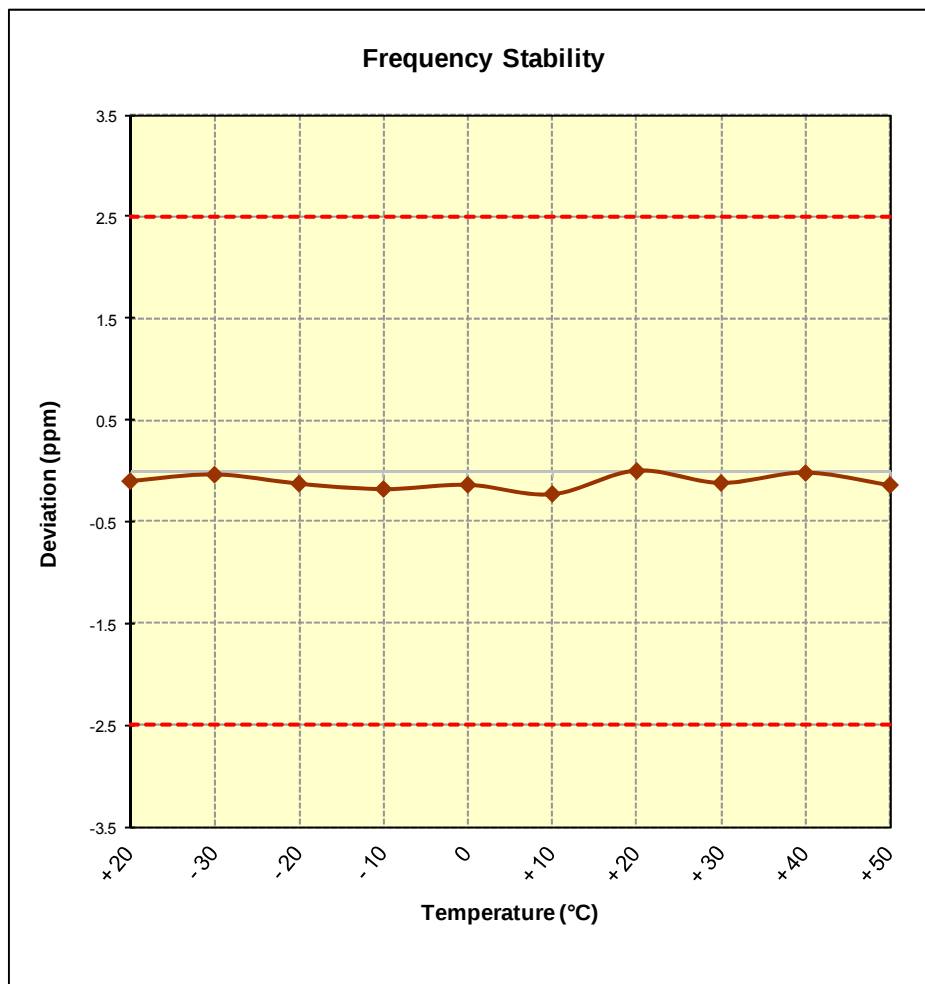
Figure 6-7. Frequency Stability Graph (Cellular WCDMA Mode – Ch. 4183)
