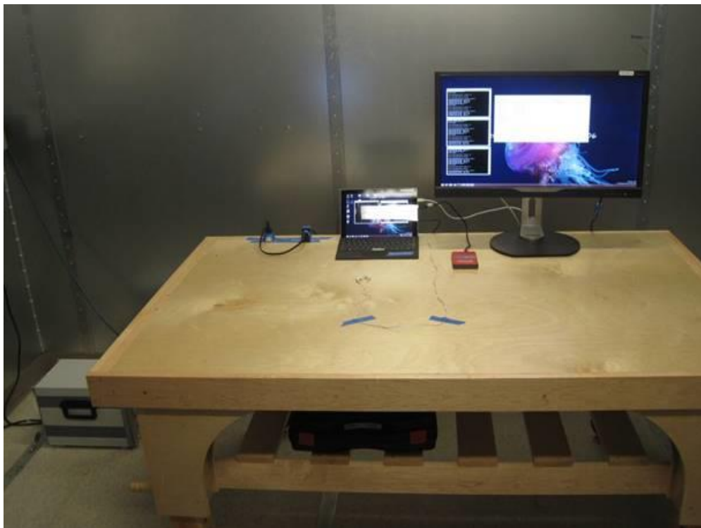
Fig.6 AC Line Conducted Emissions Measurements Test Setup
