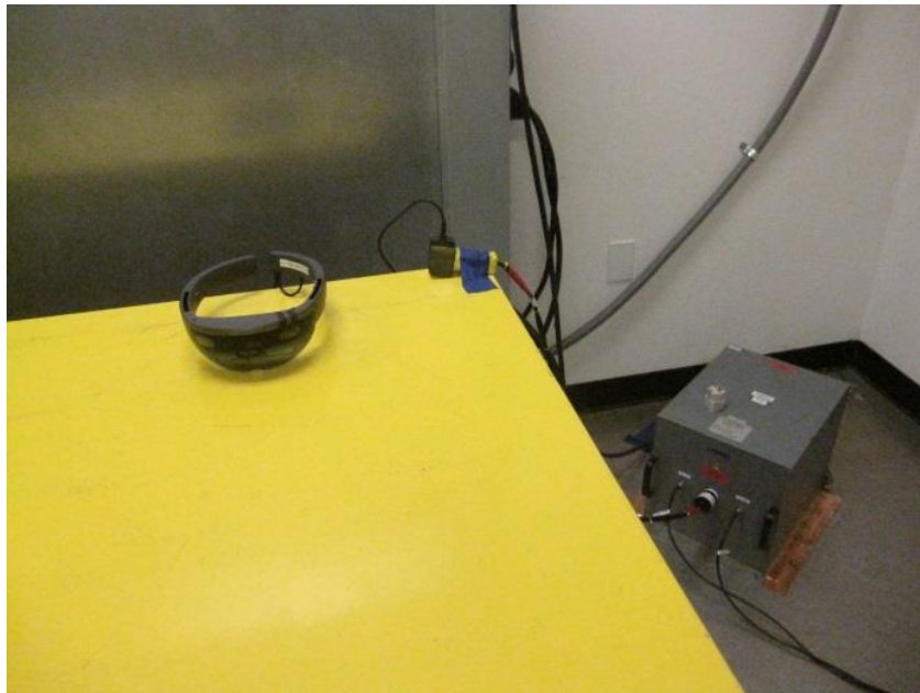
LINE CONDUCTED FRONT VIEW
