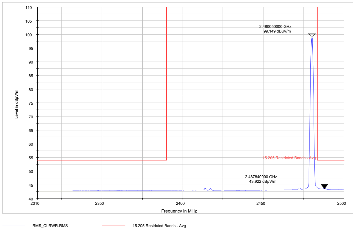
Plot 9-46. Restricted Band Edge 1-DH5 Mode- Ch. 78 (2483.5-2500MHz) – Average
