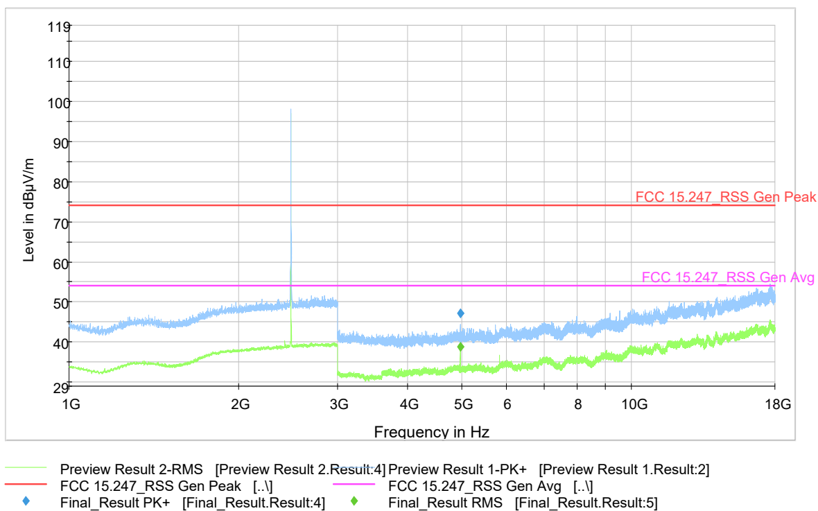
Plot 9-41. Radiated Spurious Emissions (Ch. 78) (1-18 GHz)
