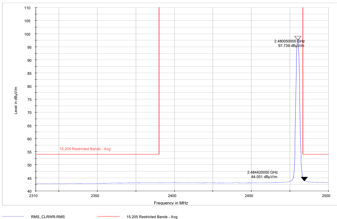
Plot 9-50. Restricted Band Edge 2-DH5 Mode- Ch. 78 (2483.5-2500MHz) – Average
