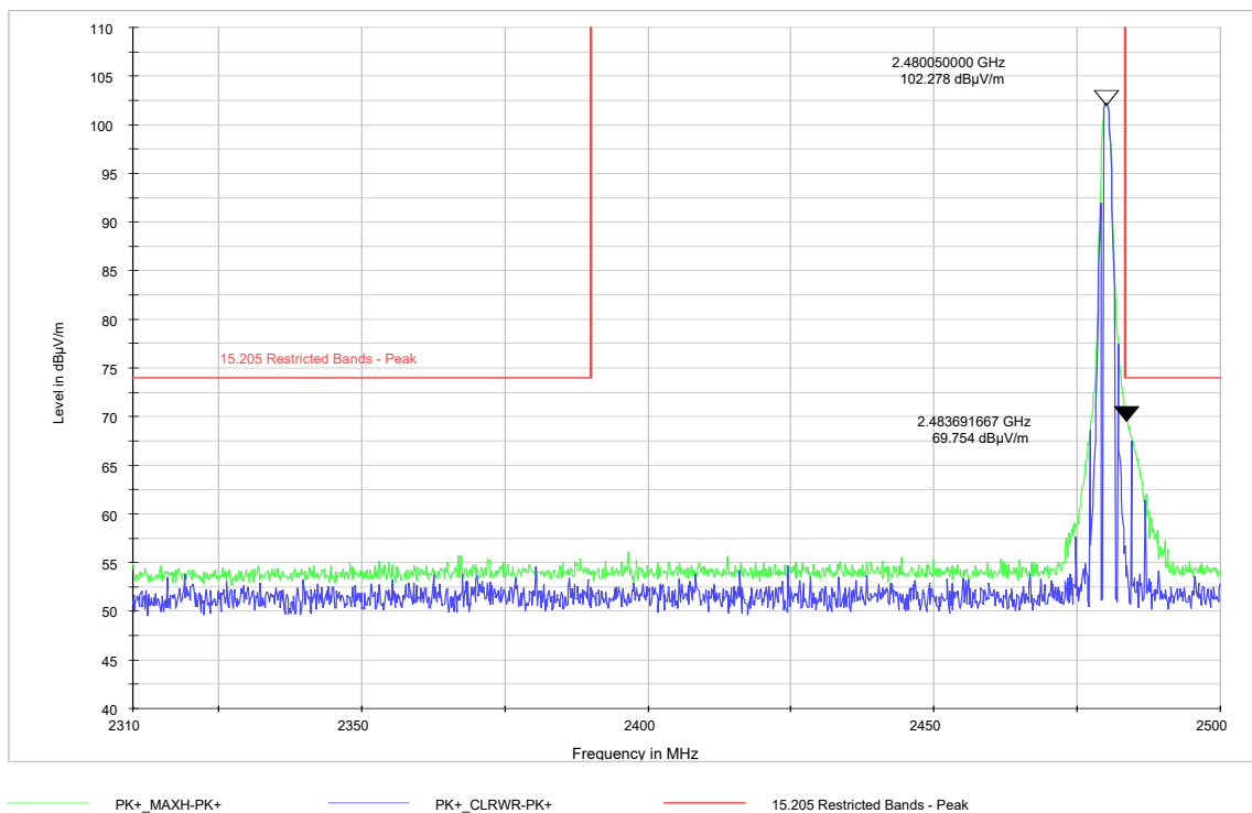
Plot 9-53. Restricted Band Edge 3-DH5 Mode- Ch. 78 (2483.5-2500MHz) – Peak
