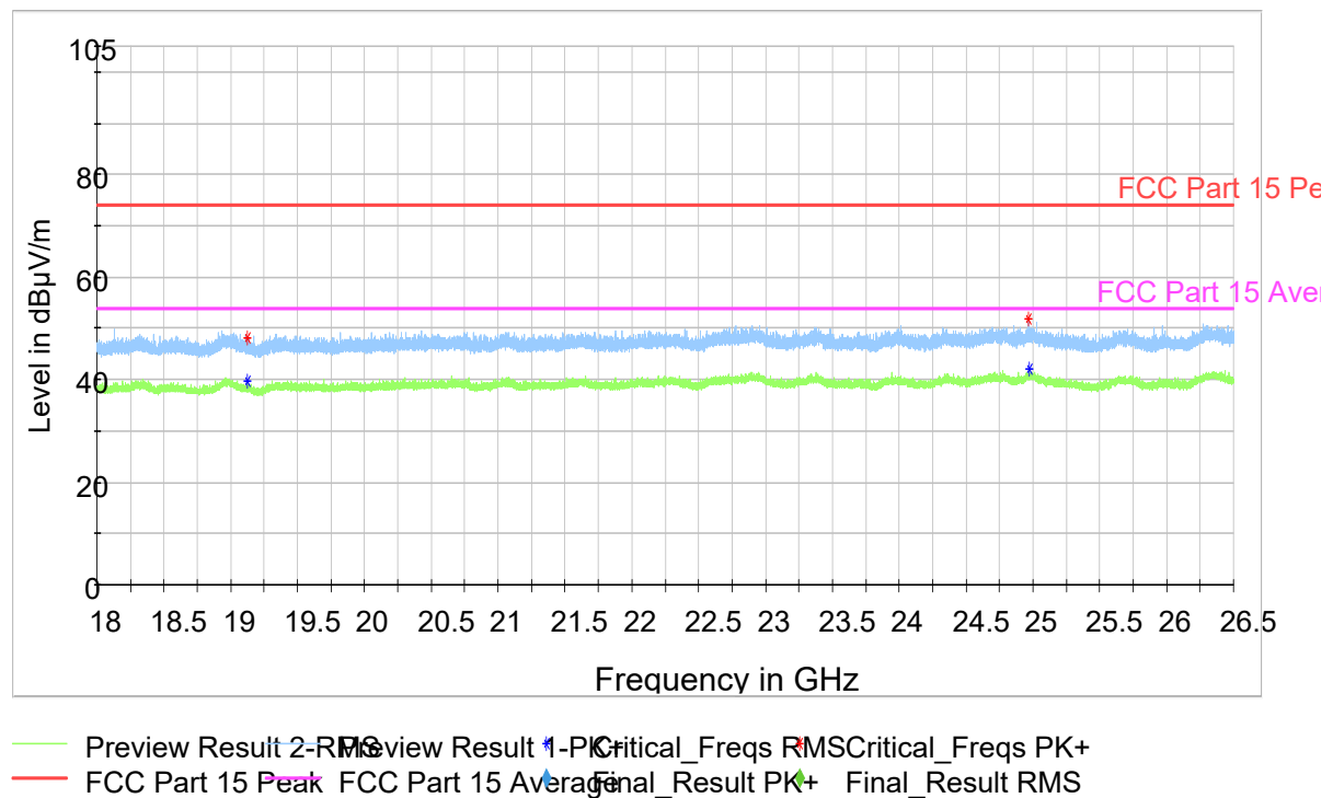
Plot 9-42. Radiated Spurious Emissions (Ch. 0) (18 - 26GHz)
