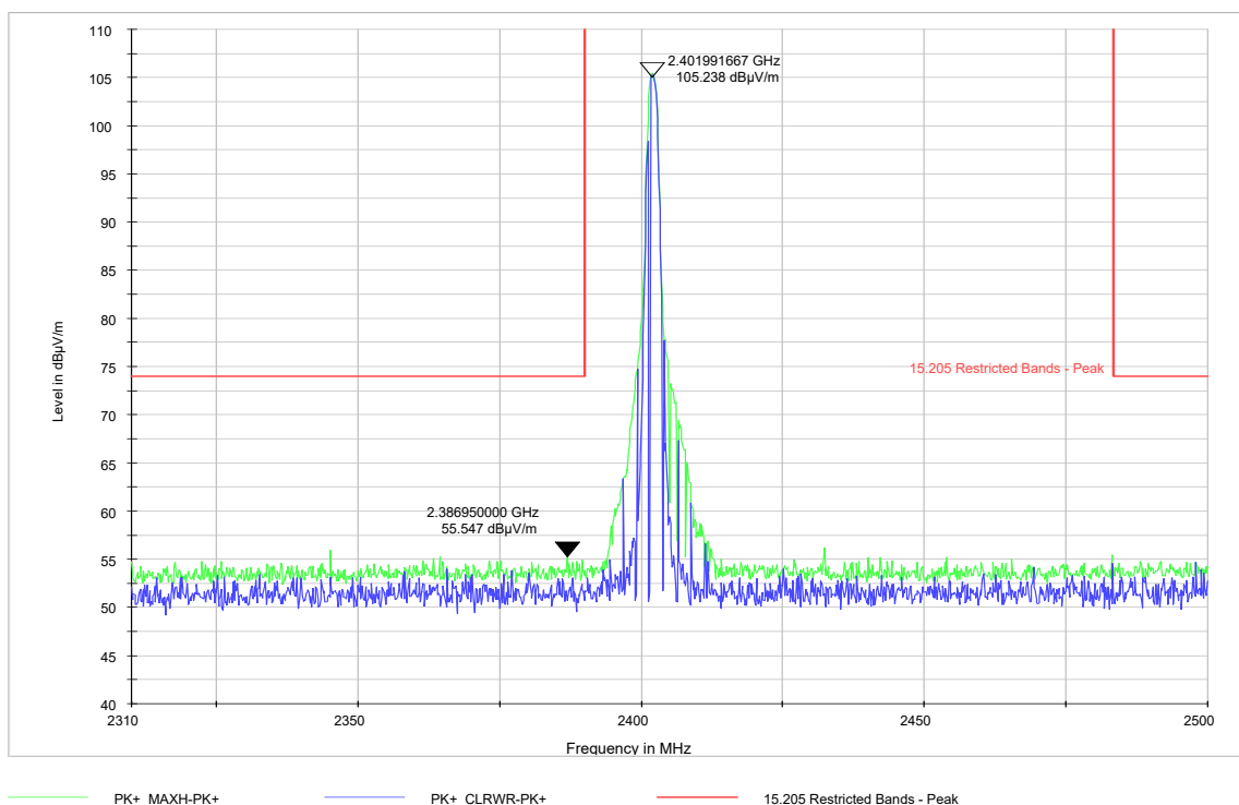
Plot 9-51. Restricted Band Edge 3-DH5 Mode- Ch. 0 (2310-2390MHz) – Peak
