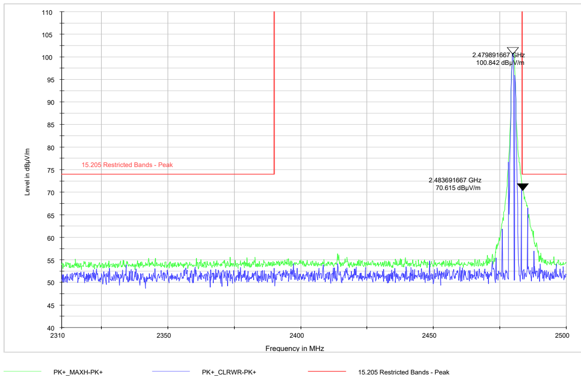
Plot 9-45. Restricted Band Edge 1-DH5 Mode- Ch. 78 (2483.5-2500MHz) – Peak
