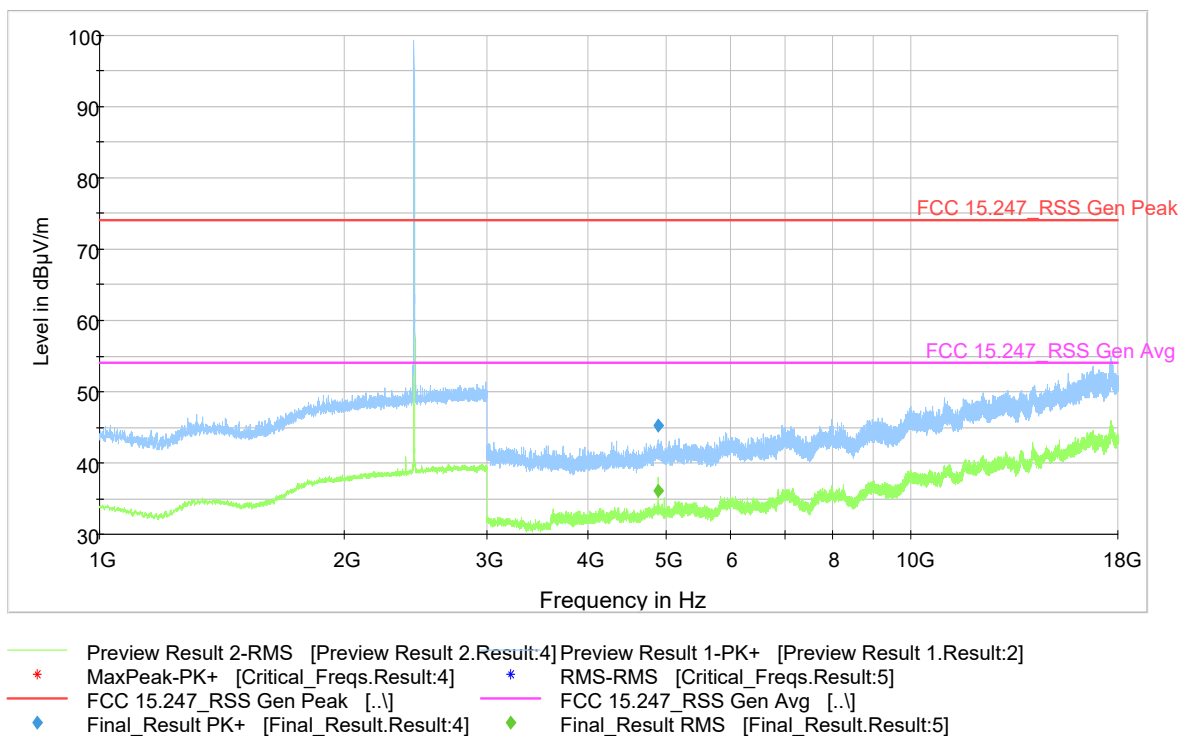
Plot 9-40. Radiated Spurious Emissions (Ch. 39) (1-18 GHz)
