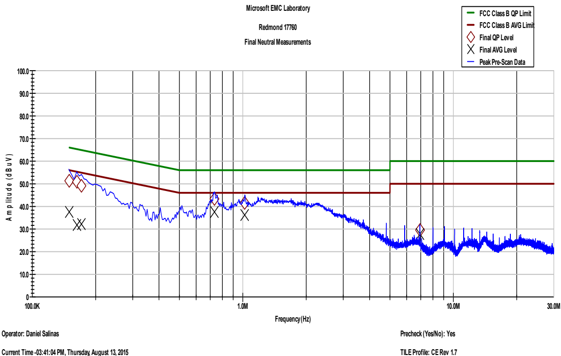
Plot 9-56. AC Line Conducted Emissions- Neutral (150 kHz- 30 MHz)
