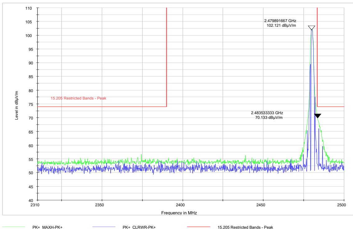
Plot 9-49. Restricted Band Edge 2-DH5 Mode- Ch. 78 (2483.5-2500MHz) – Peak
