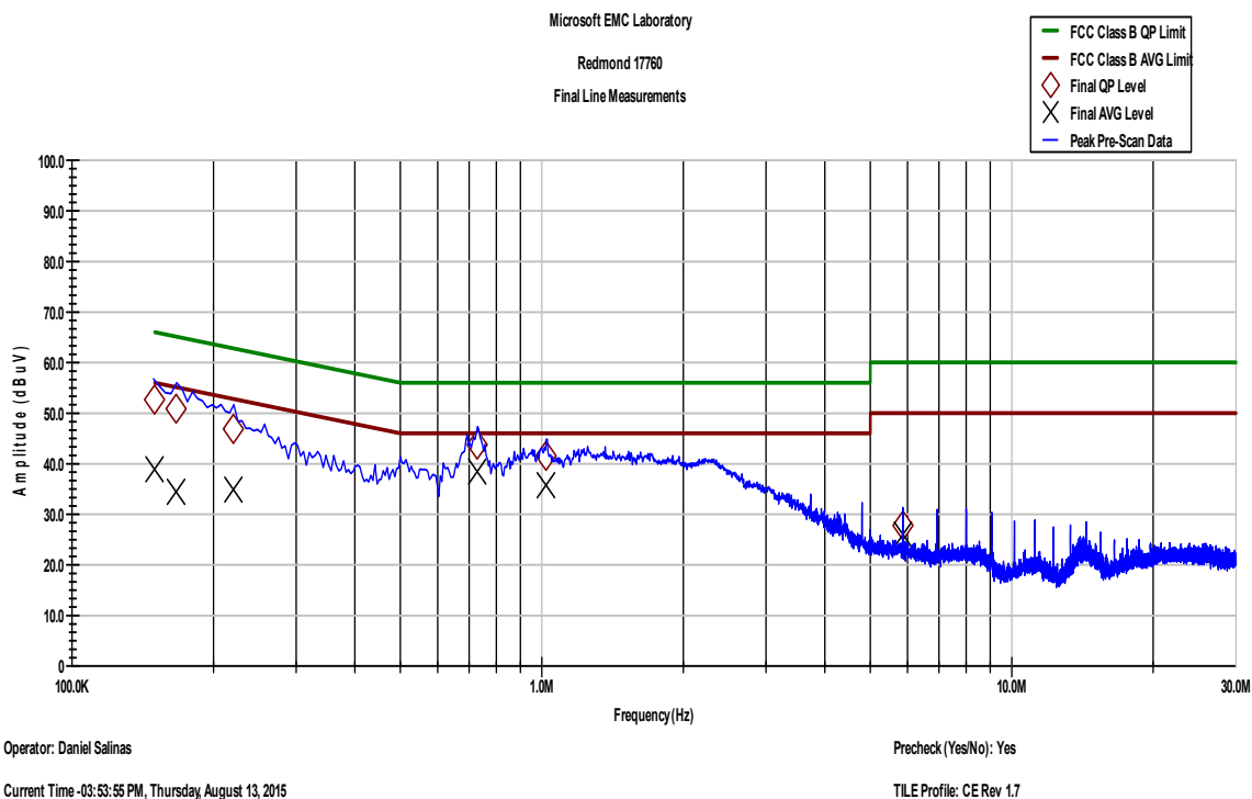
Plot 9-55. AC Line Conducted Emissions- Line (150 kHz- 30 MHz)
