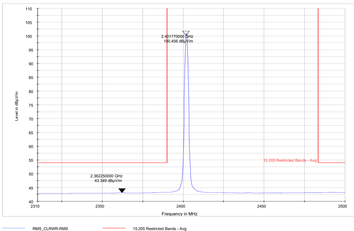
Plot 9-52. Restricted Band Edge 3-DH5 Mode- Ch. 0 (2310-2390MHz) - Average
