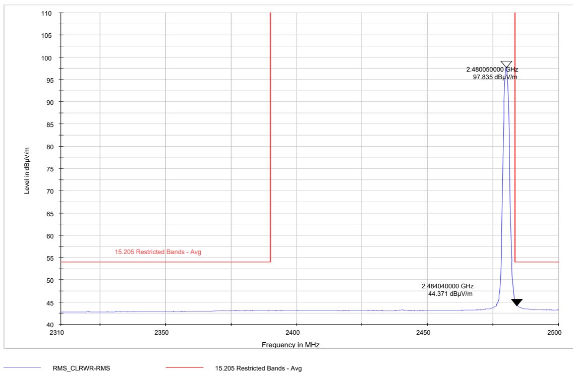
Plot 9-54. Restricted Band Edge 3-DH5 Mode- Ch. 78 (2483.5-2500MHz) - Average
