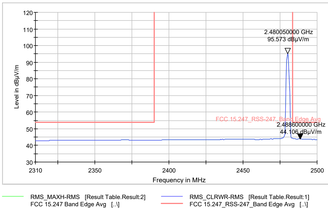
Plot 9-30. Radiated Restricted Band Edge (Ch. 39) Average
