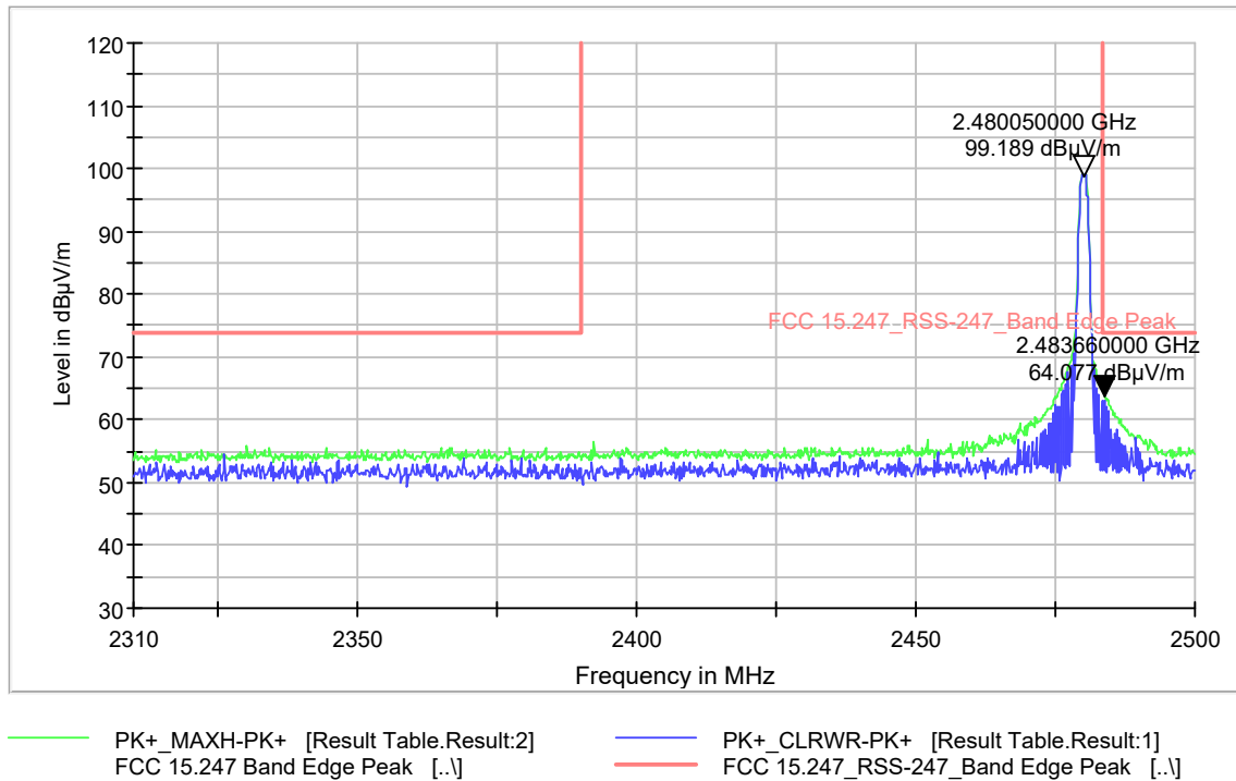
Plot 9-29. Radiated Restricted Band Edge (Ch. 39) Peak
