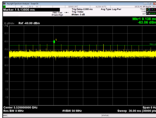
Figure 3. Radar Burst Level at -63dBm: Radar Type 0 (5520 MHz 20 MHz BW)
