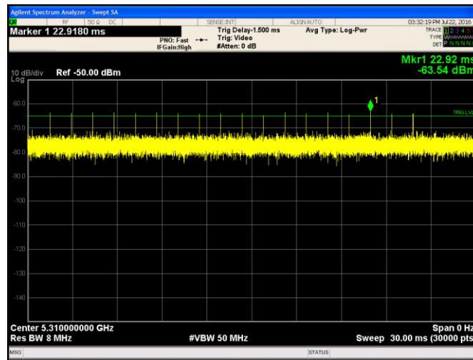
Figure 6. Radar Burst Level at -63dBm: Radar Type 0 (5310 MHz 40 MHz BW)
