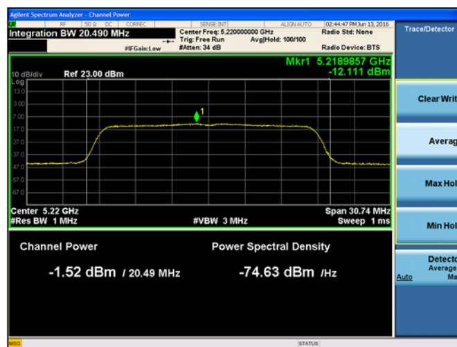
Plot 9-11. Maximum Conducted Output Power and PSD 802.11n (Ch. 44)
