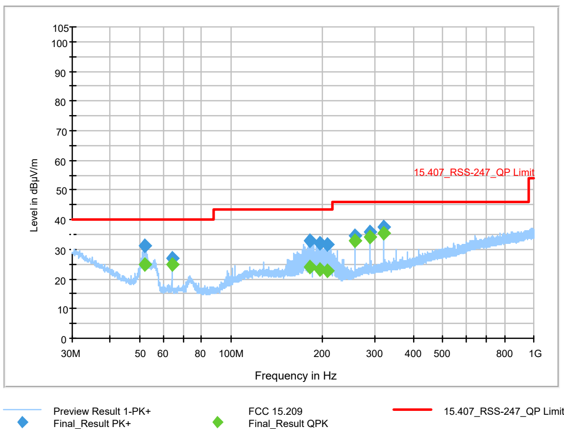
Plot 9-19. Radiated Spurious Emissions 30-1000 MHz Tx 802.11n (Ch. 149)
