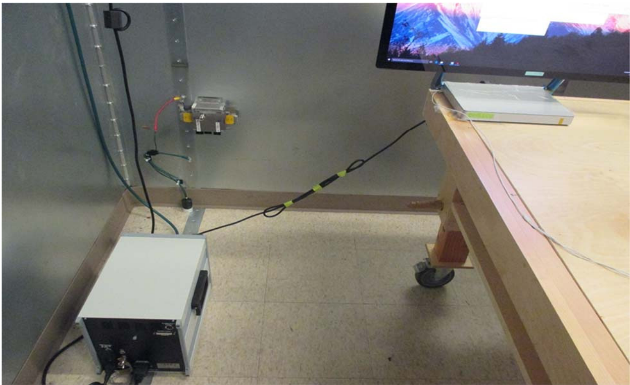
Fig.10 AC Line Conducted Emissions Measurements Test Setup- LISN Connection
