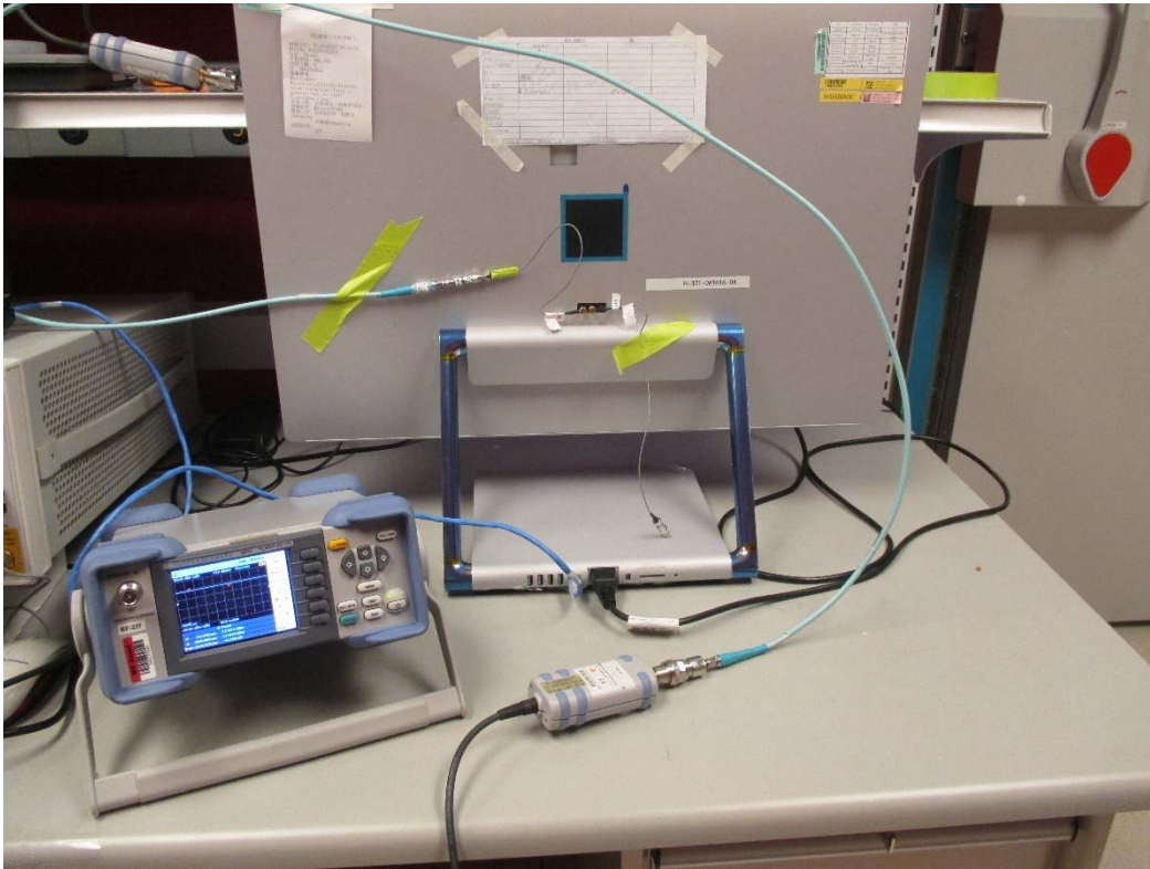
Fig.7 Antenna port Conducted Measurements Test Setup
