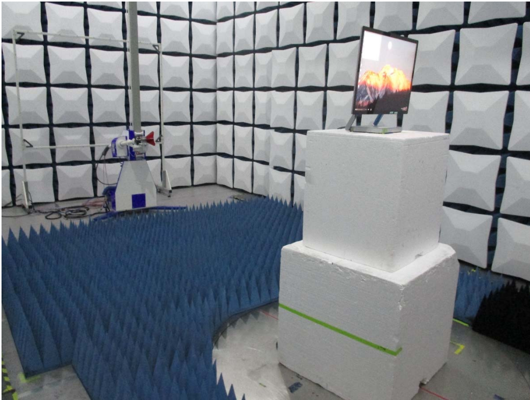
Fig 3. Radiated Spurious Emissions Test Setup (1-18 GHz) Test Site 2
