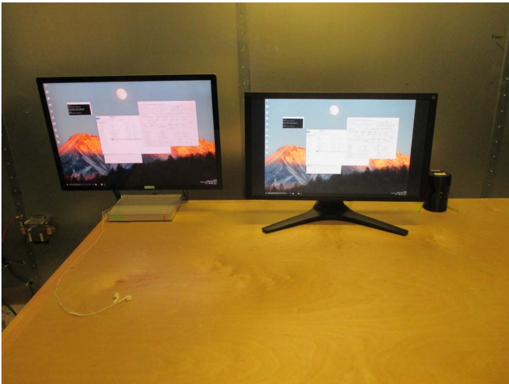
Fig.8 AC Line Conducted Emissions Measurements Test Setup- Front View
