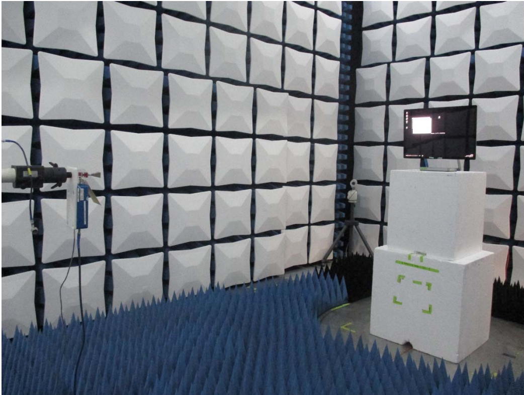
Fig.5 Radiated Spurious Emissions (26.5 - 40GHz) Test Site2
