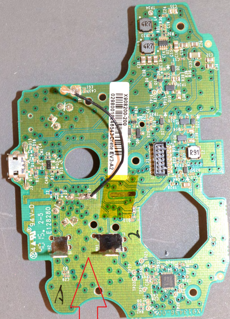
Main dual band antennas
