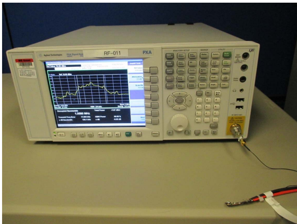
Figure 6 Conducted Measurement Test Setup
