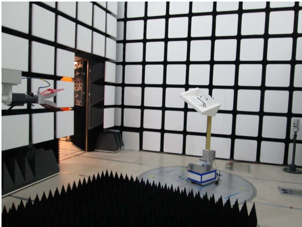
Fig.4 Radiated Spurious Emissions Test Setup (1-18 GHz)
