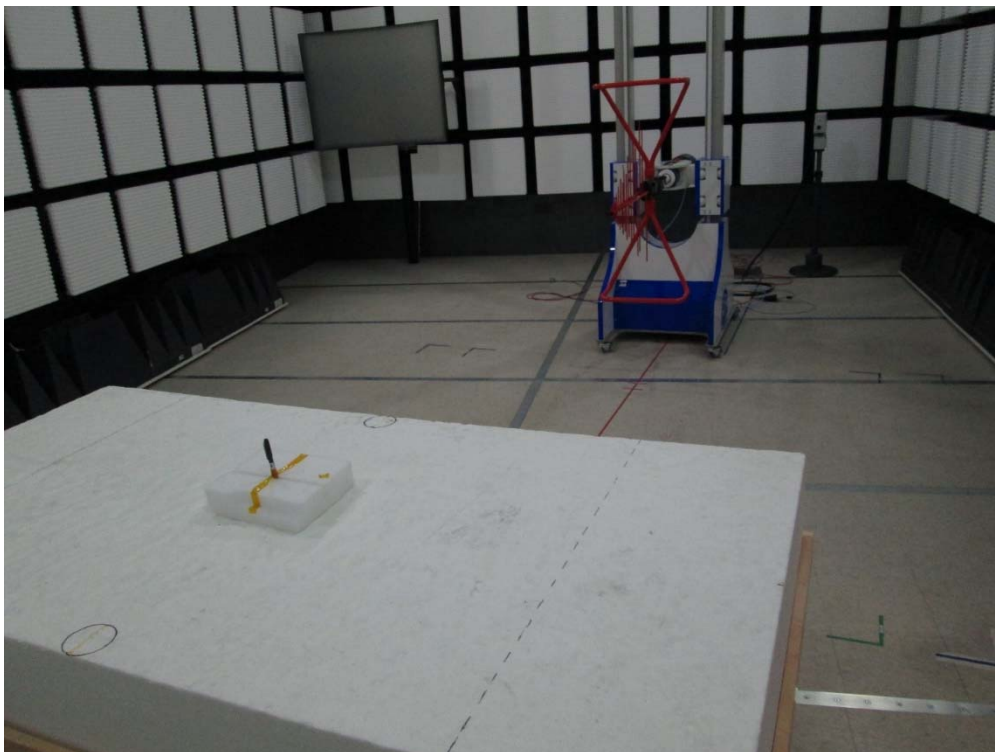
Fig.2 EUT- Standing Position
