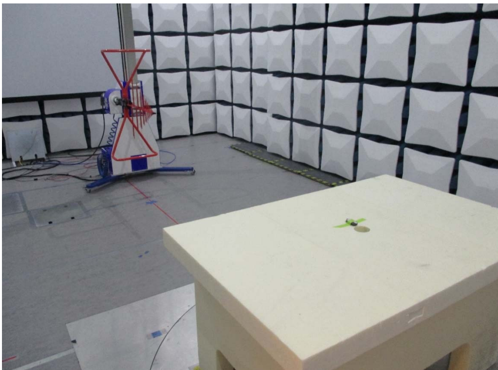
Fig.2 Radiated Spurious Emissions Test Setup (30MHz – 1GHz)
