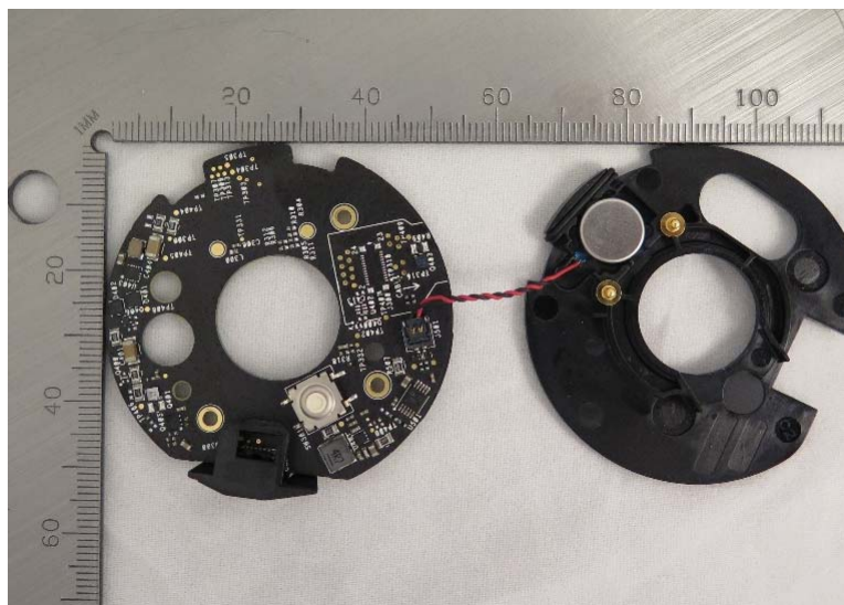
Fig.2 Internal Board- Bottom View
