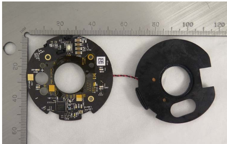
Fig.1 Internal Board- Top View
