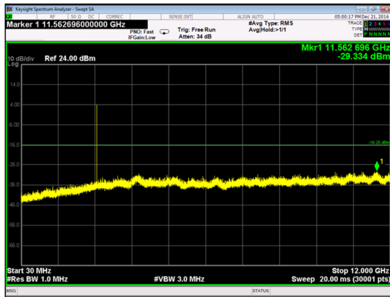
Plot 9-43. Conducted Spurious Emissions 30-12000 MHz: 1-DH5 Mode (Ch. 78)
