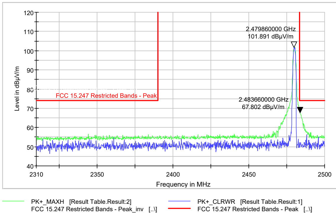
Plot 9-67. Restricted Band Edge 3-DH5 Mode- Ch. 78 (2483.5-2500MHz) – Peak
