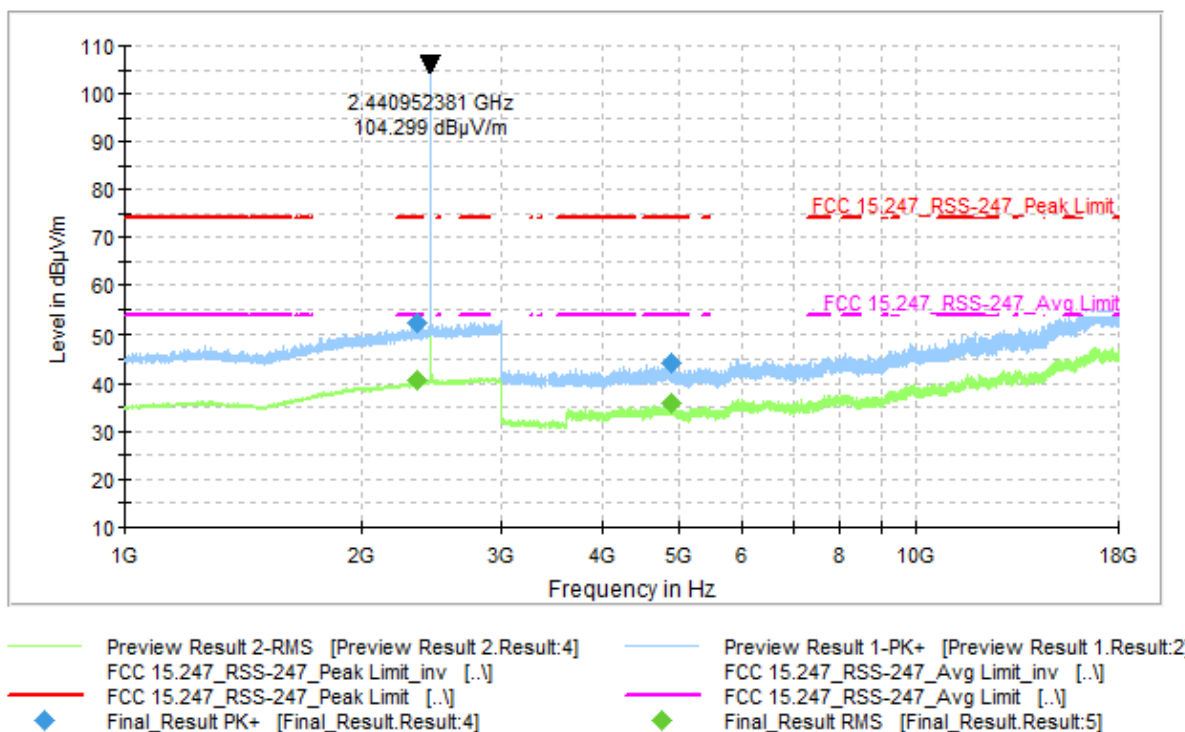
Plot 9-71. Radiated Spurious Emissions (Ch. 39) 2-DH5 (1-18 GHz)
