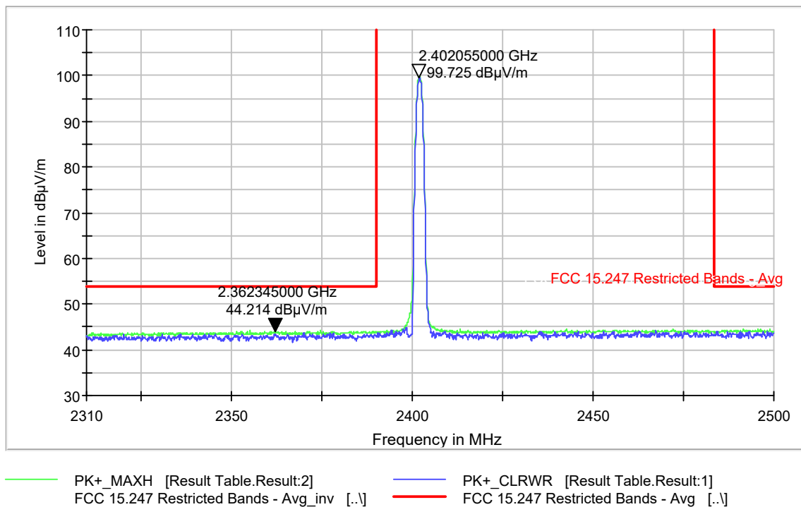
Plot 9-66. Restricted Band Edge 3-DH5 Mode- Ch. 0 (2310-2390MHz) - Average
