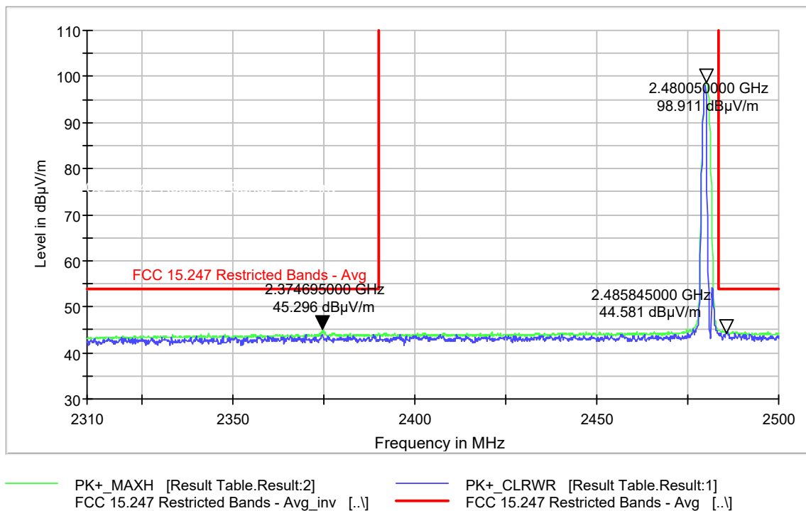
Plot 9-64. Restricted Band Edge 2-DH5 Mode- Ch. 78 (2483.5-2500MHz) – Average
