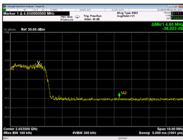
Plot 9-36. High Channel Band 2-DH5 Mode (Hopping enabled)
