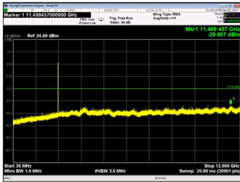
Plot 9-45. Conducted Spurious Emissions 30-12000 MHz: 2-DH5 Mode (Ch. 0)
