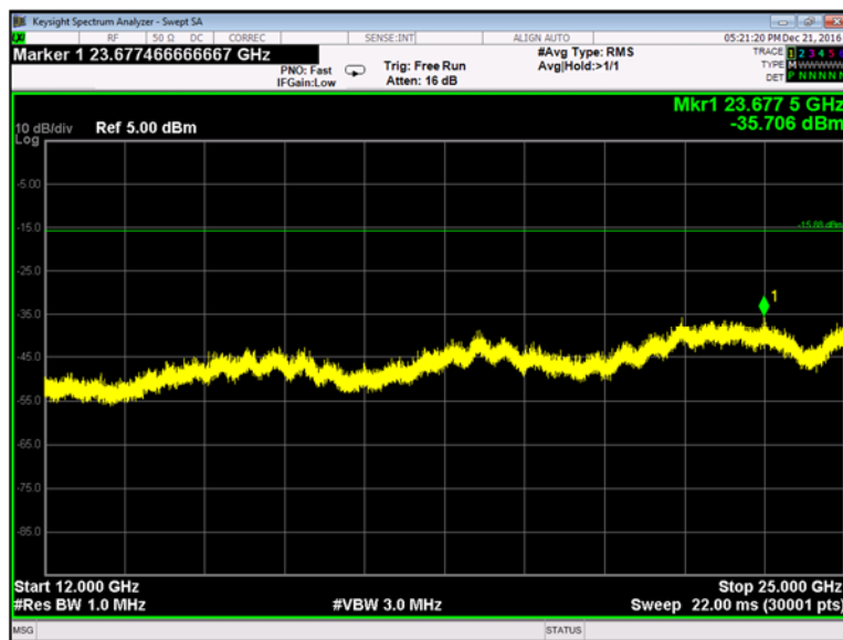
Plot 9-40. Conducted Spurious Emissions 12-25 GHz: 1-DH5 Mode (Ch. 0)
