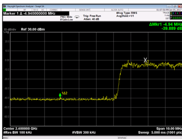
Plot 9-35. Low Channel Band edge 2-DH5 Mode (Hopping enabled)
