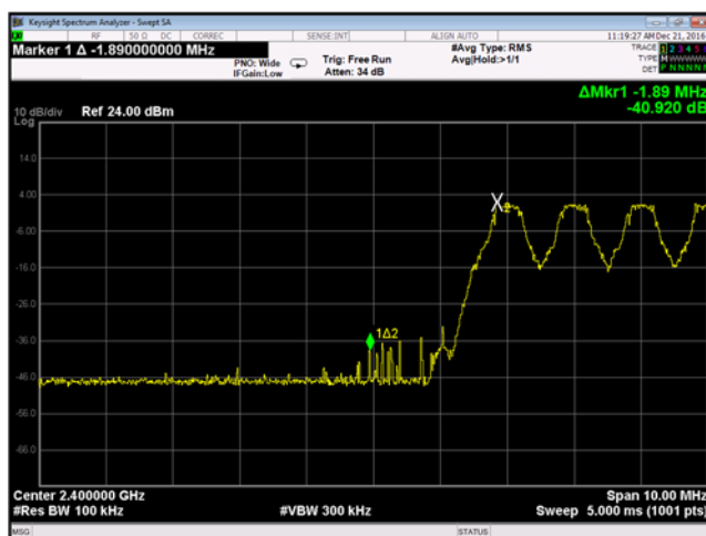
Plot 9-33. Low Channel Band edge 1-DH5 Mode (Hopping enabled)
