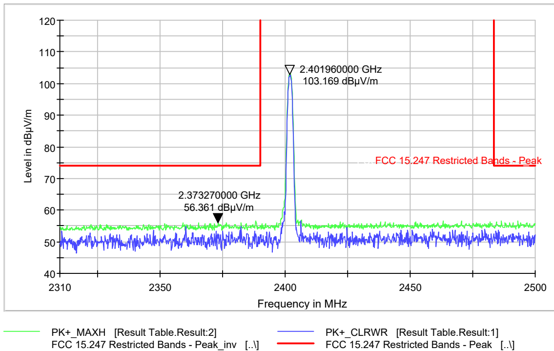
Plot 9-65. Restricted Band Edge 3-DH5 Mode- Ch. 0 (2310-2390MHz) – Peak
