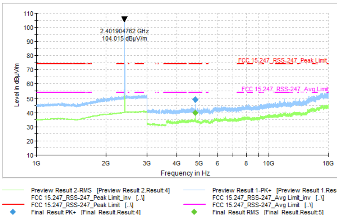
Plot 9-70. Radiated Spurious Emissions (Ch. 0) 2-DH5 (1-18 GHz)
