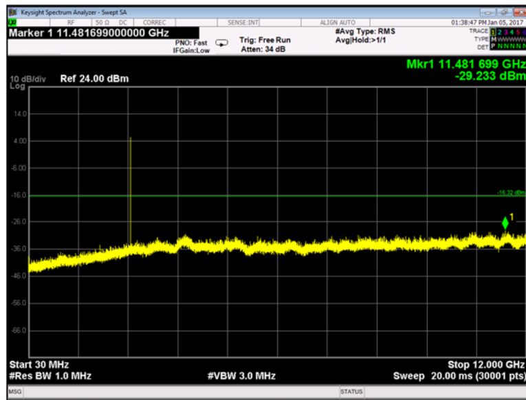
Plot 9-49. Conducted Spurious Emissions 30-12000 MHz: 2-DH5 Mode (Ch. 78)
