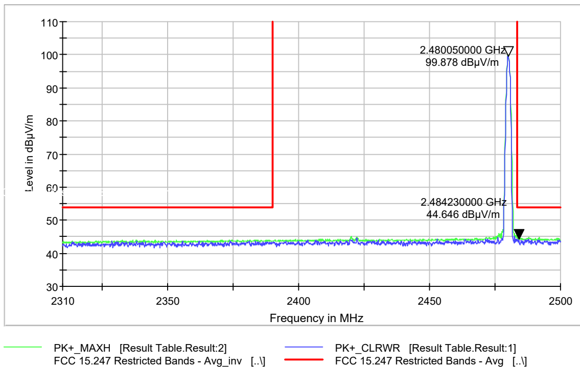
Plot 9-60. Restricted Band Edge 1-DH5 Mode- Ch. 78 (2483.5-2500MHz) – Average
