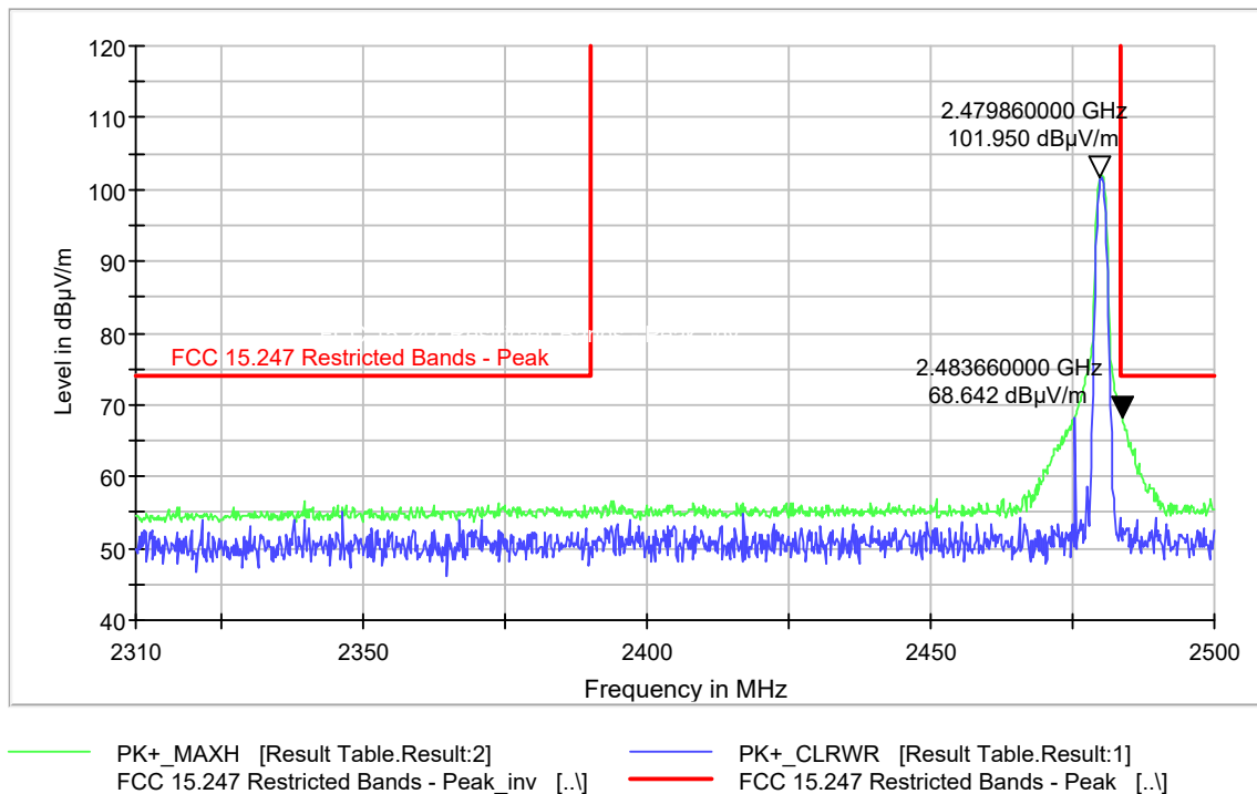
Plot 9-63. Restricted Band Edge 2-DH5 Mode- Ch. 78 (2483.5-2500MHz) – Peak
