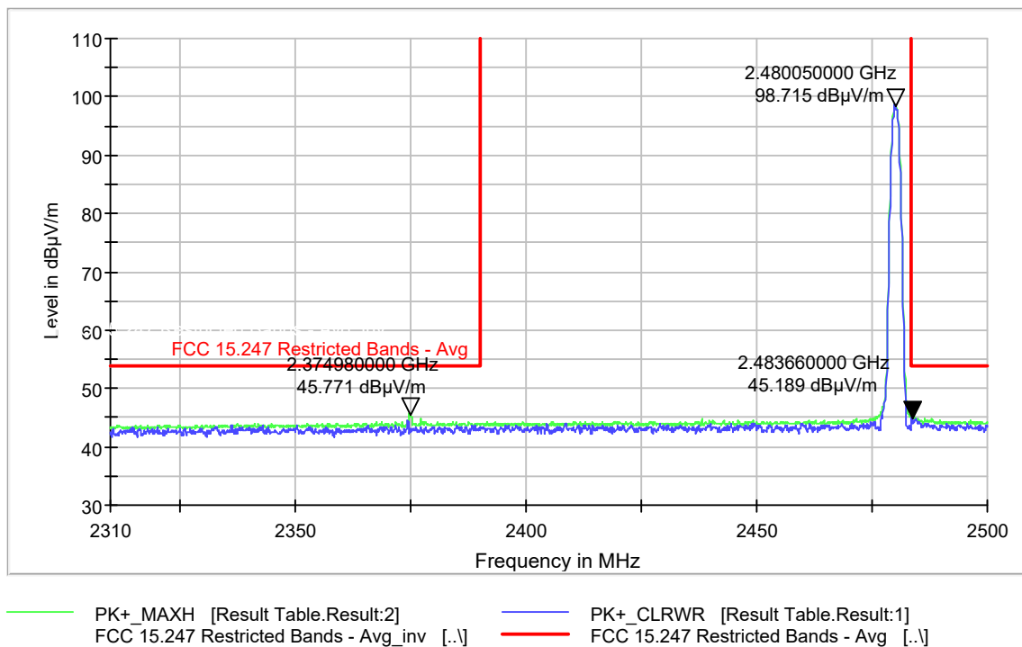
Plot 9-68. Restricted Band Edge 3-DH5 Mode- Ch. 78 (2483.5-2500MHz) - Average
