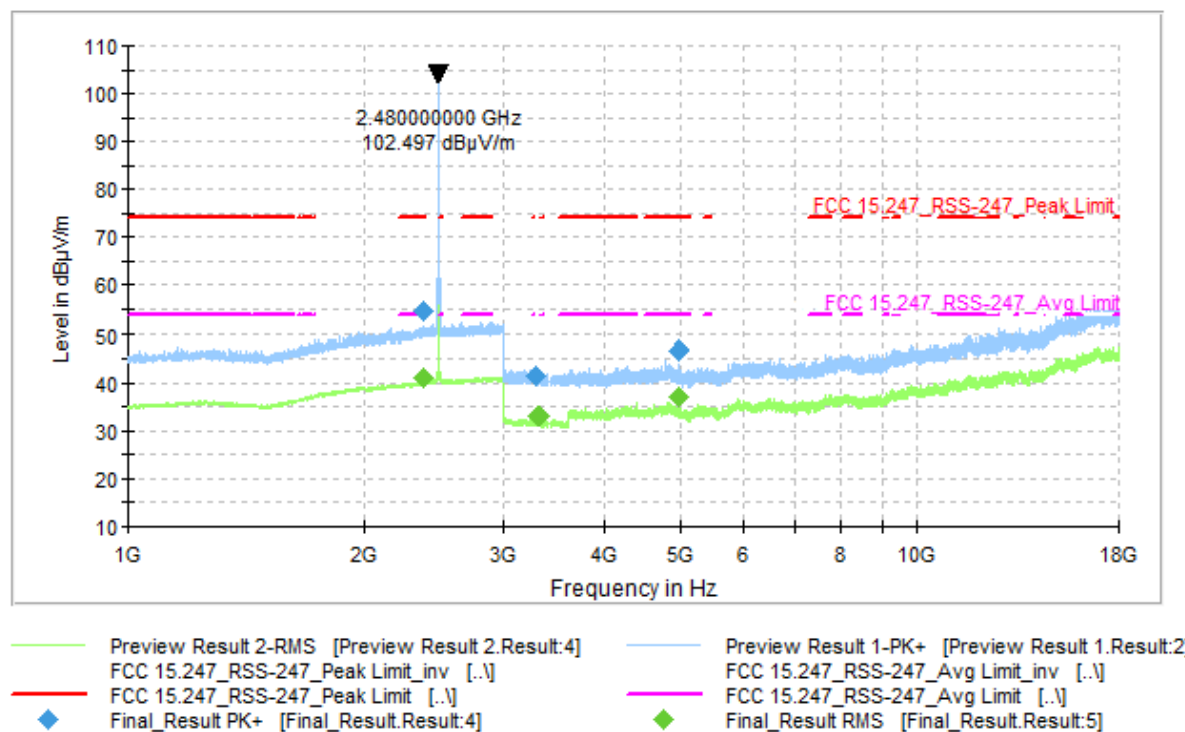
Plot 9-72. Radiated Spurious Emissions (Ch. 78) 2-DH5 (1-18 GHz)
