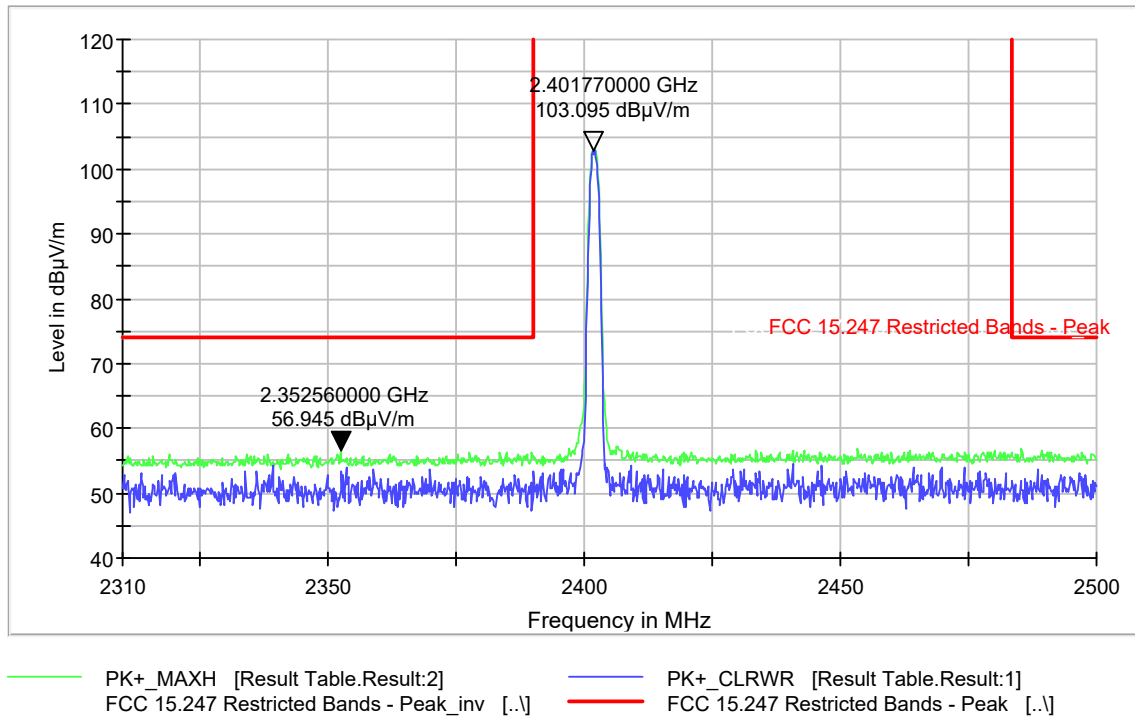
Plot 9-61. Restricted Band Edge 2-DH5 Mode- Ch. 0 (2310-2390MHz) – Peak
