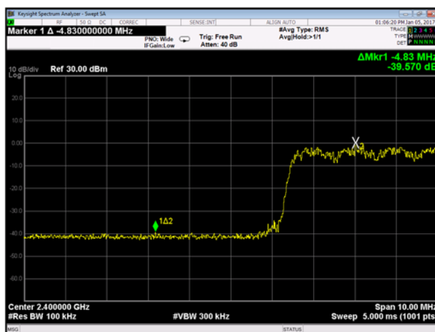
Plot 9-37. Low Channel Band edge 3-DH5 Mode (Hopping enabled)
