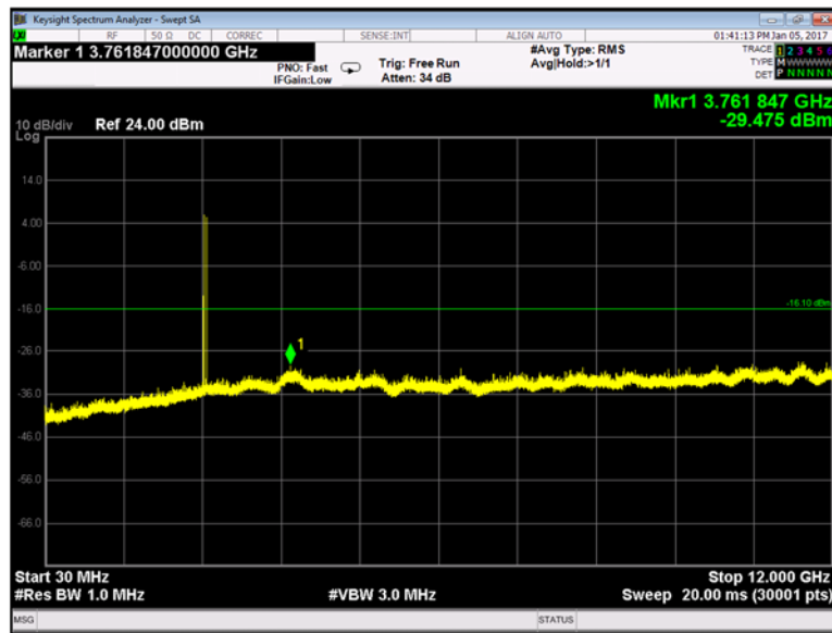
Plot 9-47. Conducted Spurious Emissions 30-12000 MHz: 2-DH5 Mode (Ch. 39)
