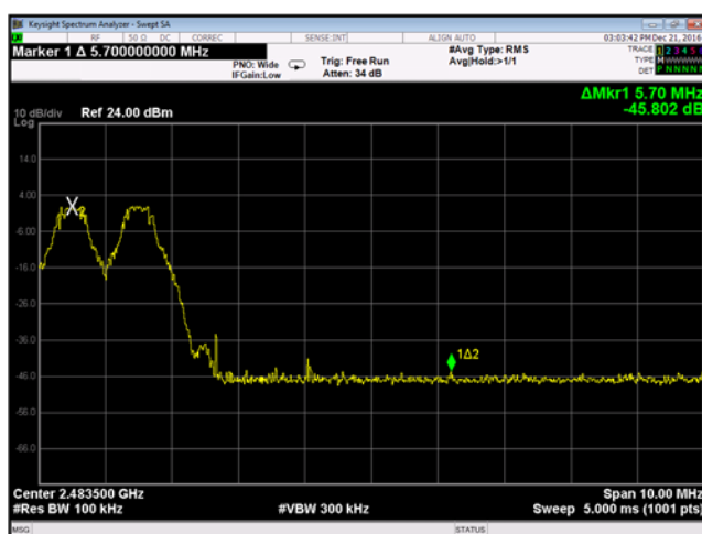
Plot 9-34. High Channel Band 1-DH5 Mode (Hopping enabled)
