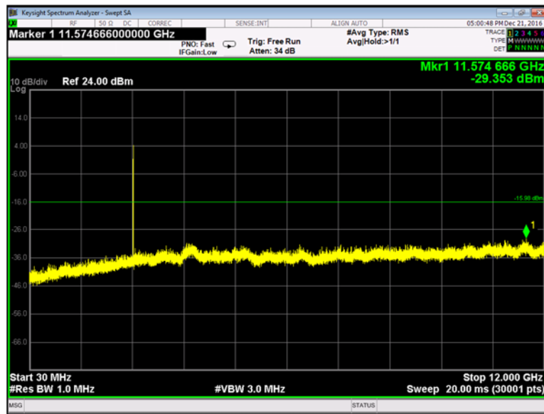
Plot 9-41. Conducted Spurious Emissions 30-12000 MHz: 1-DH5 Mode (Ch. 39)
