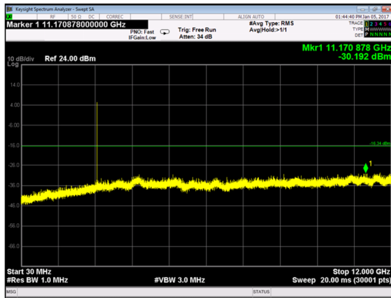
Plot 9-55. Conducted Spurious Emissions 30-12000 MHz: 3-DH5 Mode (Ch. 78)
