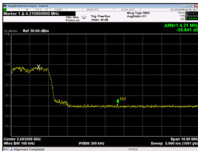
Plot 9-38. High Channel Band 3-DH5 Mode (Hopping enabled)
