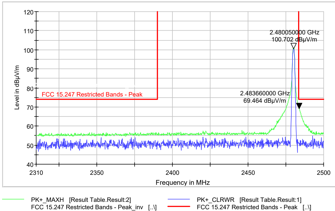
Plot 9-59. Restricted Band Edge 1-DH5 Mode- Ch. 78 (2483.5-2500MHz) – Peak
