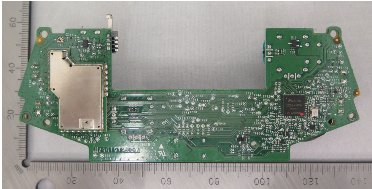
Main Board- Top View
