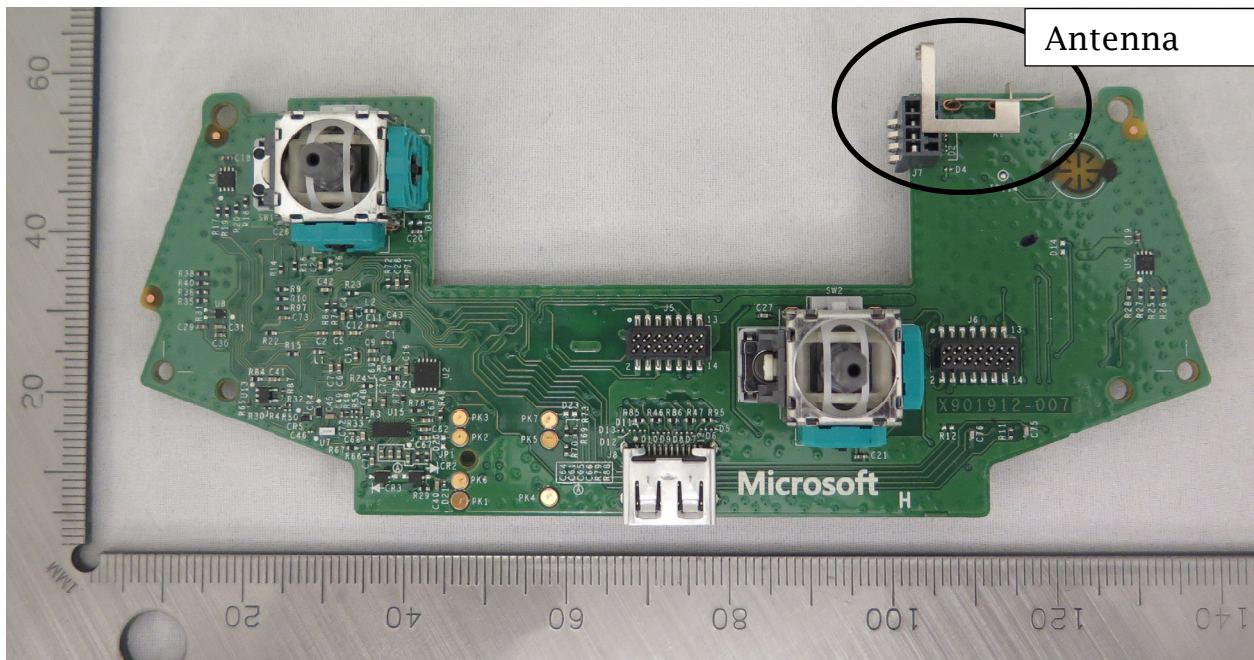
Main Board- Back View.
