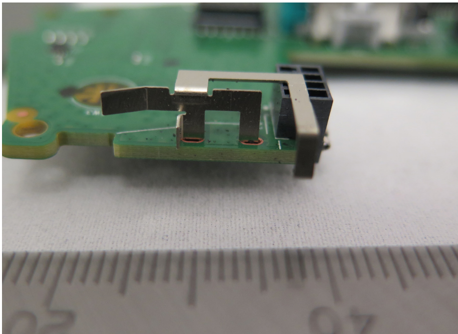
Antenna Photographs
