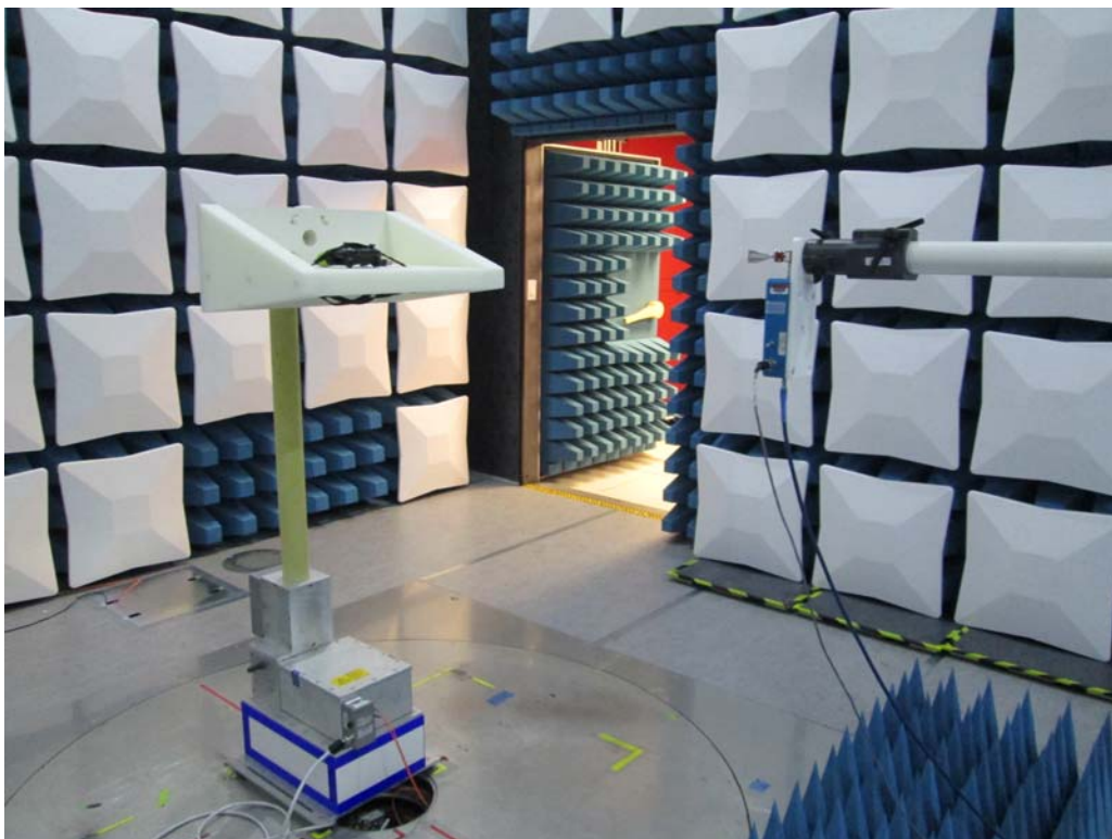
Fig.5 Radiated Spurious Emissions (26.5 -40 GHz)
