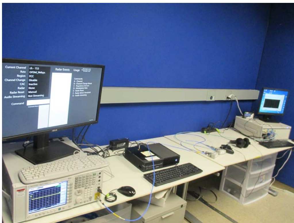
Fig.7 DFS Test Setup 1
