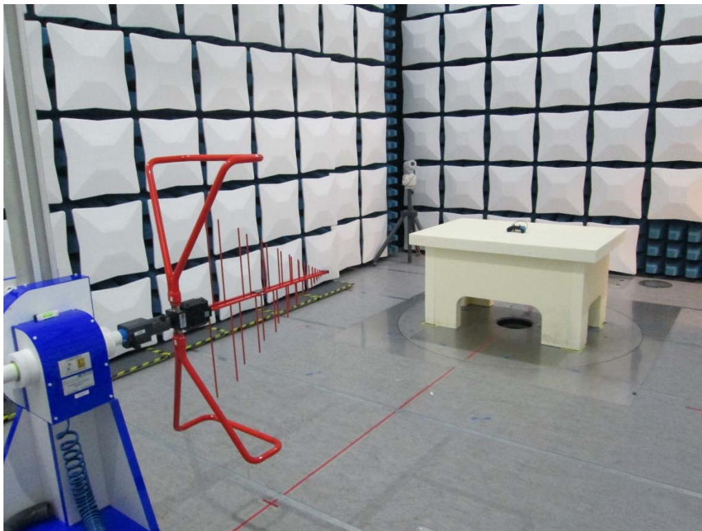
Fig.1 Radiated Spurious Emissions Test Setup (30MHz – 1GHz)
