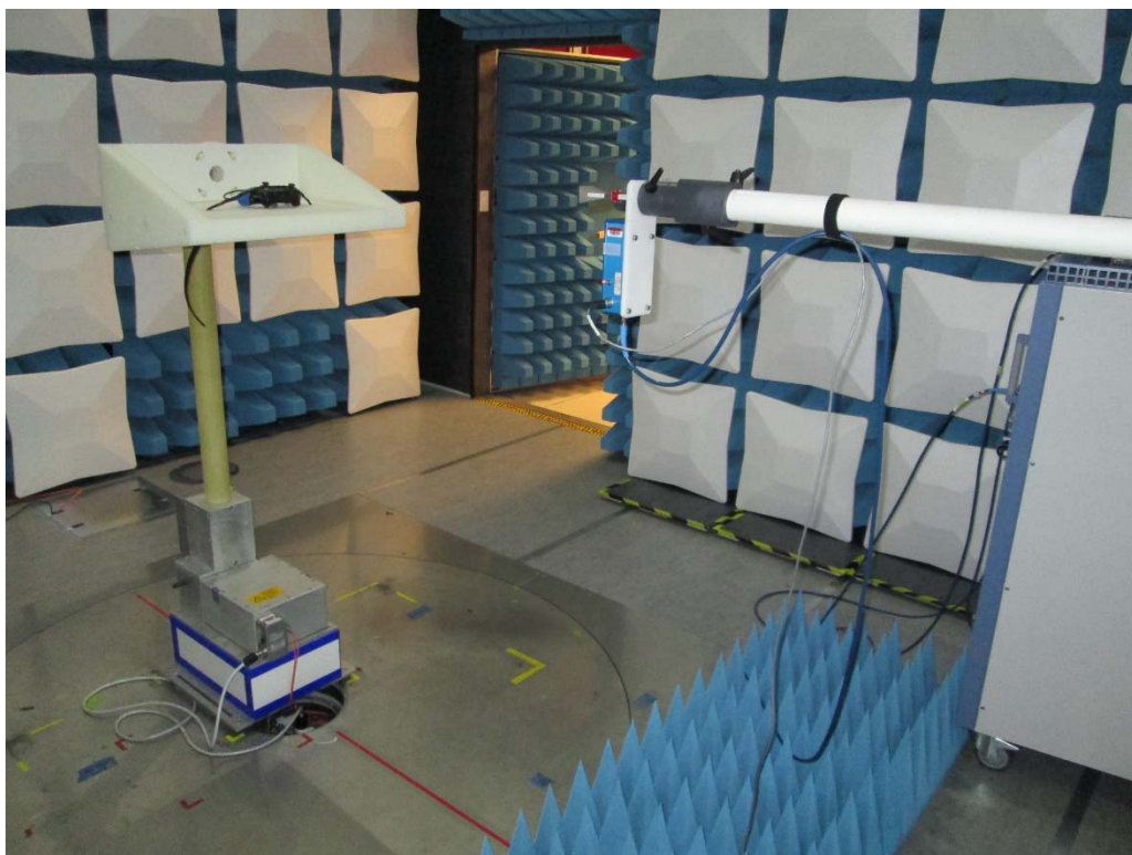
Fig.4 Radiated Spurious Emissions (18-26.5GHz)
