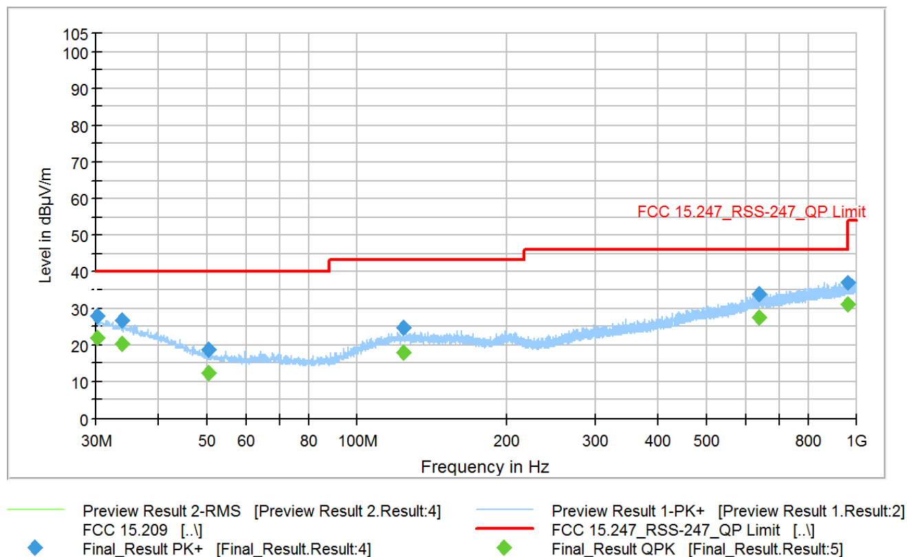
Figure 9-29 Radiated Spurious Emissions (Ch. 39) 2480 (30MHz - 1GHz)
