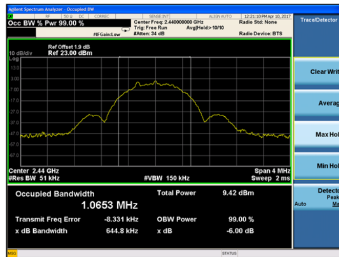
Figure 9-6 99% Bandwidth (Ch. 19)
