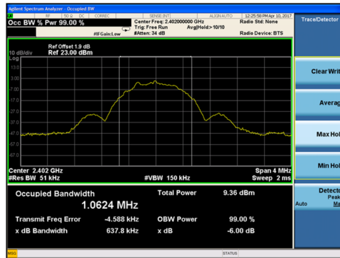
Figure 9-5 99% Bandwidth (Ch. 0)
