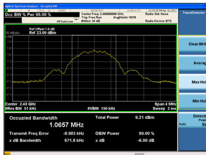
Figure 9-7 99% Bandwidth (Ch. 39)
