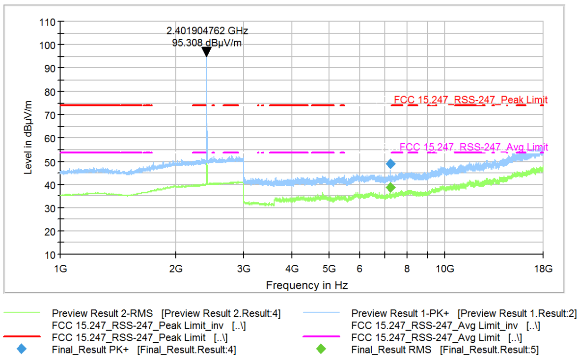
Figure 9-30 Radiated Spurious Emissions 1-18 GHz (Ch. 0)
