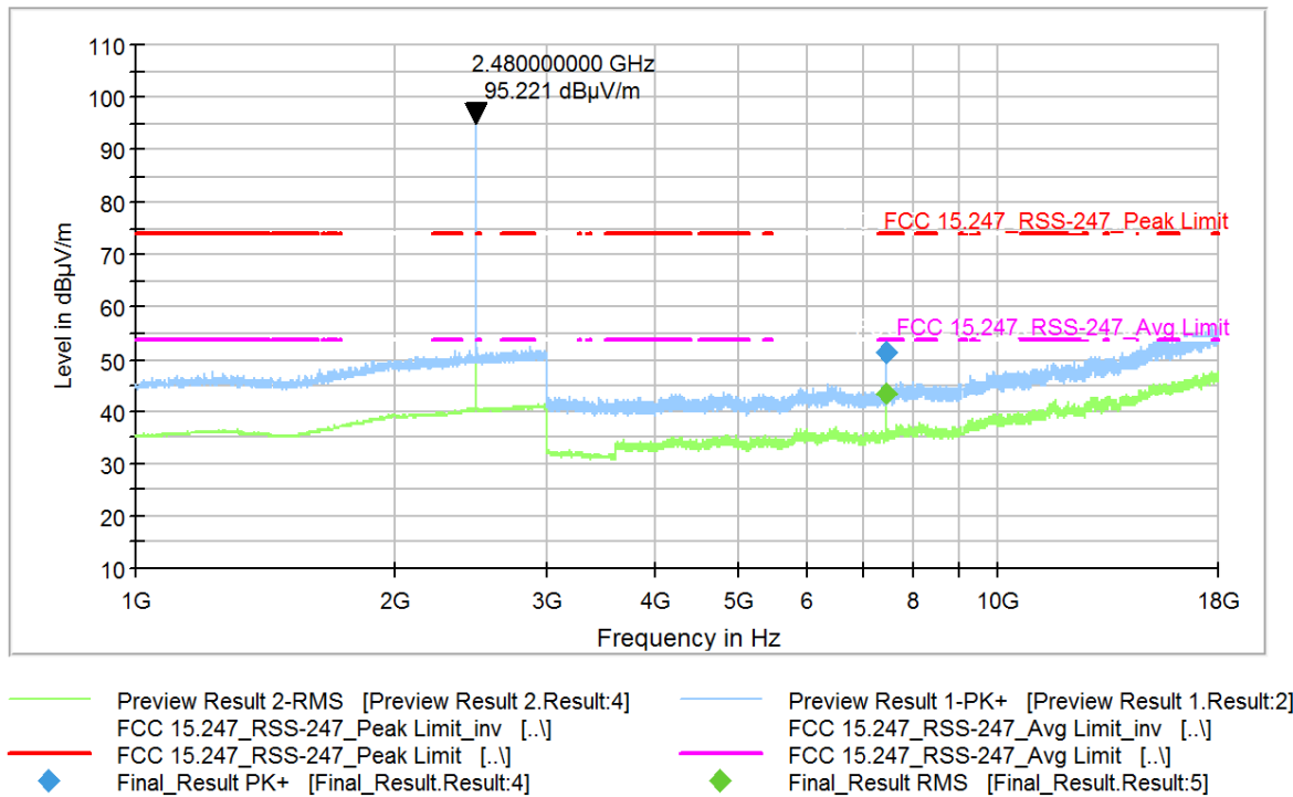
Figure 9-32 Radiated Spurious Emissions 1-18 GHz (Ch. 39)
