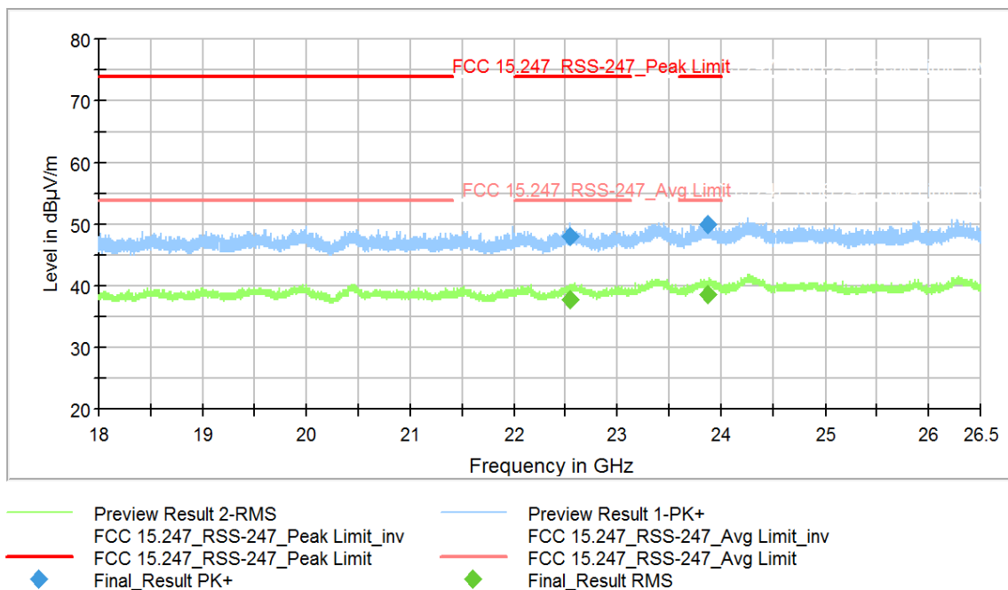
Figure 9-33 Radiated Spurious Emissions (Ch. 39) (18 – 26.5 GHz)
