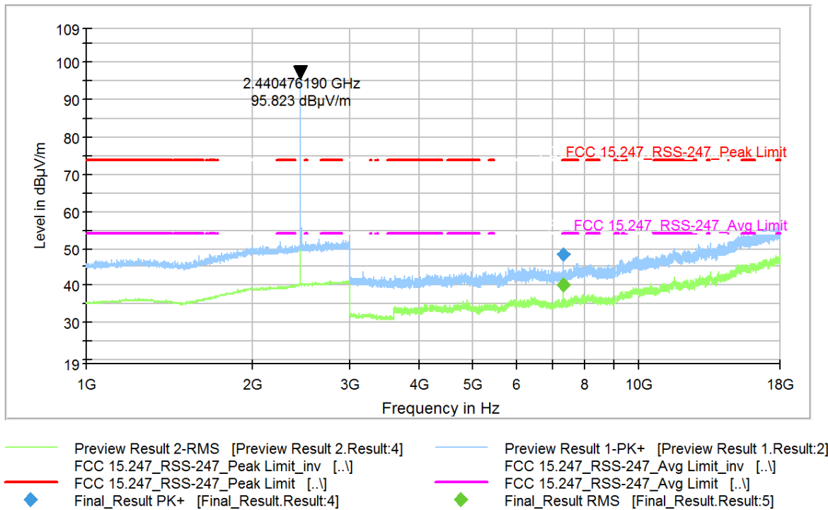
Figure 9-31 Radiated Spurious Emissions 1-18 GHz (Ch. 19)
