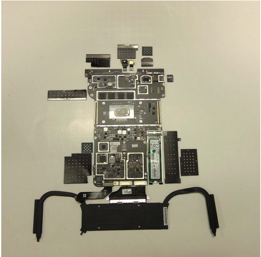
Motherboard top side with shield cans removed
