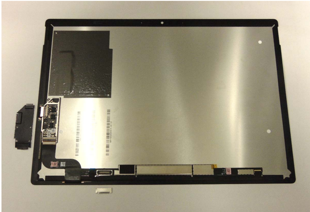
Display with shield cans removed
