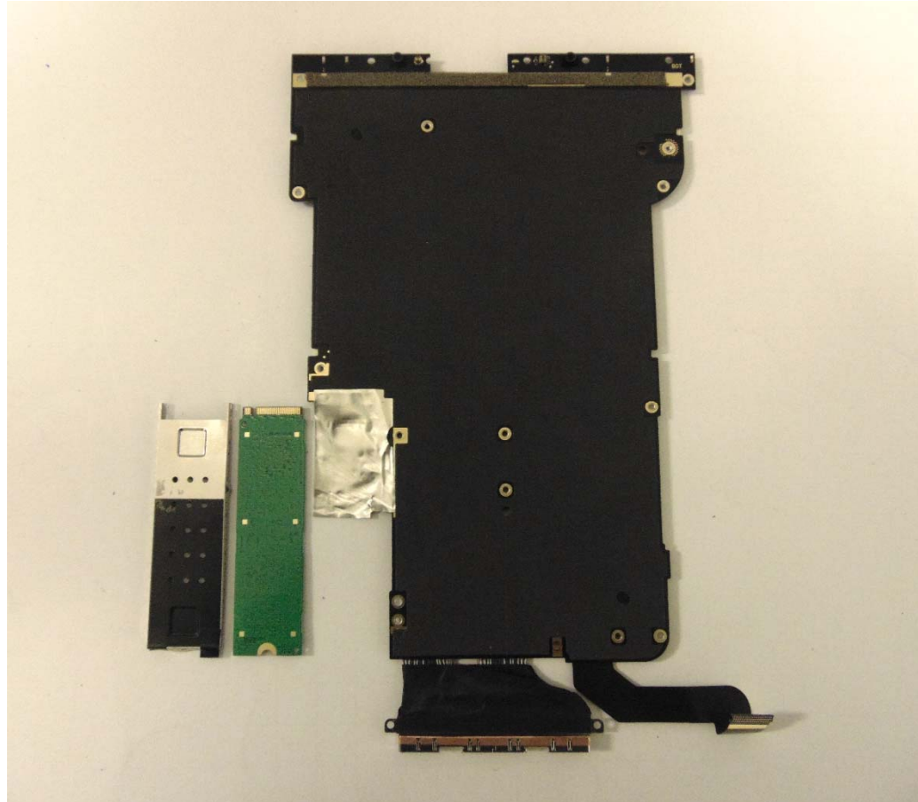
Motherboard bottom side with shield cans removed
