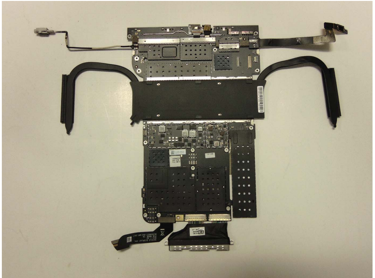
Motherboard top side with shield cans
