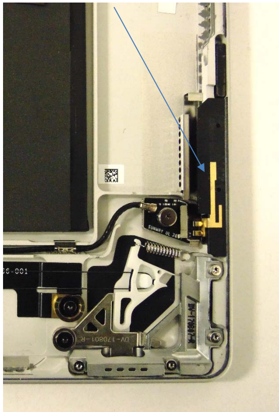
Accessory Radio antenna
