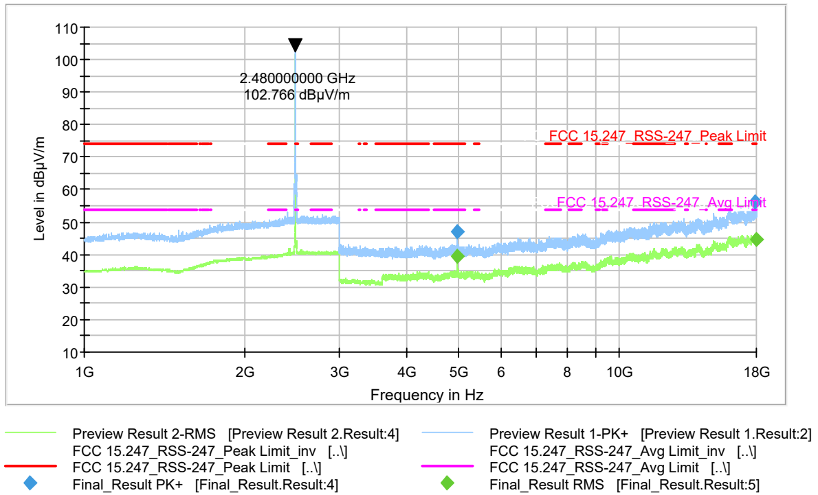
Figure 9-73 Radiated Spurious Emissions (Ch. 78) 1-DH5 (1-18 GHz)
