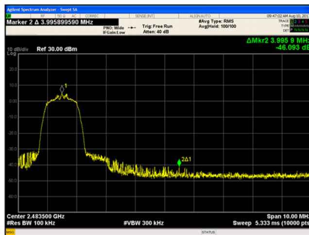
Figure 9-33 High Channel Band edge: 2-DH5 Mode (Hopping disabled)
