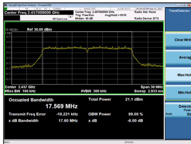
Plot 9-21 Chain A DTS Bandwidth 802.11n mode - Ch.10 (2457 MHz)
