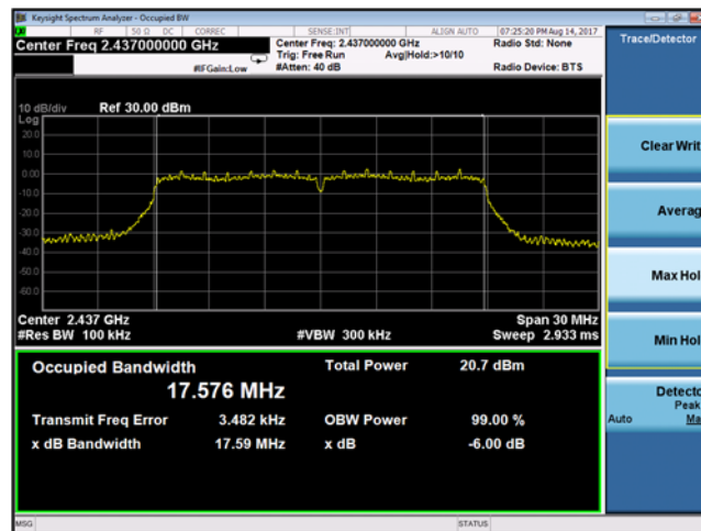
Plot 9-38 Chain B DTS Bandwidth 802.11n mode - Ch.6 (2437 MHz)
