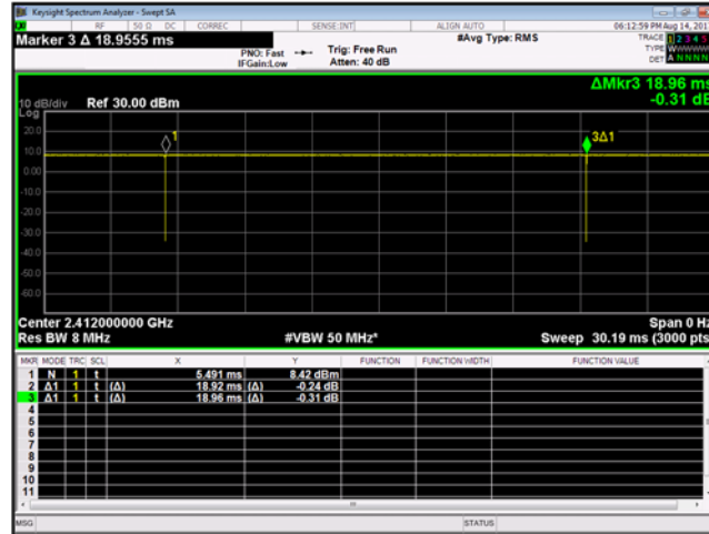
Figure 9-1. Duty Cycle 802.11b -Path A
