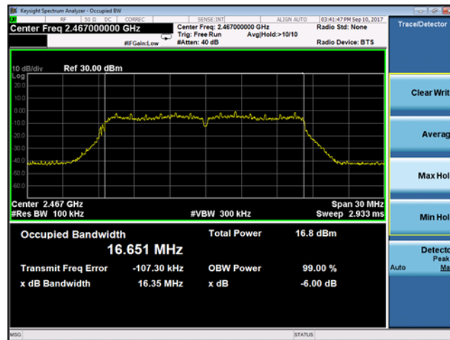
Plot 9-35 Chain B DTS Bandwidth 802.11g mode - Ch.12 (2467 MHz)
