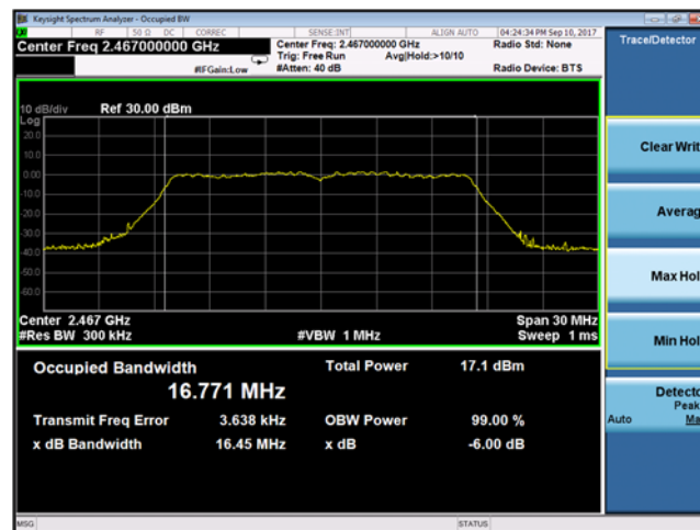
Plot 9-53 Chain A 99% Bandwidth 802.11g - Ch.12 (2467 MHz)
