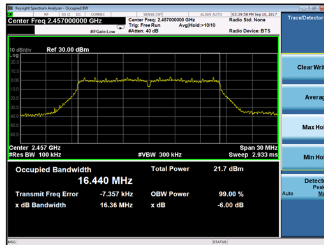
Plot 9-33 Chain B DTS Bandwidth 802.11g mode - Ch.10 (2457 MHz)
