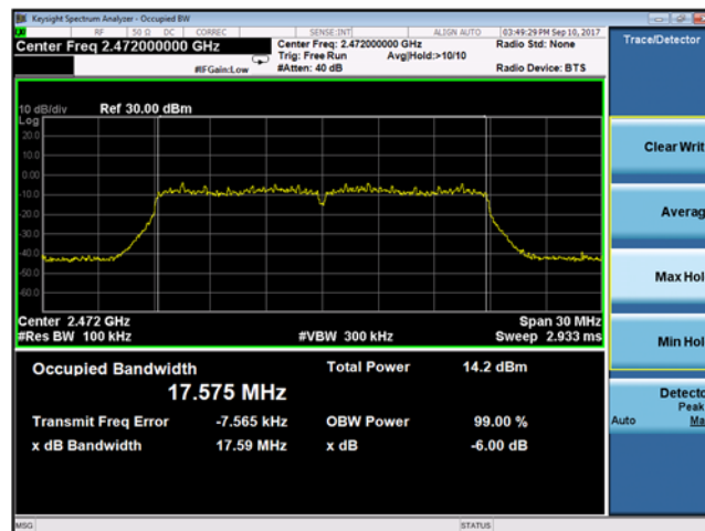
Plot 9-42 Chain B DTS Bandwidth 802.11n mode - Ch.13 (2472 MHz)
