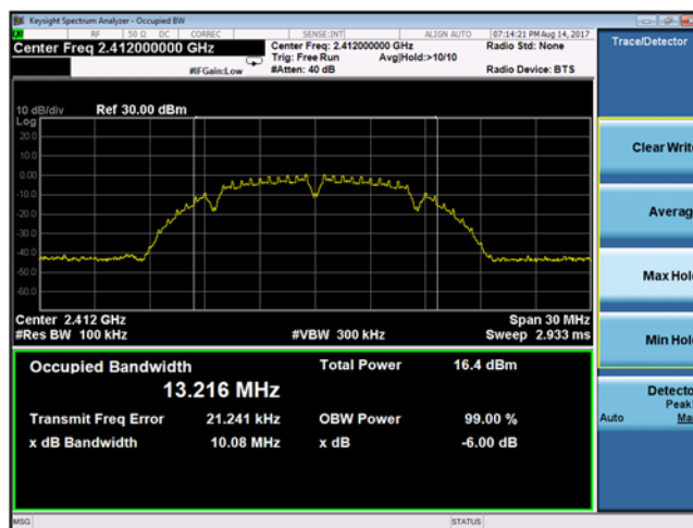
Plot 9-7 Chain A DTS Bandwidth 802.11b mode - Ch.1 (2412 MHz)
