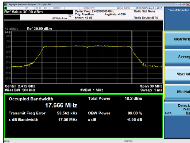
Plot 9-55 Chain A 99% Bandwidth 802.11n - Ch.1 (2412 MHz)
