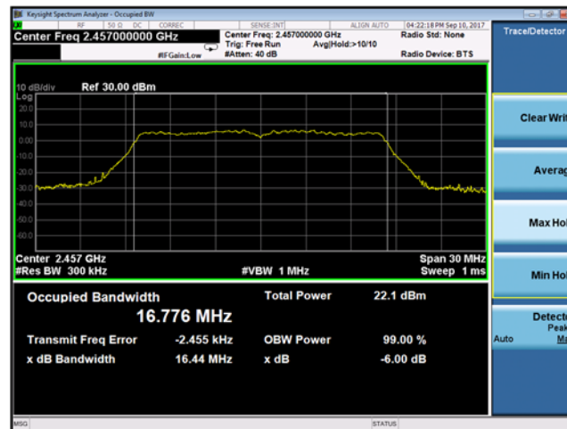
Plot 9-51 Chain A 99% Bandwidth 802.11g - Ch.10 (2457 MHz)
