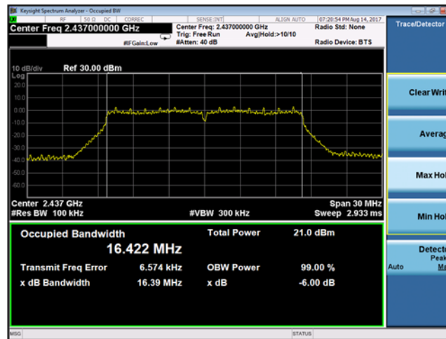
Plot 9-32 Chain B DTS Bandwidth 802.11g mode - Ch.6 (2437 MHz)
