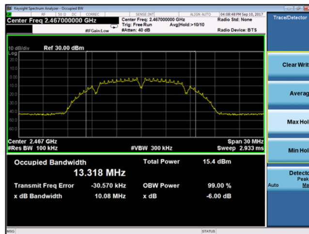
Plot 9-11 Chain A DTS Bandwidth 802.11b mode - Ch.12 (2467 MHz)
