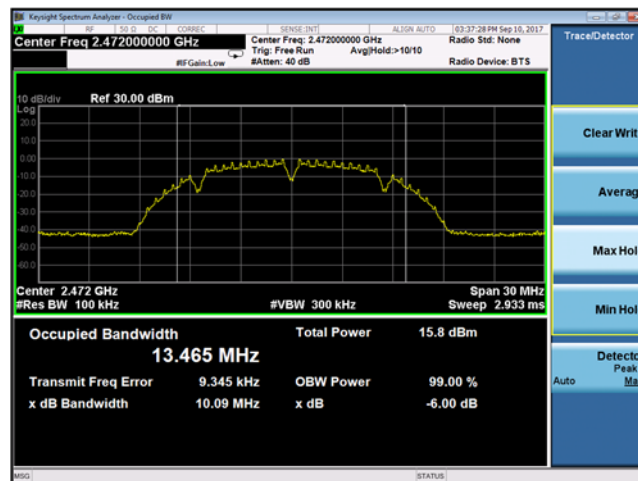
Plot 9-30 Chain B DTS Bandwidth 802.11b mode - Ch.13 (2472 MHz)
