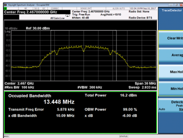
Plot 9-29 Chain B DTS Bandwidth 802.11b mode - Ch.12 (2467 MHz)
