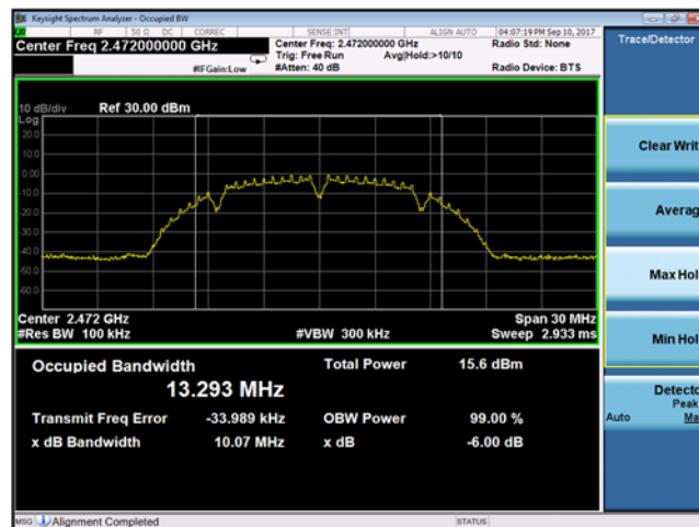
Plot 9-12 Chain A DTS Bandwidth 802.11b mode - Ch.13 (2472 MHz)
