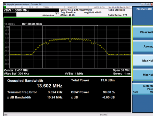
Plot 9-45 Chain A 99% Bandwidth 802.11b - Ch.10 (2457 MHz)
