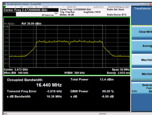
Plot 9-36 Chain B DTS Bandwidth 802.11g mode - Ch.13 (2472 MHz)
