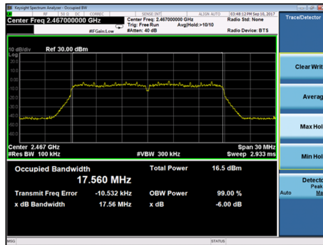
Plot 9-41 Chain B DTS Bandwidth 802.11n mode - Ch.12 (2467 MHz)
