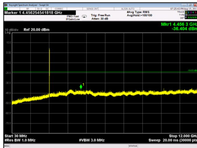
Plot 9-119 Chain A Conducted Spurious Emissions 30 MHz - 12 GHz 802.11b - Ch.6 (2437 MHz)
