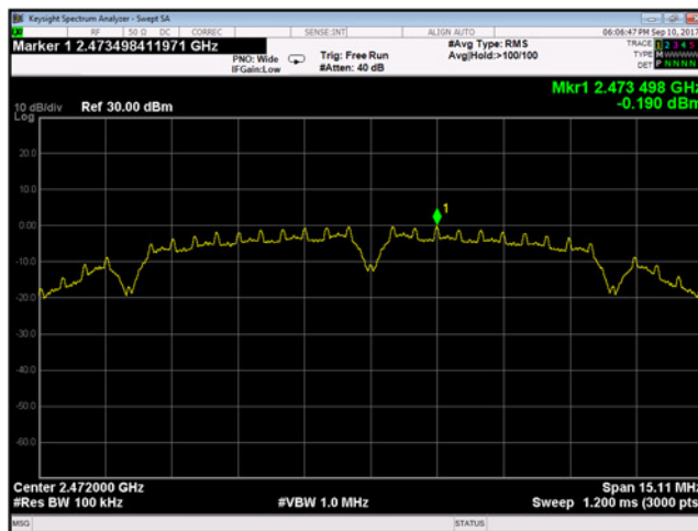
Plot 9-84 Chain A Peak Power Spectral Density 802.11b - Ch.13 (2472 MHz)
