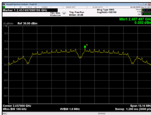
Plot 9-99 Chain B Peak Power Spectral Density 802.11b - Ch.10 (2457 MHz)
