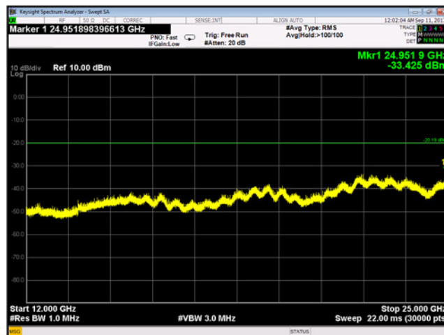
Plot 9-129 Chain A Conducted Spurious Emissions 12 - 25 GHz 802.11b - Ch.13 (2472 MHz)
