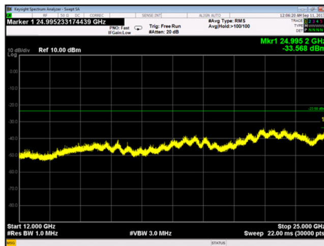
Plot 9-144 Chain A Conducted Spurious Emissions 12 - 25 GHz 802.11g - Ch.13 (2472 MHz)
