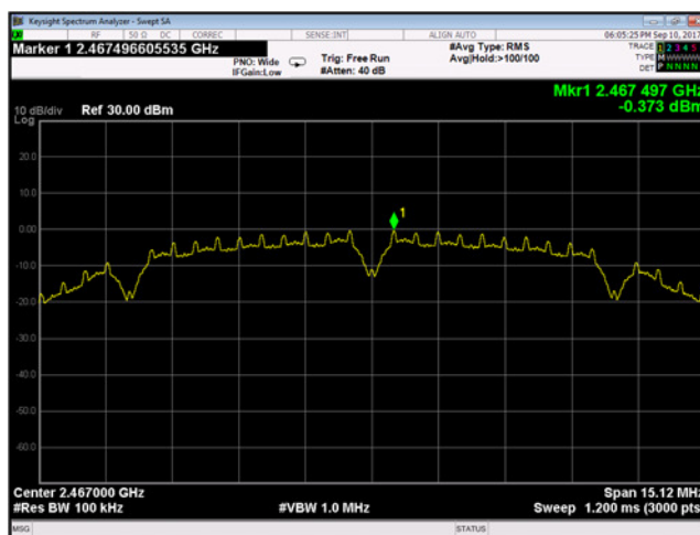
Plot 9-83 Chain A Peak Power Spectral Density 802.11b - Ch.12 (2467 MHz)
