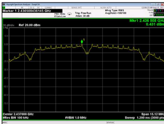
Plot 9-98 Chain B Peak Power Spectral Density 802.11b - Ch.6 (2437 MHz)
