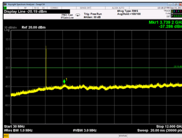
Plot 9-128 Chain A Conducted Spurious Emissions 30 MHz - 12 GHz 802.11b - Ch.13 (2472 MHz)
