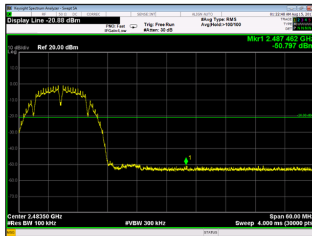
Plot 9-218 Chain B Conducted Band Edge 802.11b - Ch. 11 (2462 MHz)
