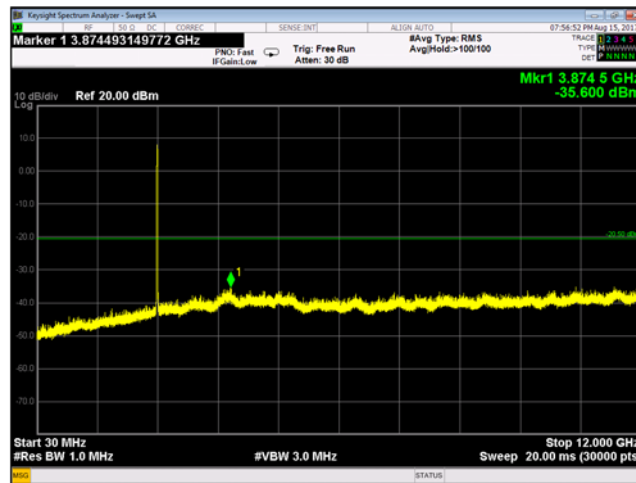
Plot 9-176 Chain B Conducted Spurious Emissions 30 MHz - 12 GHz 802.11g - Ch.1 (2412 MHz)
