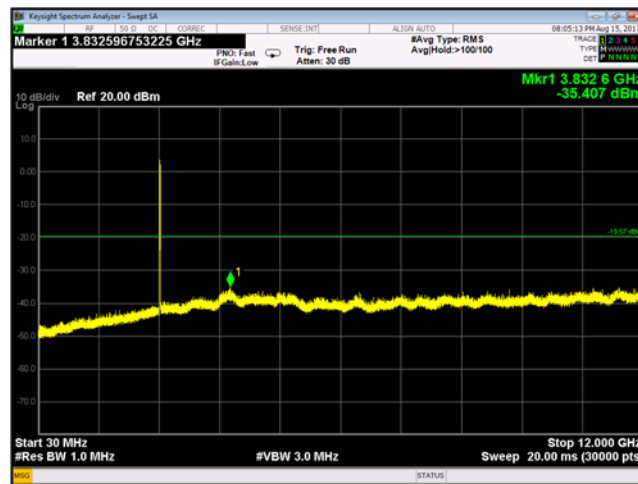
Plot 9-164 Chain B Conducted Spurious Emissions 30 MHz - 12 GHz 802.11b - Ch.6 (2437 MHz)
