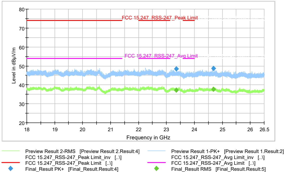
Figure 9-324 Radiated Spurious Emissions (Ch. 39) (18 – 26.5 GHz)
