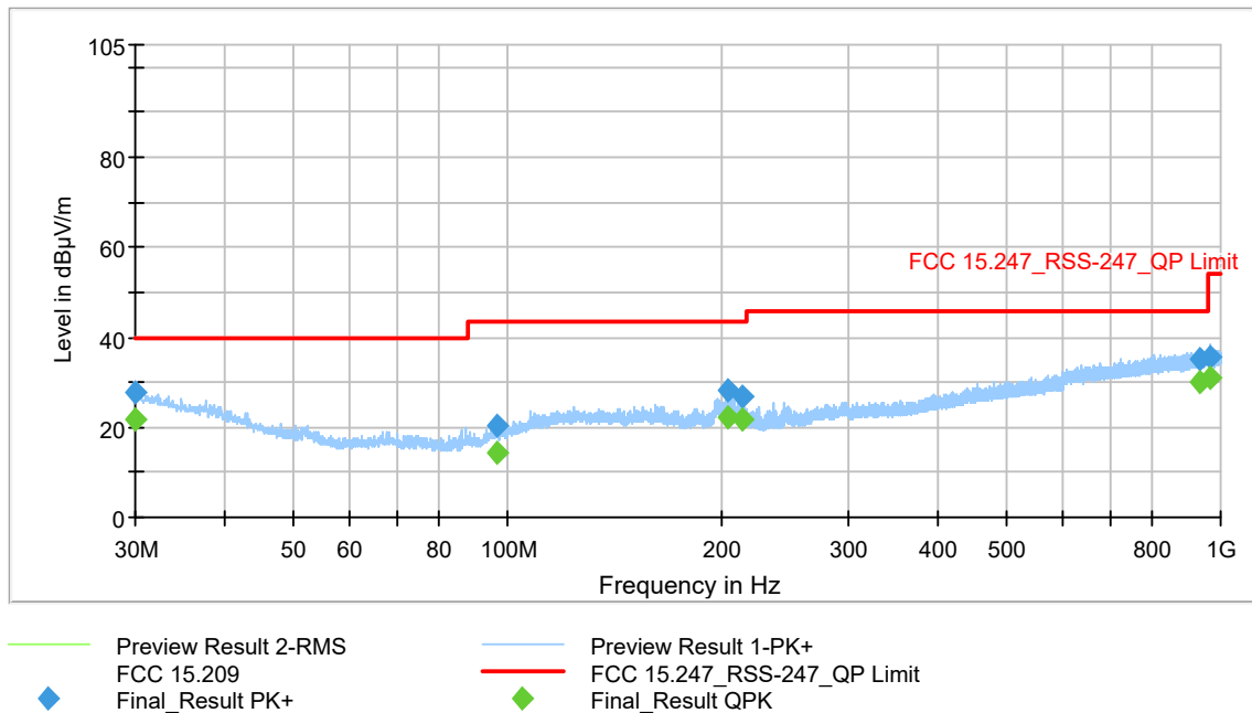
Figure 9-30 Radiated Spurious Emissions (Ch. 39) 2480 (30MHz - 1GHz)
