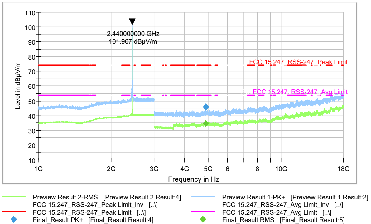
Figure 9-302 Radiated Spurious Emissions 1-18 GHz (Ch. 19)
