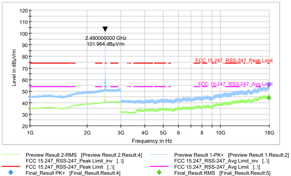
Figure 9-313 Radiated Spurious Emissions 1-18 GHz (Ch. 39)
