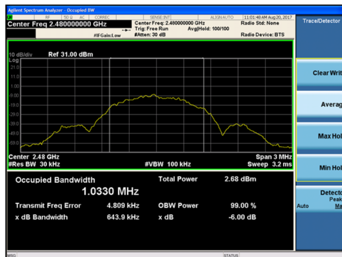
Figure 9-7 99% Bandwidth (Ch. 39)
