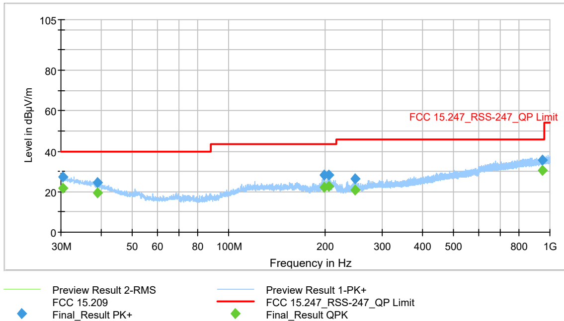
Figure 9-29 Radiated Spurious Emissions (Ch. 0) 2402 (30MHz - 1GHz)
