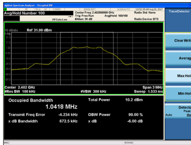
Figure 9-2 6dB Bandwidth (Ch. 0)
