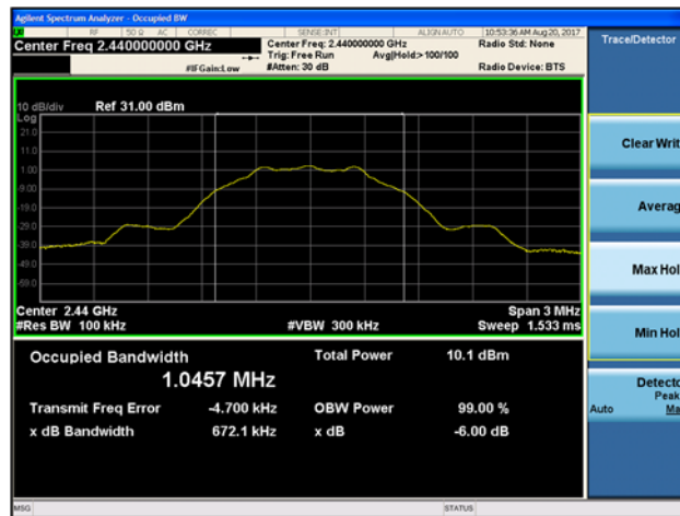
Figure 9-3 6dB Bandwidth (Ch. 19)
