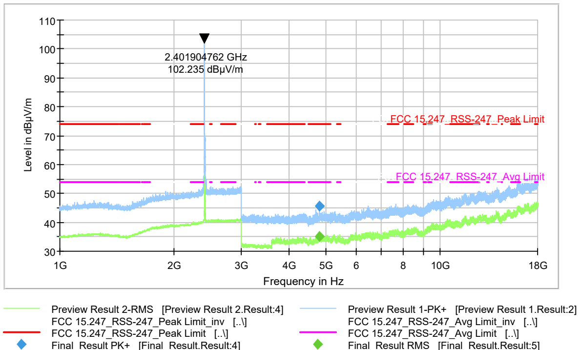
Figure 9-291 Radiated Spurious Emissions 1-18 GHz (Ch. 0)
