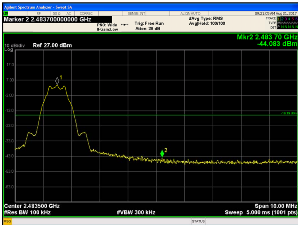
Figure 9-24 Conducted- High Band Edge (Ch. 39)
