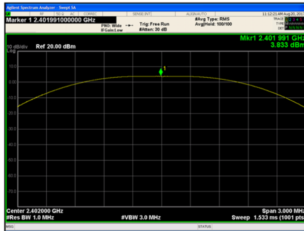
Figure 9-8 Peak Power (Ch. 0)
