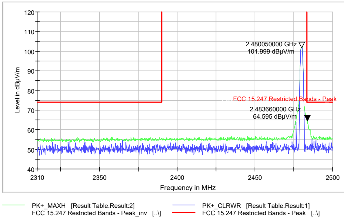
Figure 9-27 Radiated Restricted Band Edge (Ch. 39) Peak
