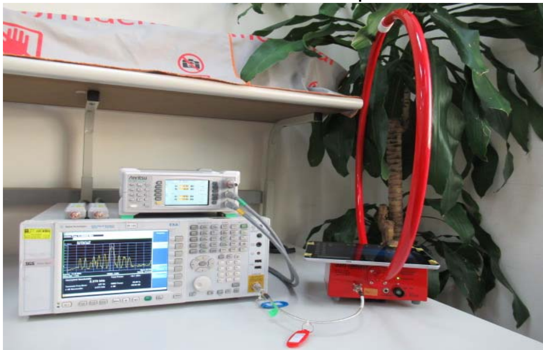
Frequency stability Setup Photo
