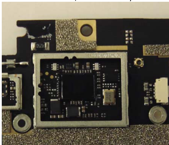
Wi-Fi/BT radio circuitry
