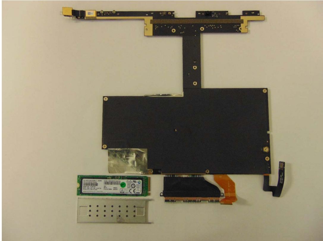
Motherboard bottom side with shield cans removed
