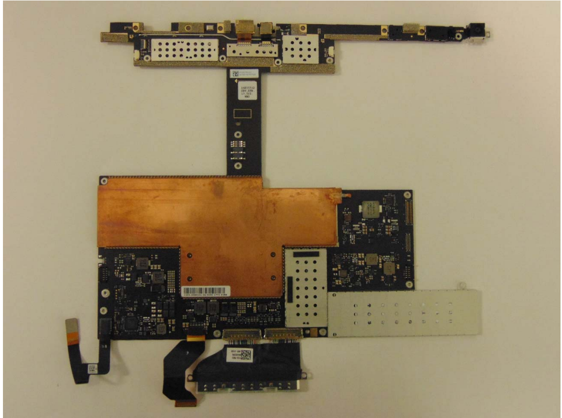
Motherboard top side with shield cans
