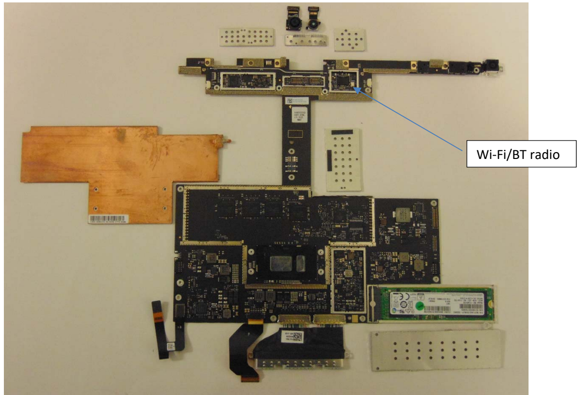
Motherboard top side with shield cans removed
