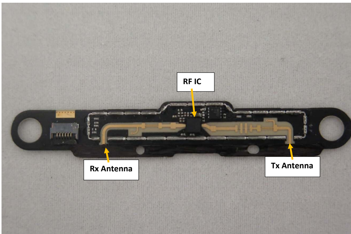
RF PCB
