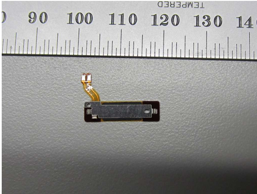
Coil FPC – View 1
