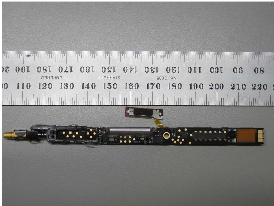
Main PCB – View 1
