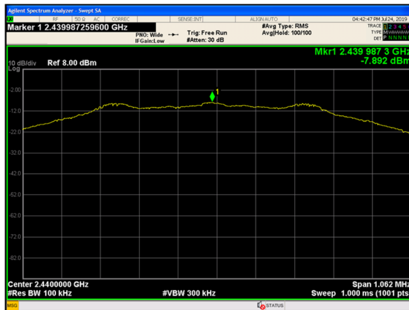
Figure 9-14 Power Spectral Density (Ch. 19)
