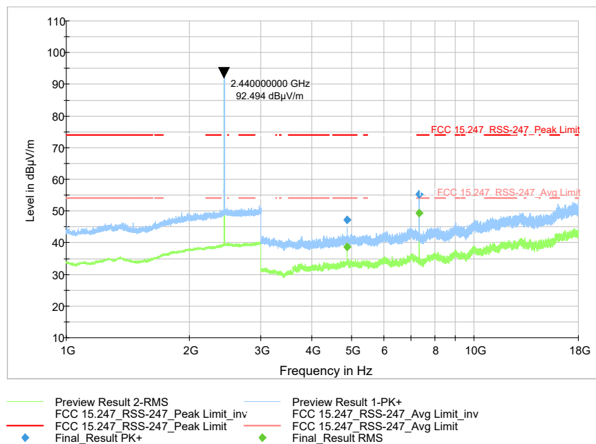
Figure 9-34 Radiated Spurious Emissions 1-18 GHz (Ch. 19)
