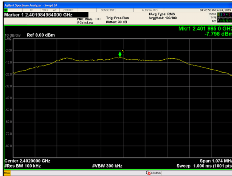
Figure 9-13 Power Spectral Density (Ch. 0)
