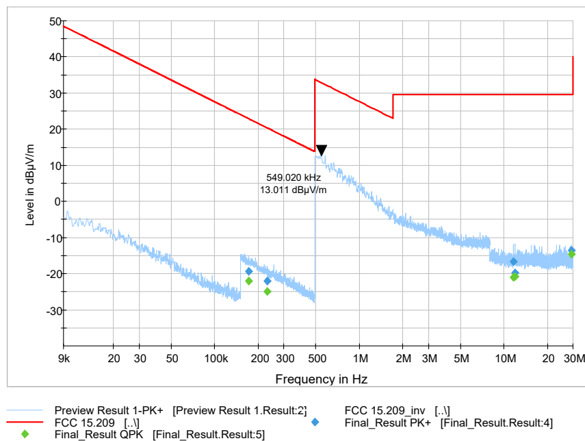
Figure 9-31 Radiated Spurious Emissions (Ch. 39) 2480 (9kHz – 30MHz)
