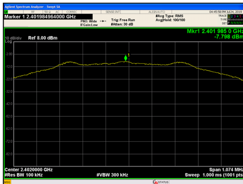
Figure 9-16 Reference Level Measurement (Ch.0)
