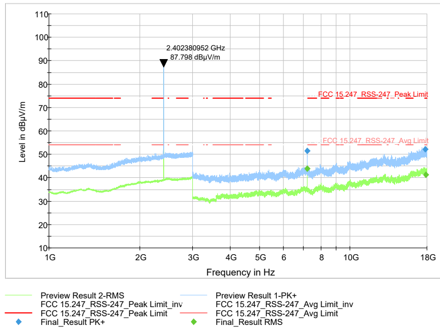
Figure 9-33 Radiated Spurious Emissions 1-18 GHz (Ch. 0)
