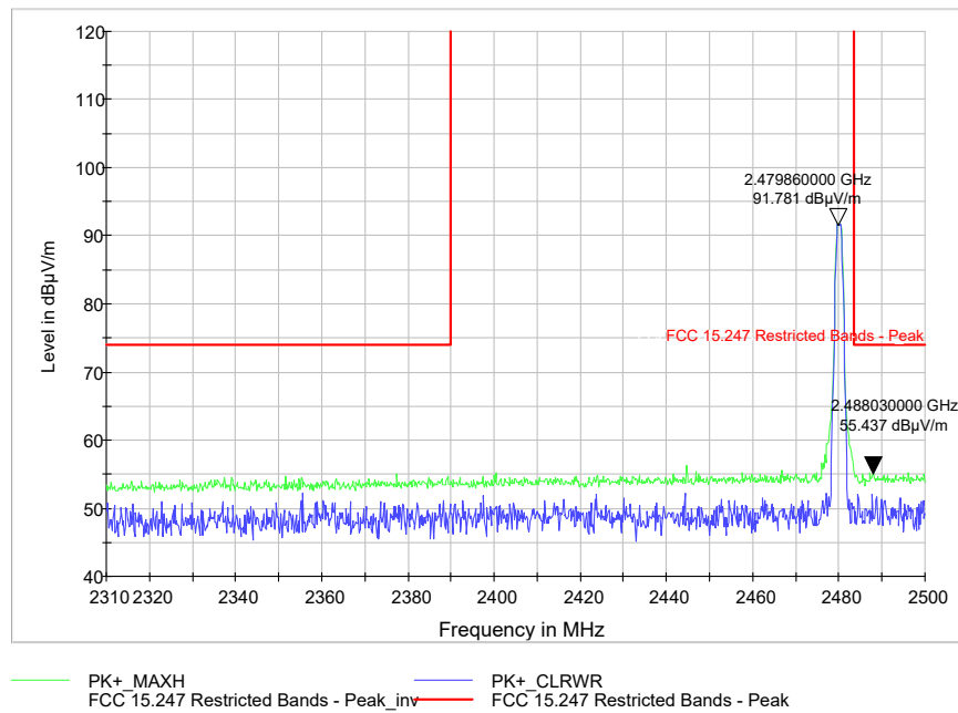
Figure 9-29 Radiated Restricted Band Edge (Ch. 39) Peak
