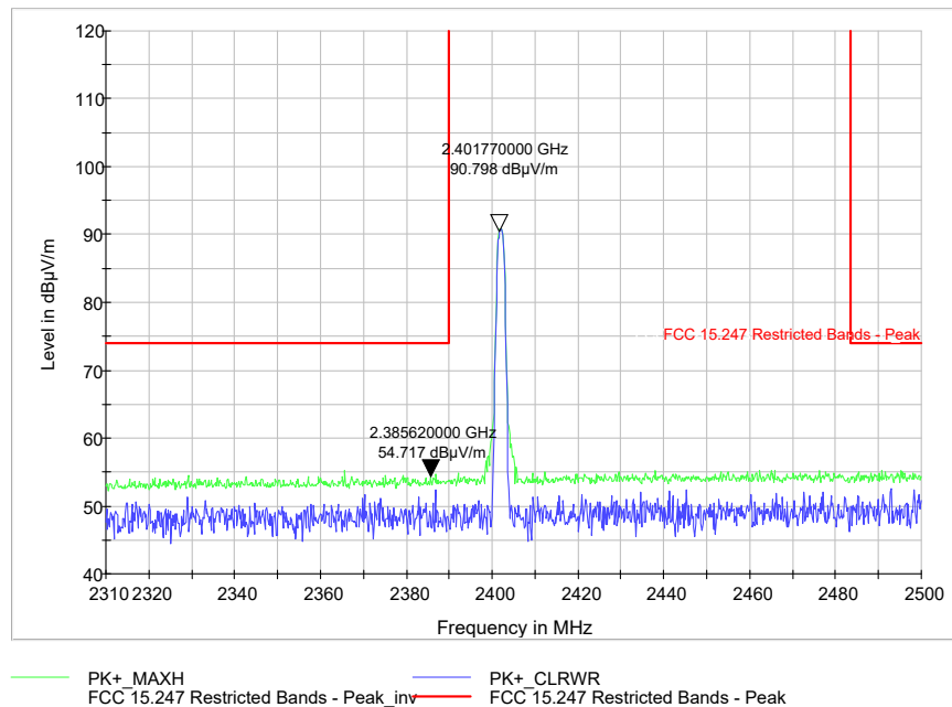
Figure 9-27 Radiated Restricted Band Edge (Ch. 0) Peak
