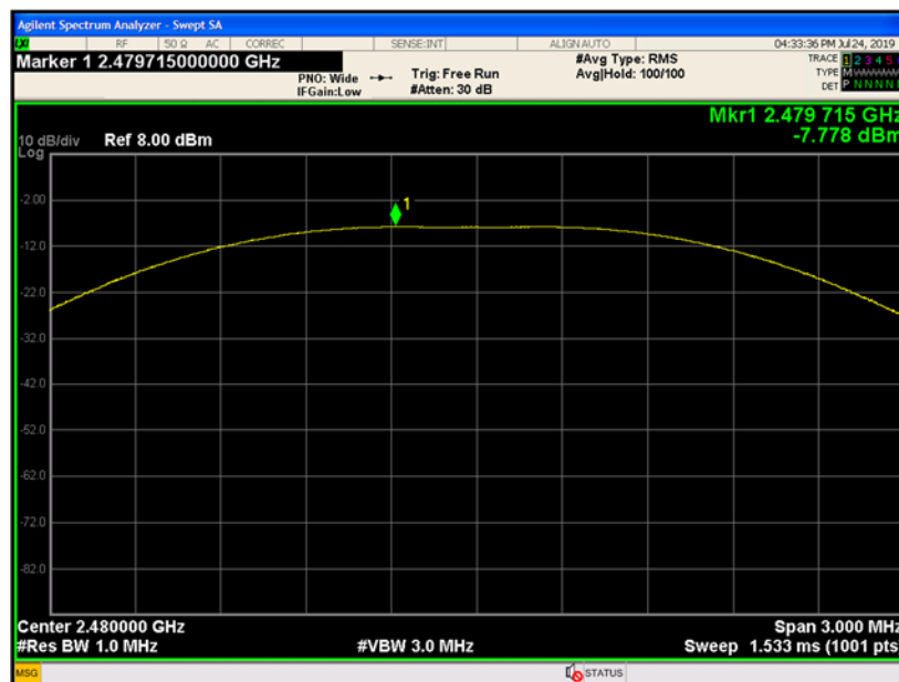
Figure 9-12 Peak Power (Ch. 39)
