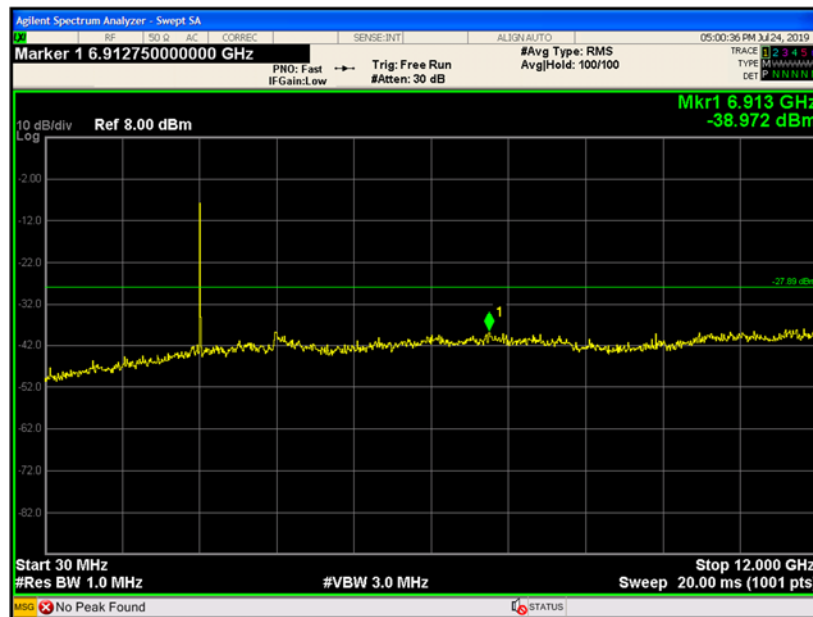
Figure 9-20 Conducted Spurious Emissions 30-12000 MHz (Ch. 19)
