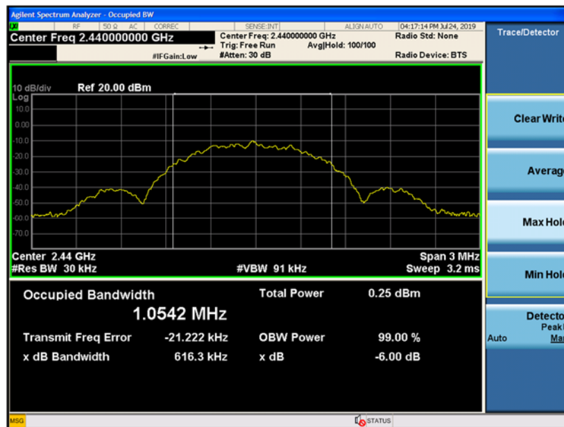
Figure 9-8 99% Bandwidth (Ch. 19)
