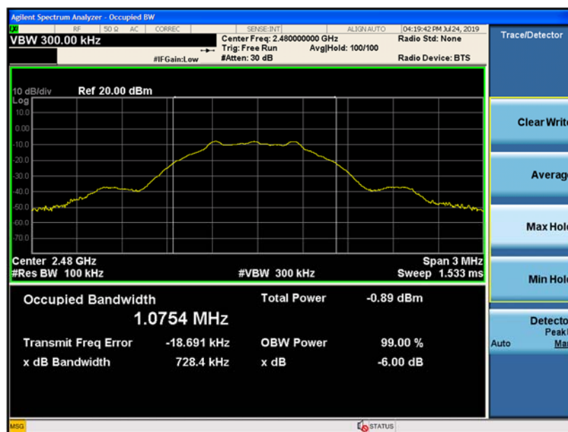
Figure 9-6 6dB Bandwidth (Ch. 39)
