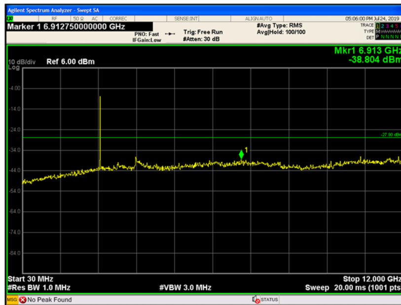
Figure 9-23 Conducted Spurious Emissions 30-12000 MHz (Ch.39)
