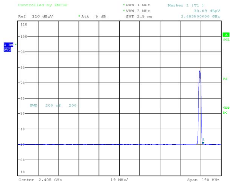
Figure 9-29 Radiated Restricted Band Edge (Ch. 39) Peak
