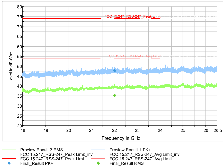
Figure 9-36 Radiated Spurious Emissions (Ch. 19) (18 – 26.5 GHz)
