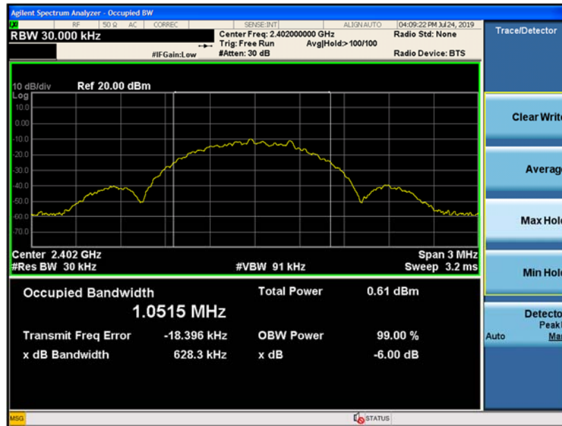
Figure 9-7 99% Bandwidth (Ch. 0)
