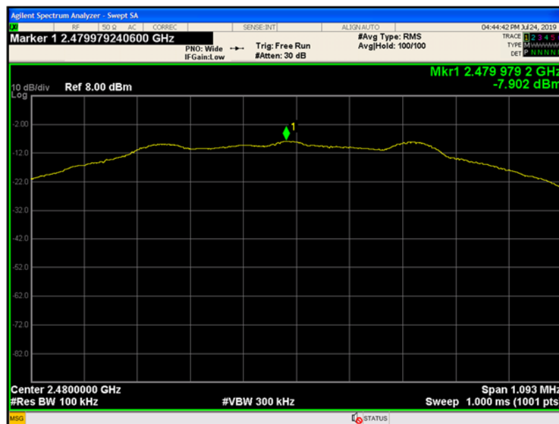
Figure 9-15 Power Spectral Density (Ch. 39)
