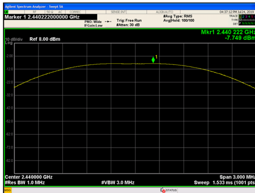
Figure 9-11 Peak Power (Ch. 19)
