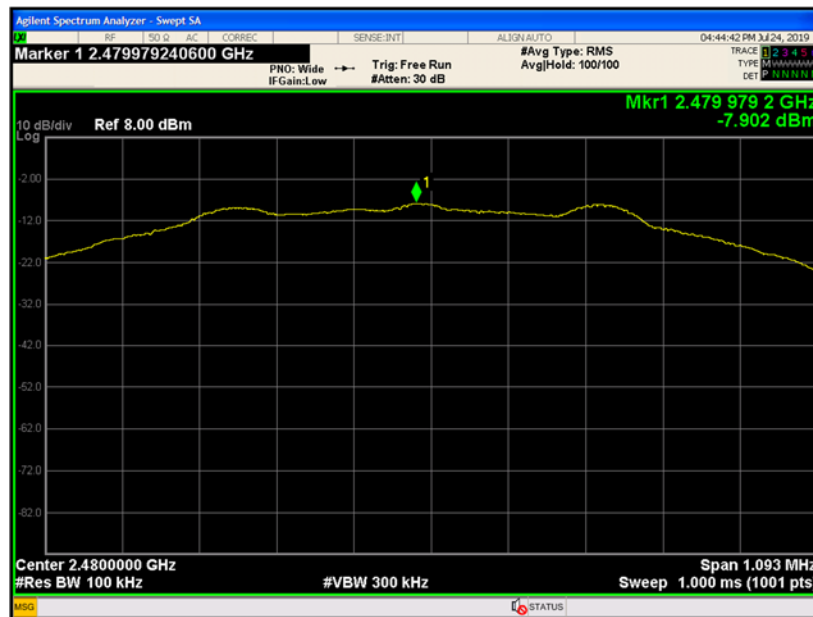
Figure 9-22 Reference Level Measurement (Ch.39)
