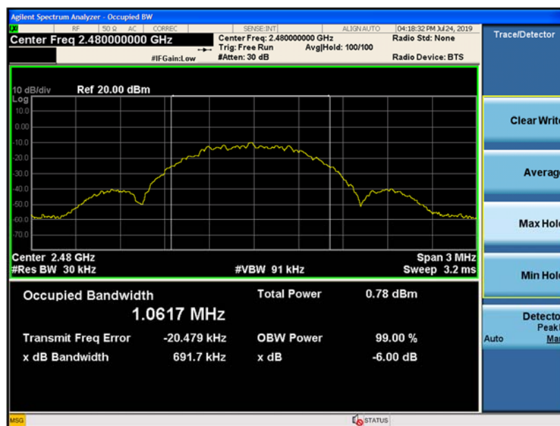
Figure 9-9 99% Bandwidth (Ch. 39)
