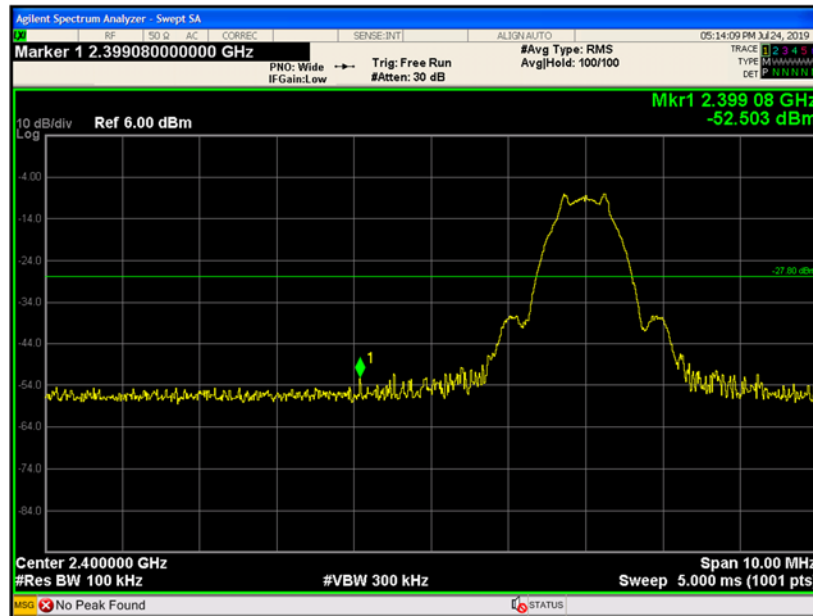
Figure 9-25 Conducted-Low Band Edge (Ch. 0)
