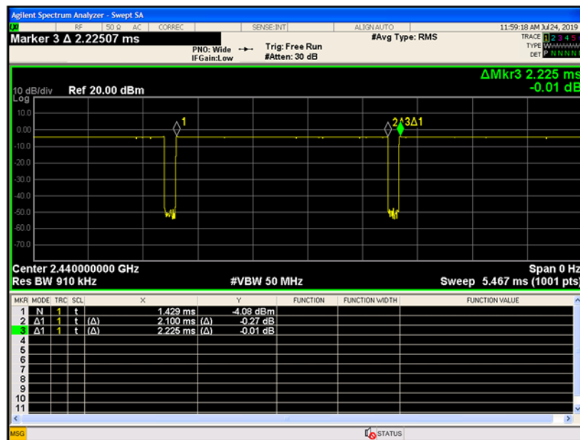
Figure 9-2 Duty Cycle 2440MHz (Ch.19)
