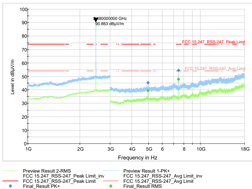
Figure 9-35 Radiated Spurious Emissions 1-18 GHz (Ch. 39)
