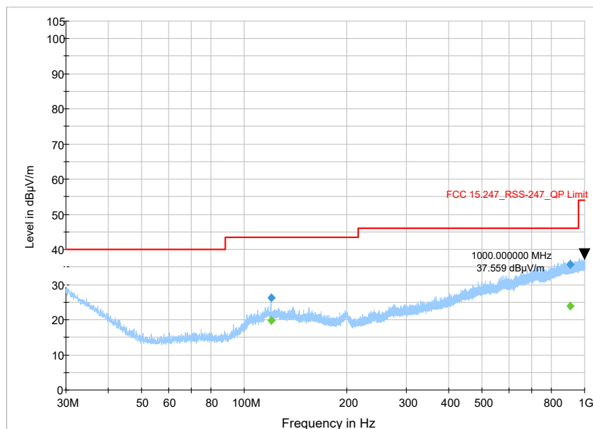
Figure 9-32 Radiated Spurious Emissions (Ch. 19) 2440 (30MHz - 1GHz)
