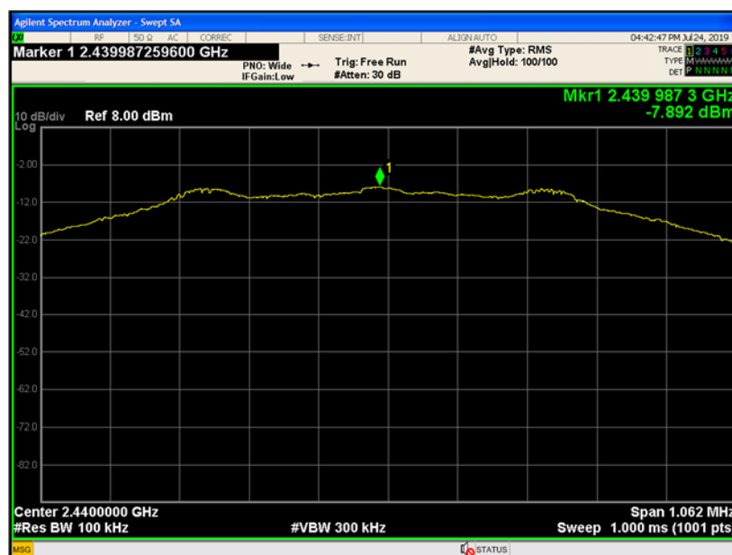
Figure 9-19 Reference Level Measurement (Ch.19)
