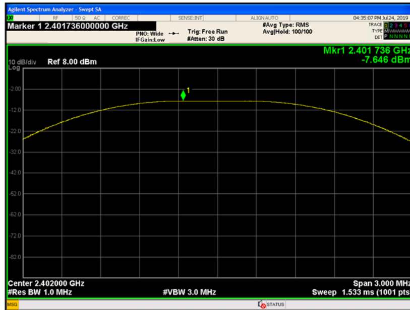
Figure 9-10 Peak Power (Ch. 0)
