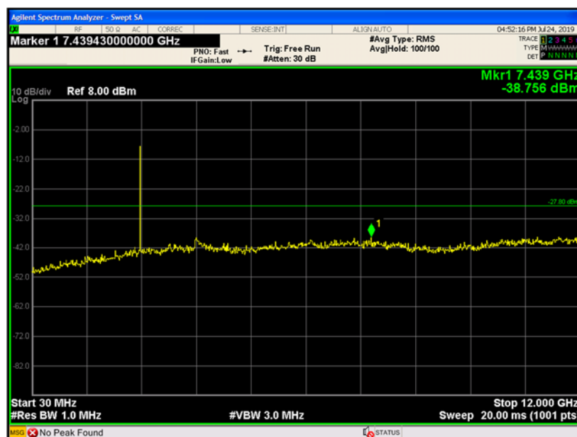
Figure 9-17 Conducted Spurious Emissions 30-12000 MHz (Ch. 0)
