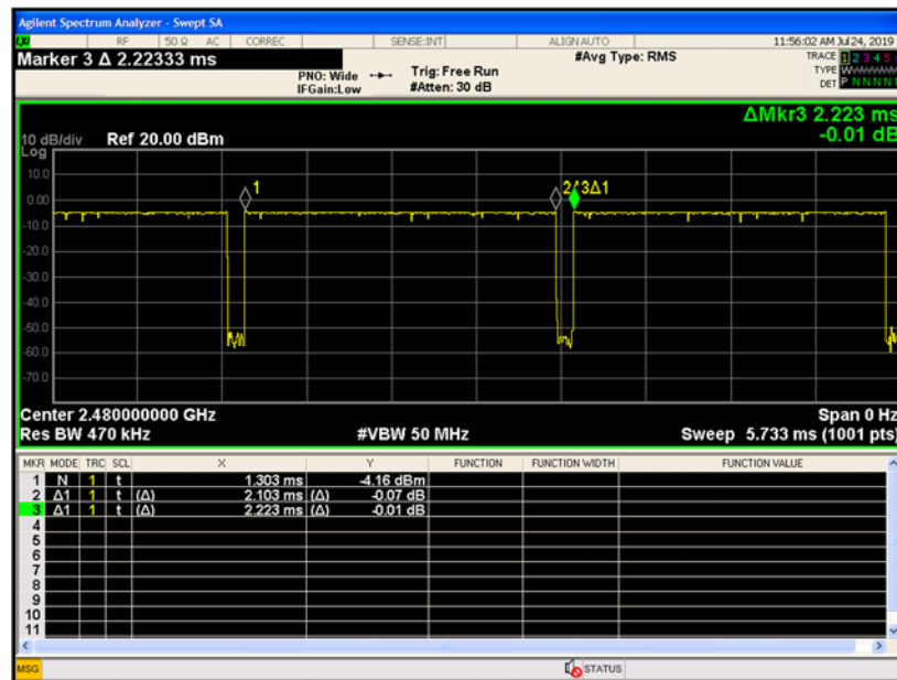
Figure 9-3 Duty Cycle 2480MHz (Ch.39)
