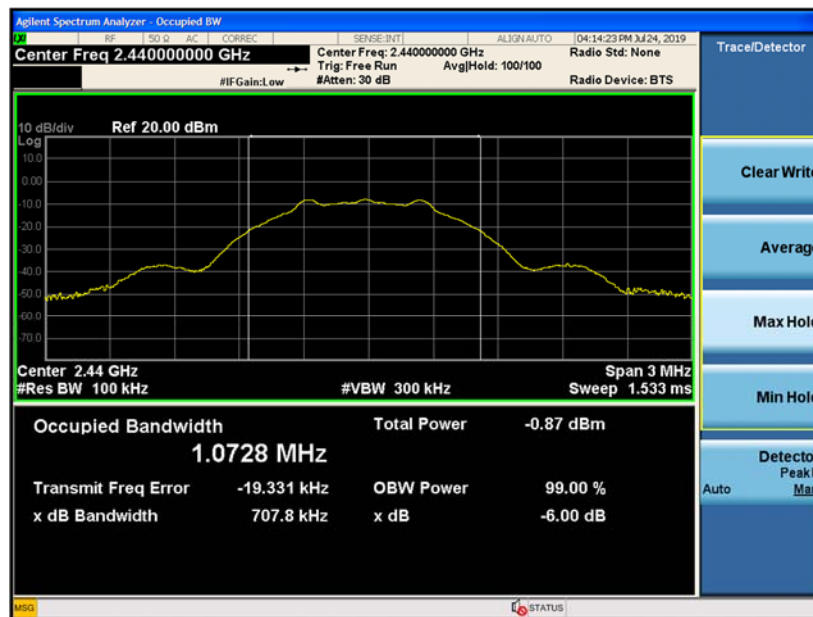
Figure 9-5 6dB Bandwidth (Ch. 19)
