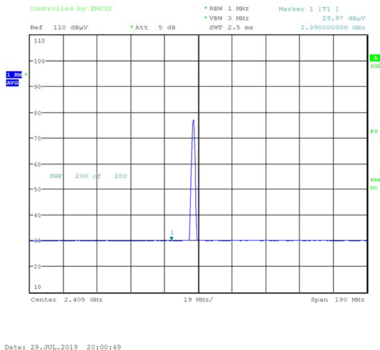
Figure 9-28 Radiated Restricted Band Edge (Ch. 0) Average
