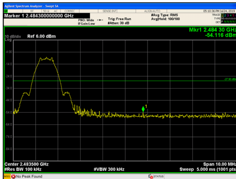
Figure 9-26 Conducted- High Band Edge (Ch. 39)
