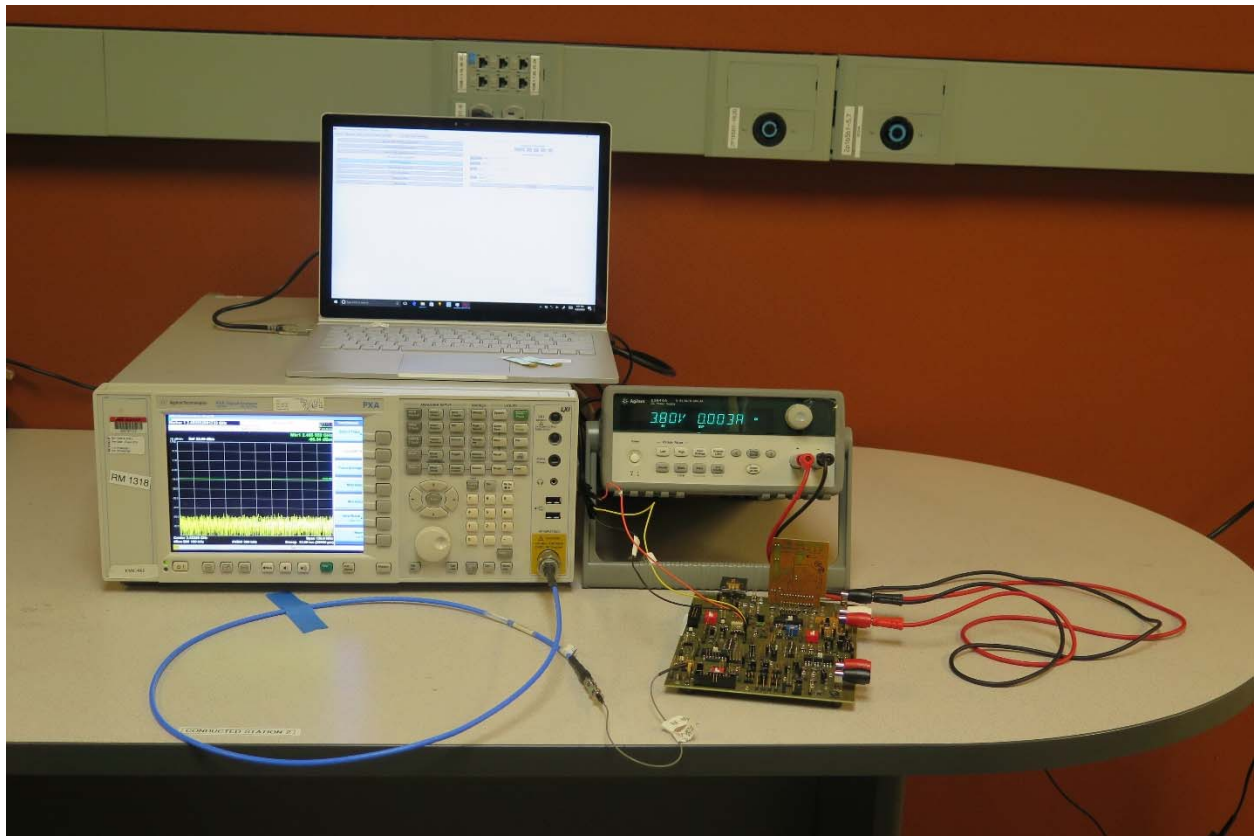
Figure 5 Conducted Test Setup
