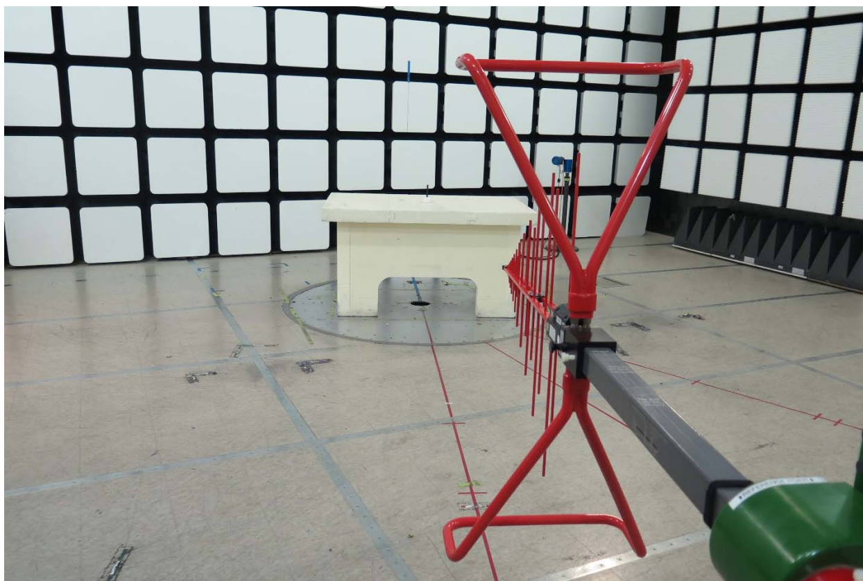
Figure 2 Radiated Spurious Emissions Test Setup (30M-1GHz)
