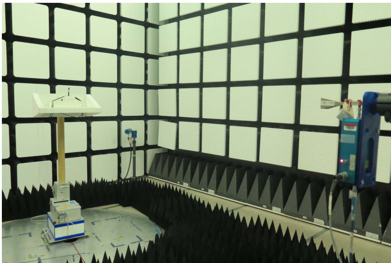
Figure 4 Radiated Spurious Emissions Test Setup (18-26.5GHz)
