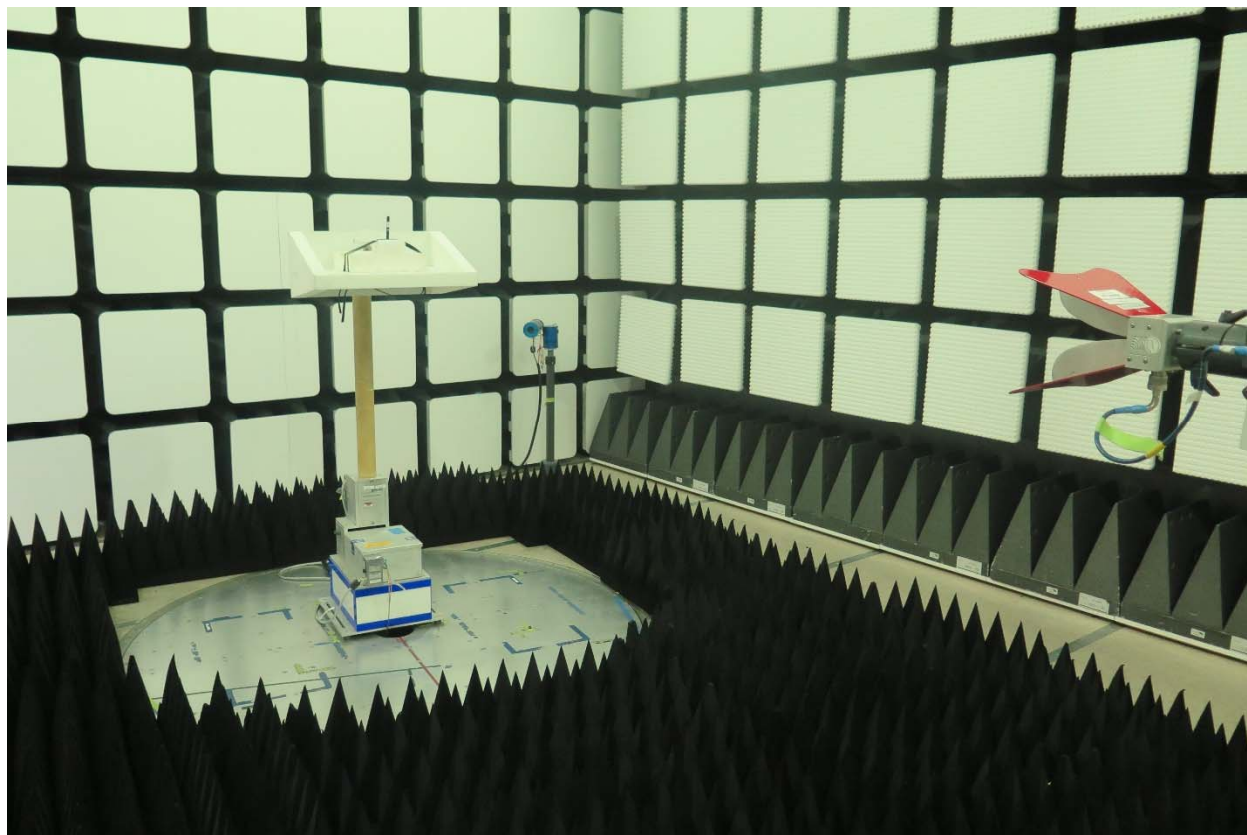
Figure 3 Radiated Spurious Emissions Test Setup (1-18GHz)
