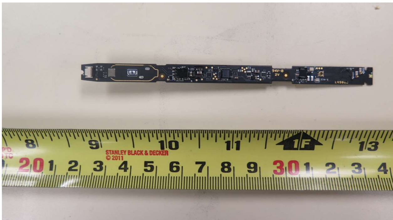
EUT PCBA- View 2
