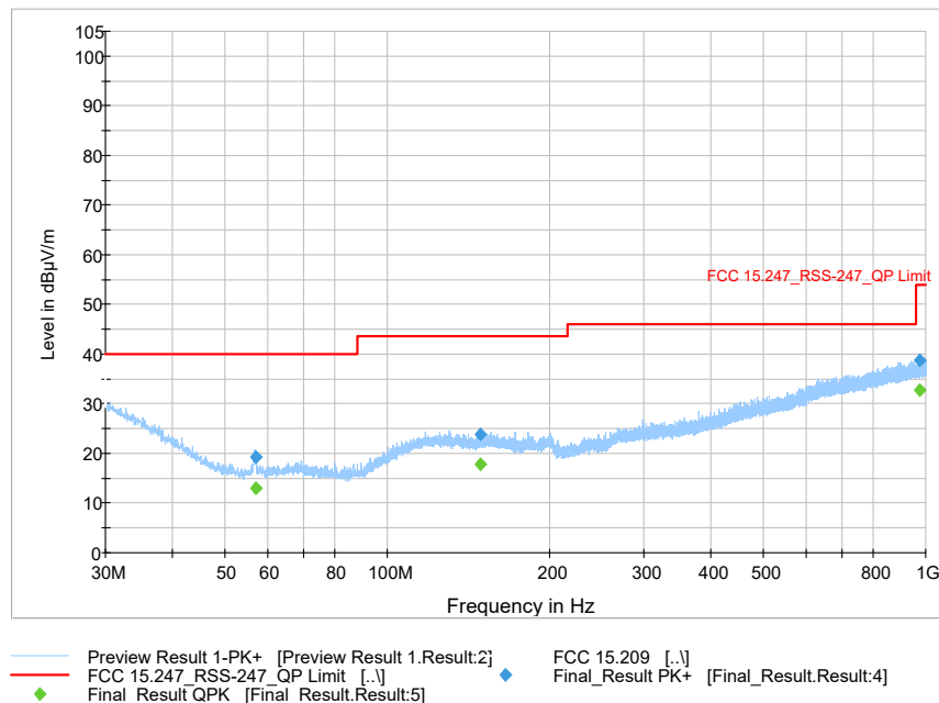
Figure 9-30 Radiated Spurious Emissions (Ch. 0) 2402 (30MHz - 1GHz)
