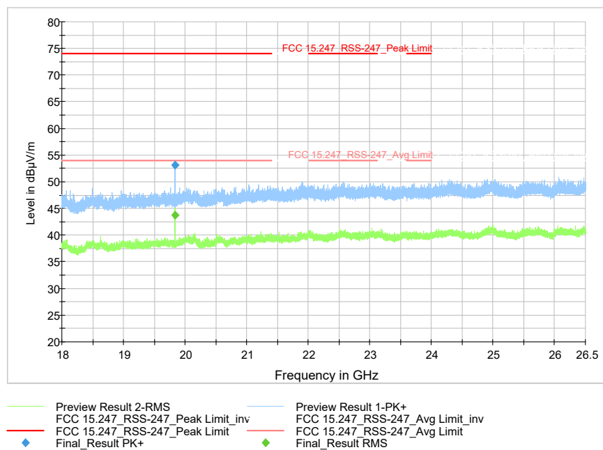
Figure 9-37 Radiated Spurious Emissions (Ch. 39) (18 – 26.5 GHz)
