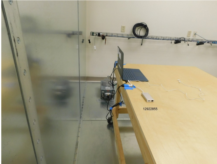
AC POWER LINE CONDUCTED EMISSIONS BACK
