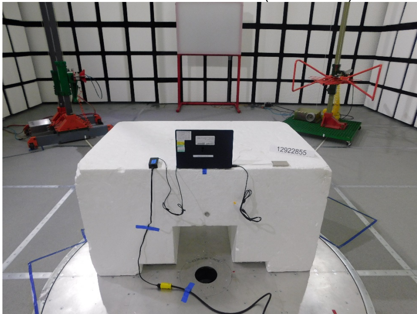
RADIATED SPURIOUS PHOTOS BACK (Below 1GHz)
