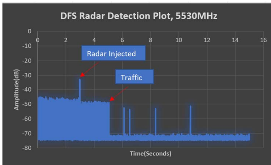
Figure 23. Channel Move Time 5530 MHz
