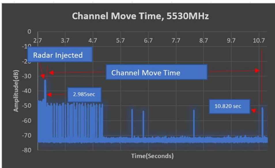
Figure 24. DFS Radar Detection Plot 5530 MHz
