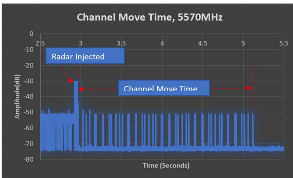
Figure 26. DFS Radar Detection Plot 5570 MHz, 160MHz Bandwidth
