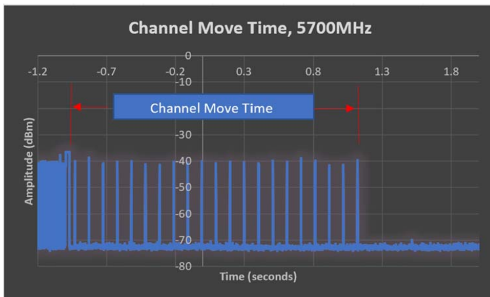
Figure 20. Channel Move Time 5700 MHz
