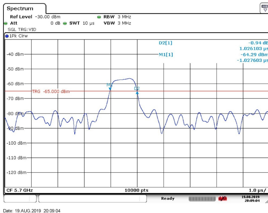
Figure 4. Radar Pulse width: Radar Type 0 (5700 MHz, 20MHz BW)
