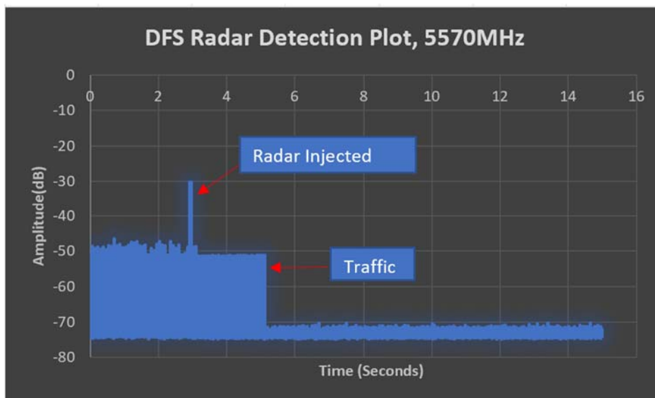
Figure 25. Channel Move Time 5570 MHz, 160 MHz Bandwidth
