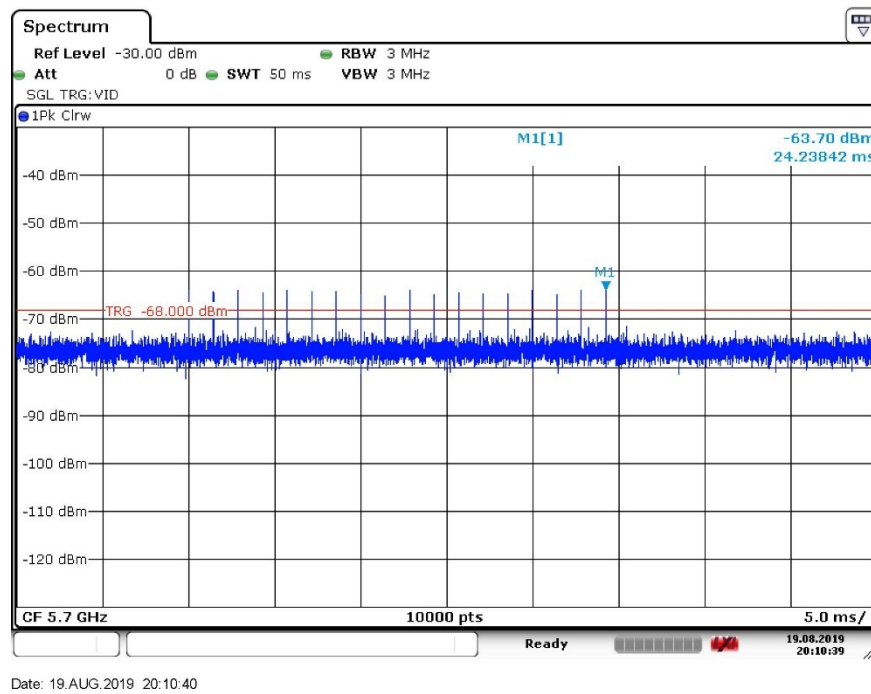
Figure 3. Radar Burst Level at -63dBm: Radar Type 0 (5700MHz, 20MHz BW)
