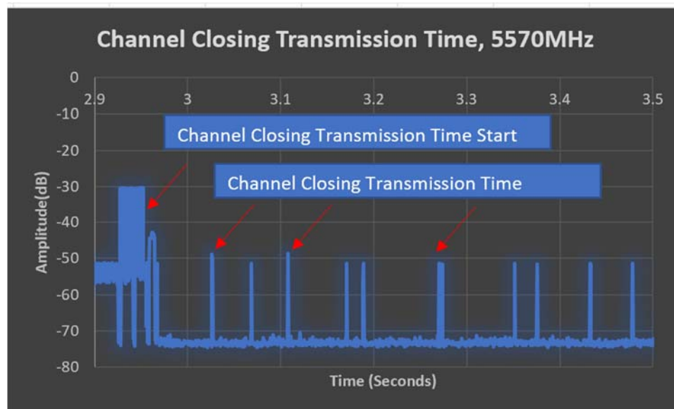
Figure 30. Channel Closing Transmission Time (5570 MHz), 160MHz Bandwidth
