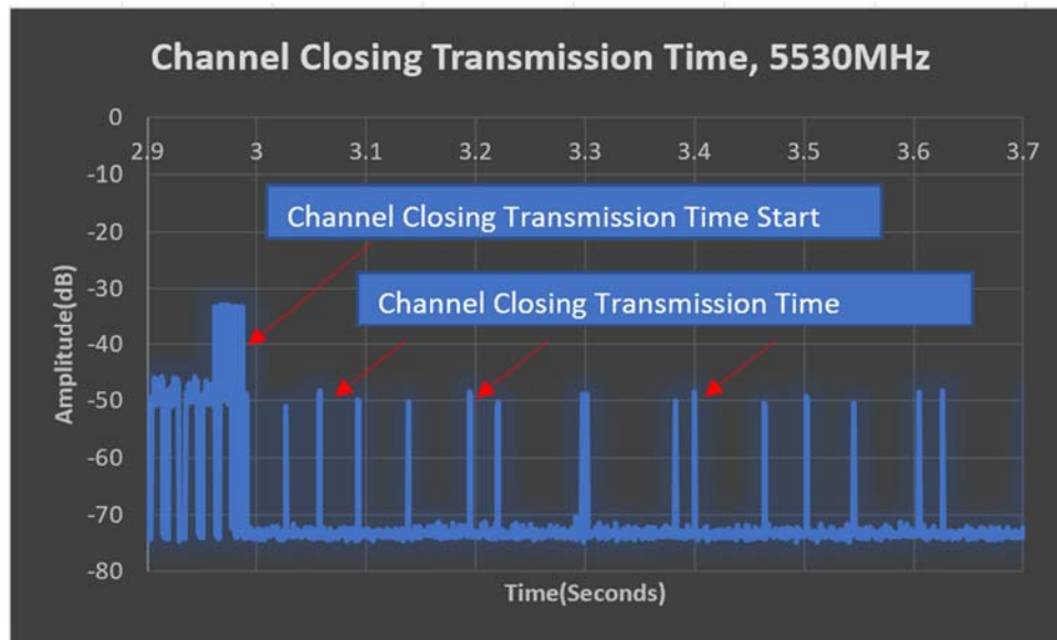
Figure 29. Channel Closing Transmission Time (5530 MHz), 80MHz Bandwidth
