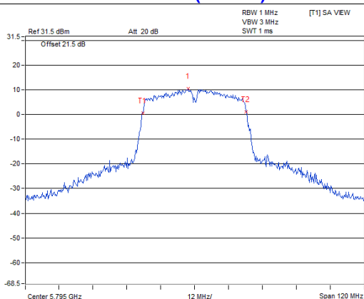
802.11ac (VHT40) / CH159
