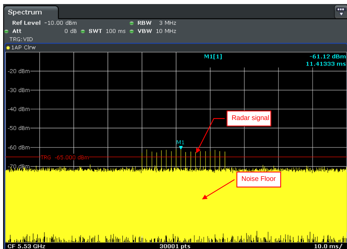
Radar Signal 0
